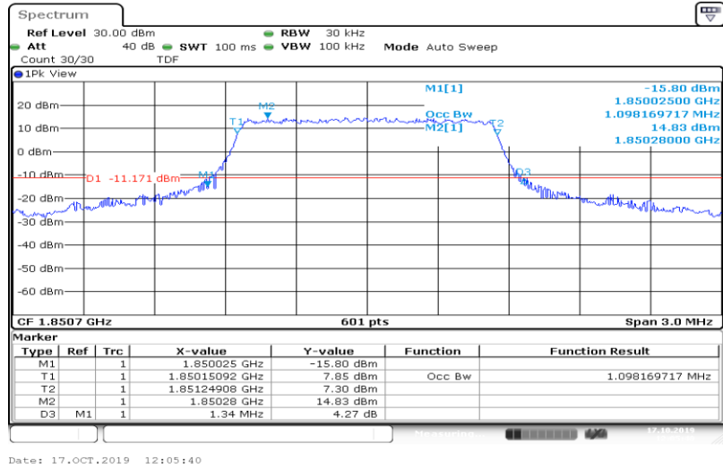
Band2-1.4MHz-QPSK-18900-6RB#0-1.098
