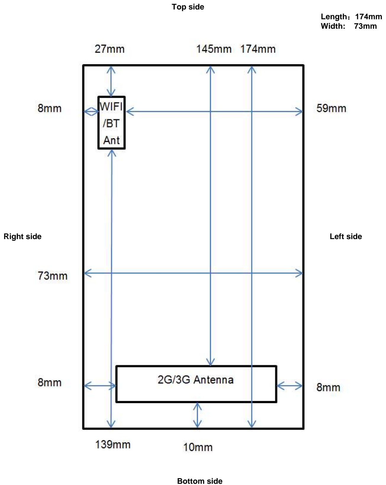
Figure1: The antenna position of the DUT
