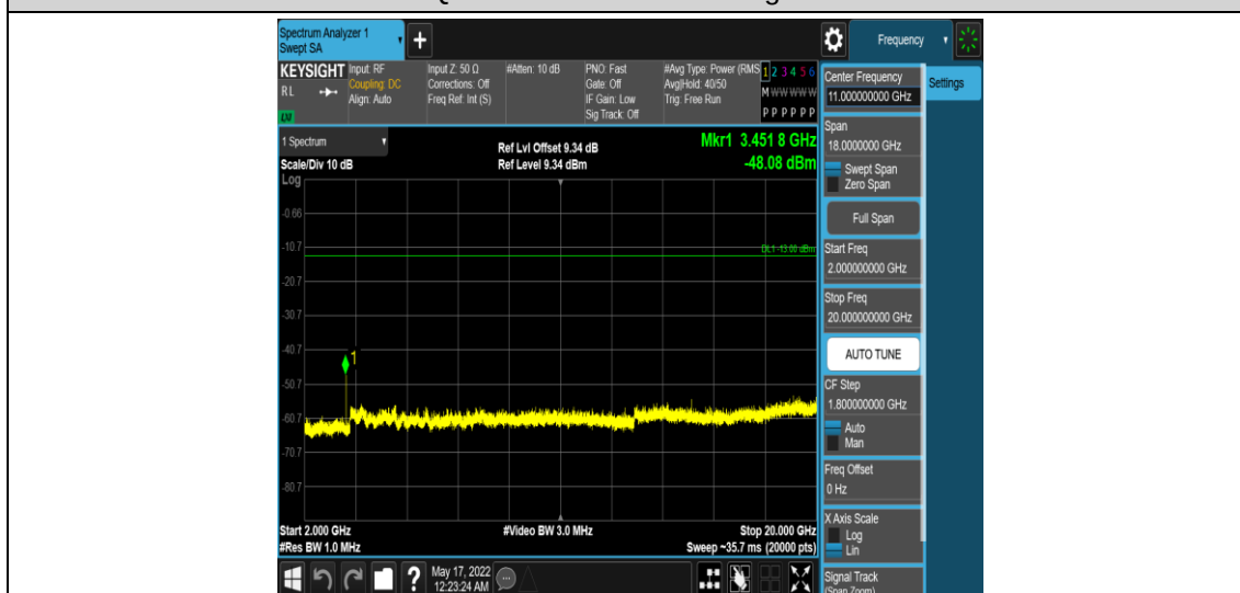
Band4-15MHz-QPSK-20175-1RB#0-Range5:2000~20000MHz
