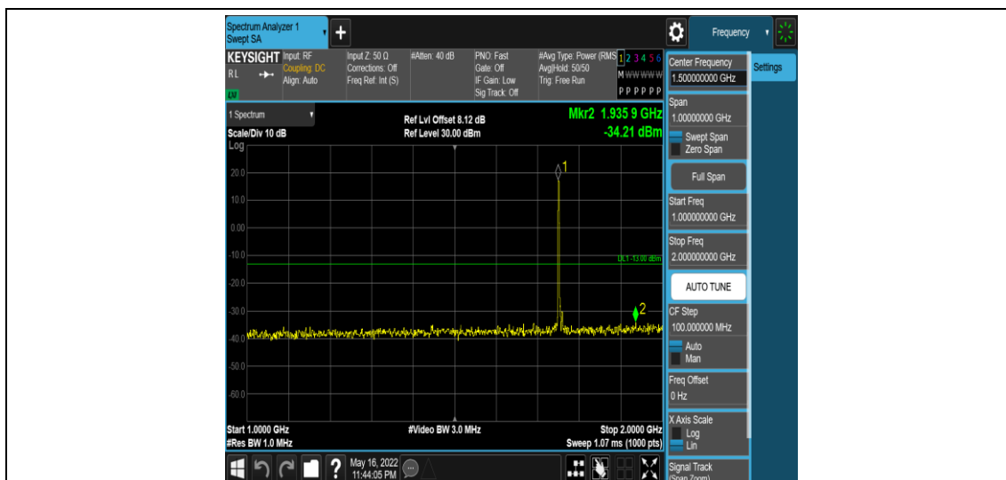
Band4-5MHz-16QAM-20375-1RB#0-Range4:1000~2000MHz
