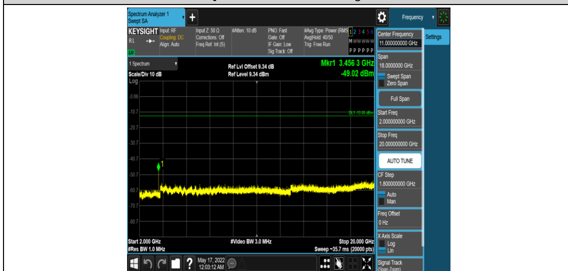
Band4-10MHz-16QAM-20175-1RB#0-Range5:2000~20000MHz
