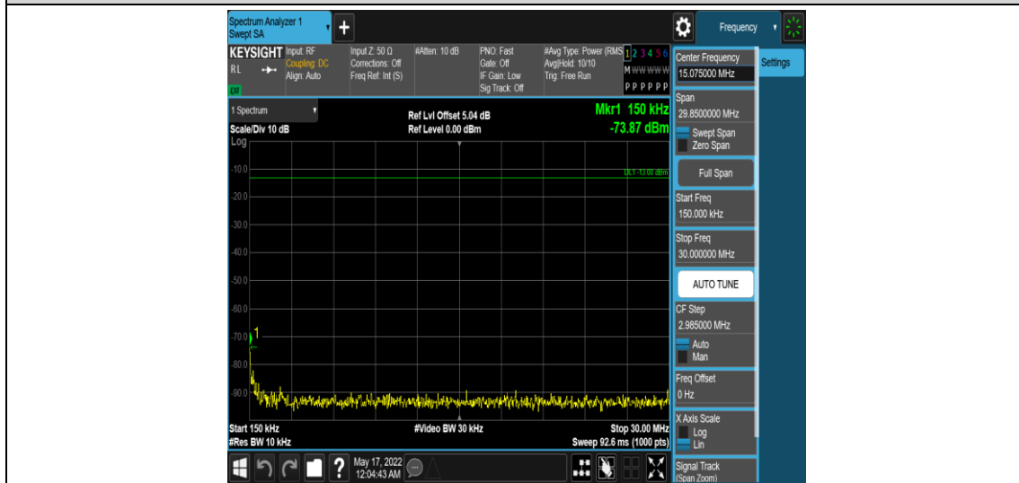
Band4-10MHz-16QAM-20350-1RB#0-Range2:0.15~30MHz
