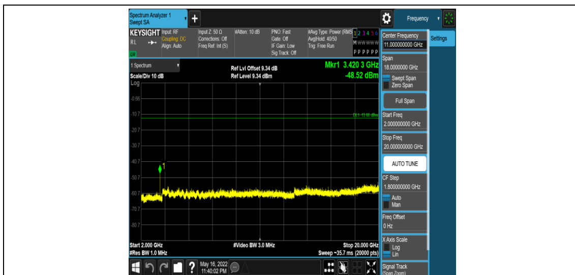
Band4-5MHz-16QAM-19975-1RB#0-Range5:2000~20000MHz
