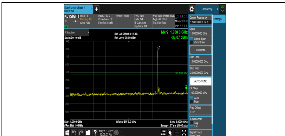
Band4-10MHz-16QAM-20350-1RB#0-Range4:1000~2000MHz
