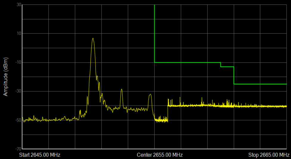
Band41(2535-2655) 16QAM BW=5MHz Channel=41215 RB Size=1 Position=#0
