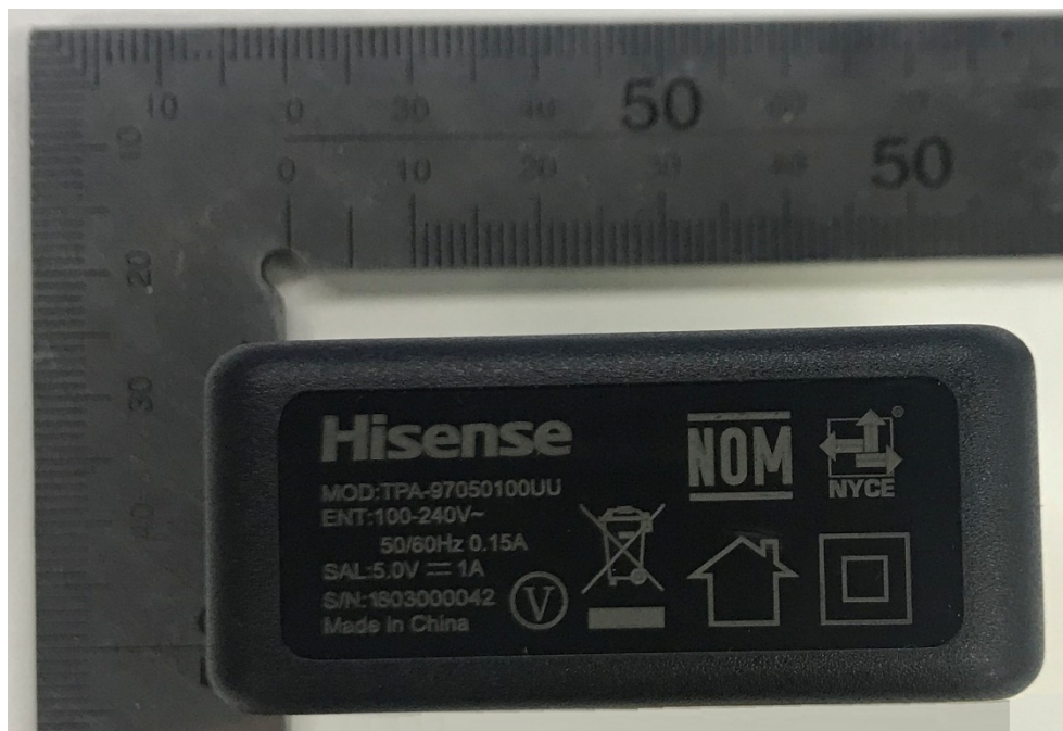
CHARGER View (TPA-97050100UU Made by Shenzhen Tianyin Electronics Co.,Ltd)
