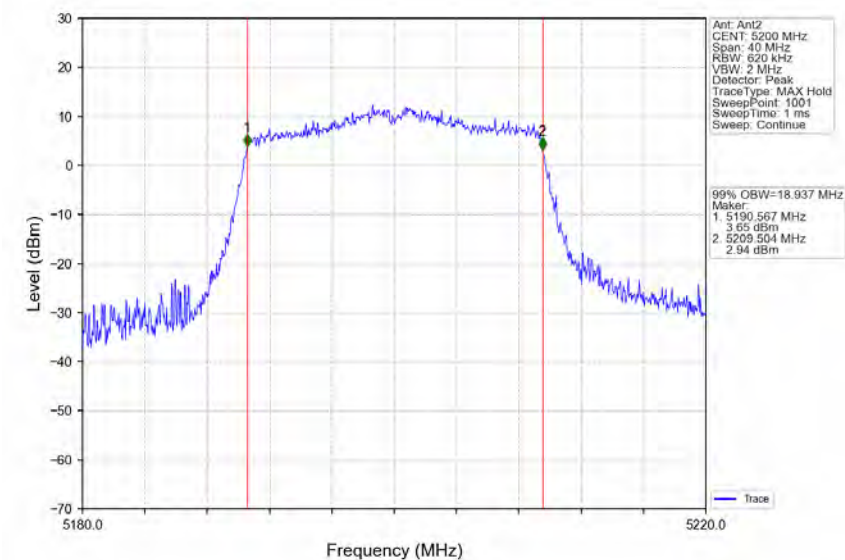
802.11ax(HEW20)_MCH_5200MHz_RU242_Left_Ant2_NTNV
