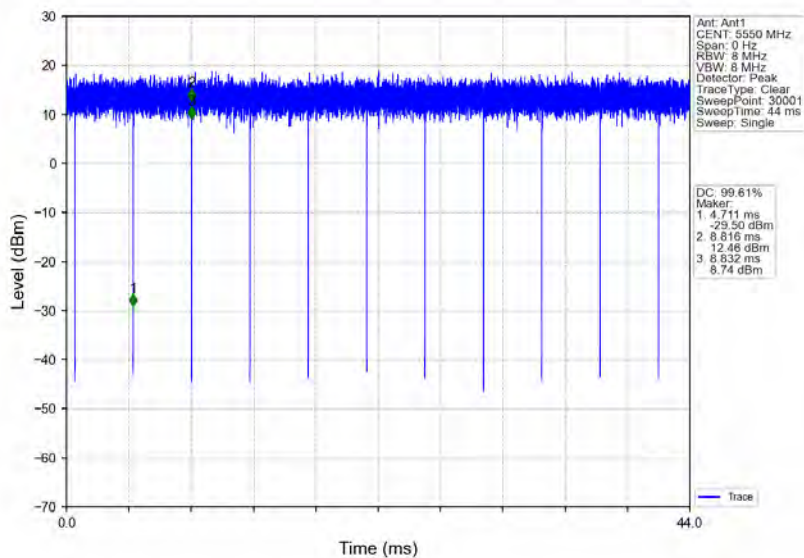
802.11ax(HEW40)_MCH_5550MHz_RU484_Left_Ant1_NTNV
