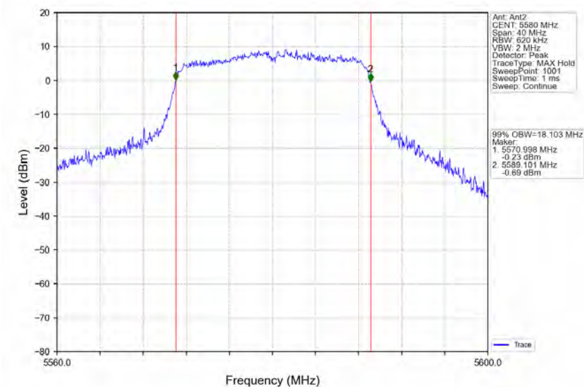
802.11n(HT20)_MCH_5580MHz_Ant2_NTNV
