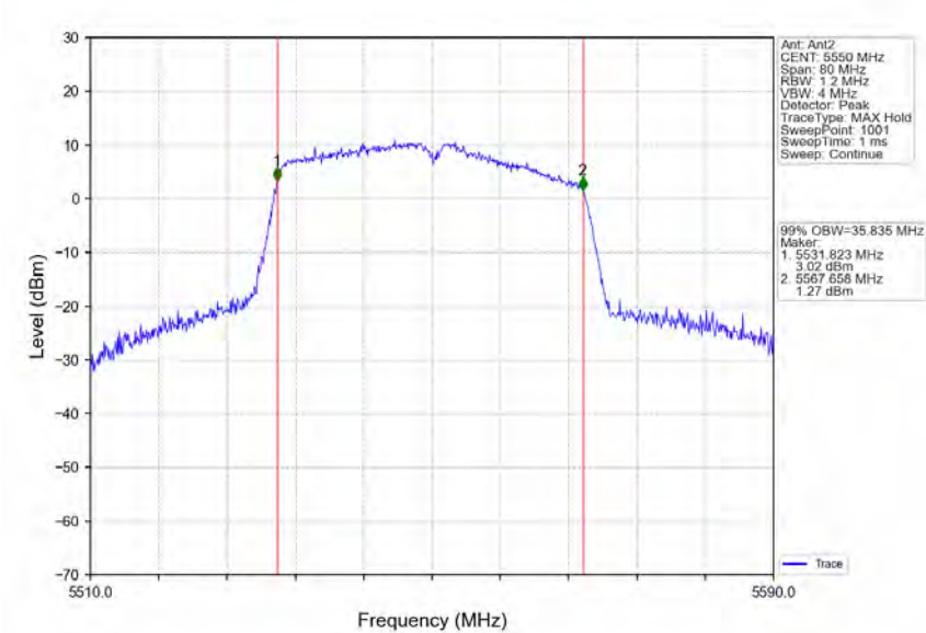
802.11n(HT40)_MCH_5550MHz_Ant2_NTNV
