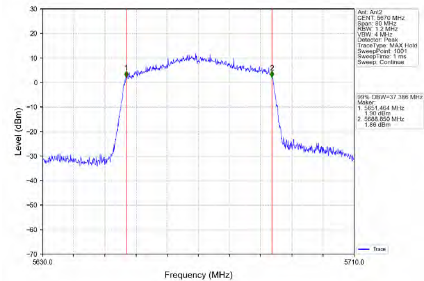
802.11ax(HEW40)_HCH_5670MHz_RU484_Left_Ant2_NTNV
