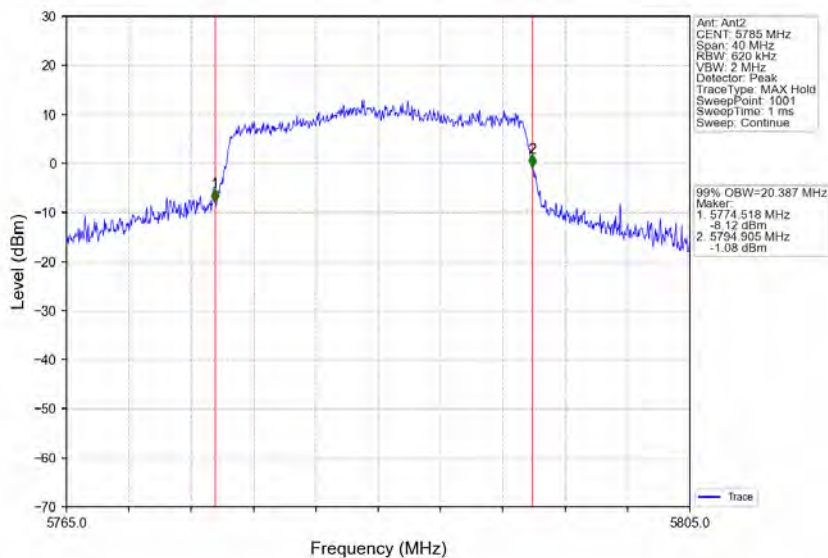
802.11ax(HEW20)_MCH_5785MHz_RU242_Left_Ant2_NTNV
