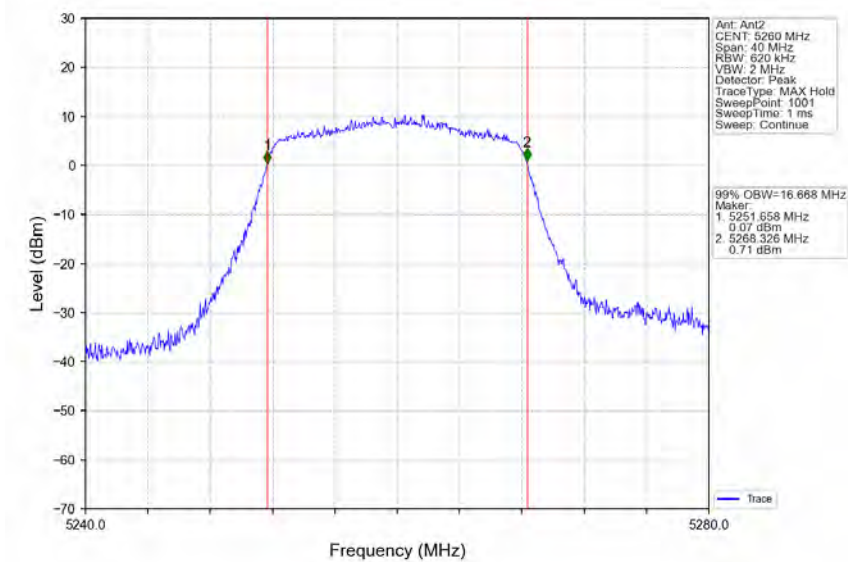
802.11a_LCH_5260MHz_Ant2_NTNV
