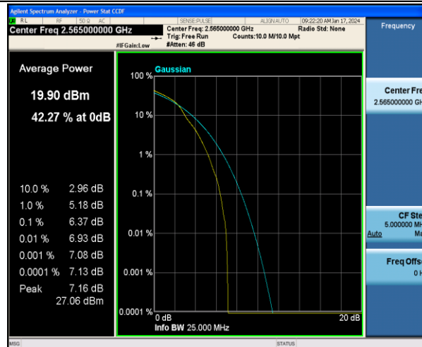
Band7-10MHz-16QAM-21400-1RB#0-PASS
