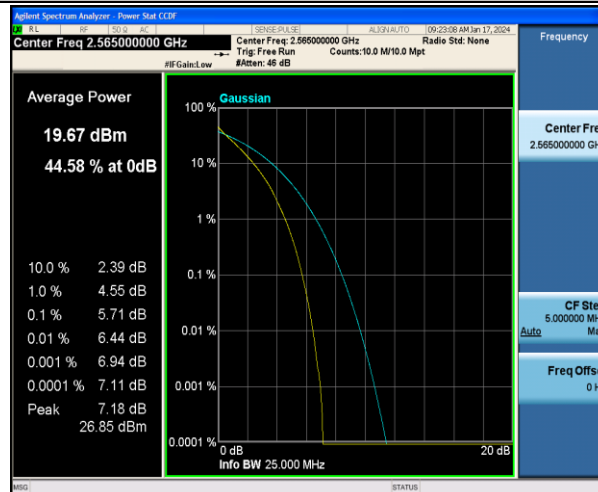
Band7-10MHz-QPSK-21400-50RB#0-PASS
