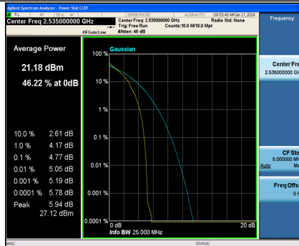
Band7-20MHz-QPSK-21100-1RB#0-PASS
