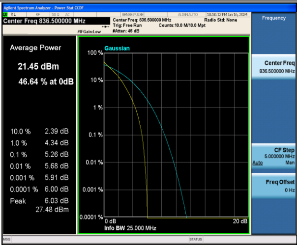
Band5-5MHz-QPSK-20525-25RB#0-PASS
