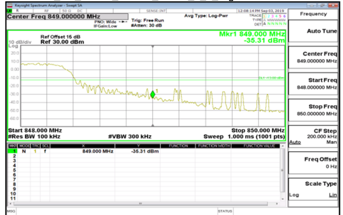
Cat M1_Band5_10MHz_QPSK_6_0_HighCH20600-844
