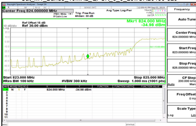
Cat M1_Band5_10MHz_QPSK_6_0_LowCH20450-829
