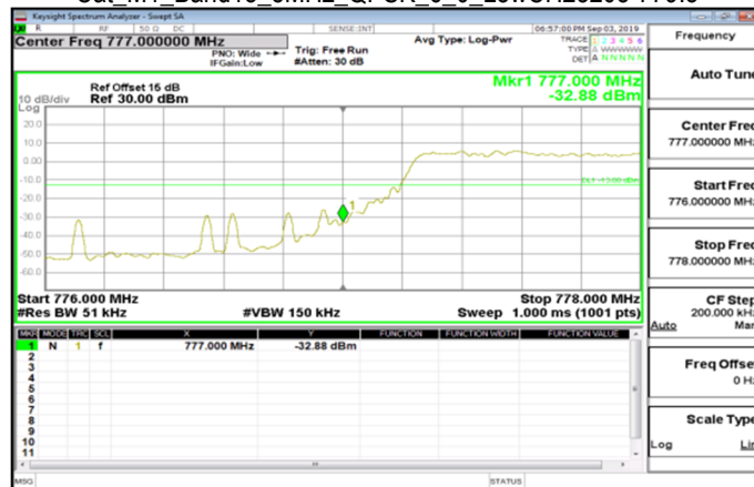
Cat_M1_Band13_5MHz_QPSK_6_0_LowCH23205-779.5
