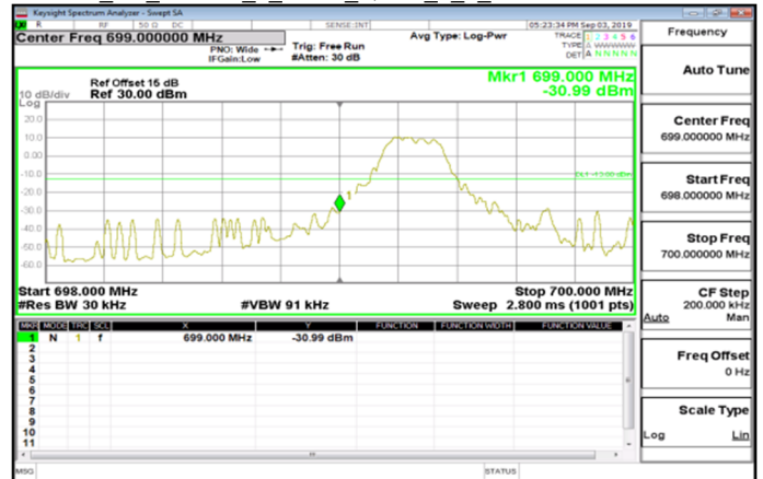
Cat M1_Band12_1_4MHz_QPSK_1_0_LowCH23017-699.7
