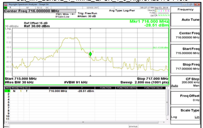
Cat M1_Band12_1_4MHz_QPSK_1_5_HighCH23173-715.3
