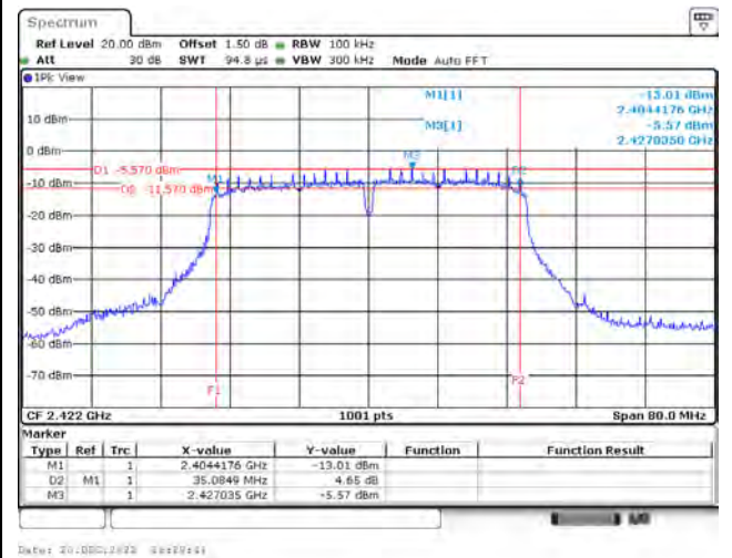
802.11n (40 MHz) / 2422 MHz
