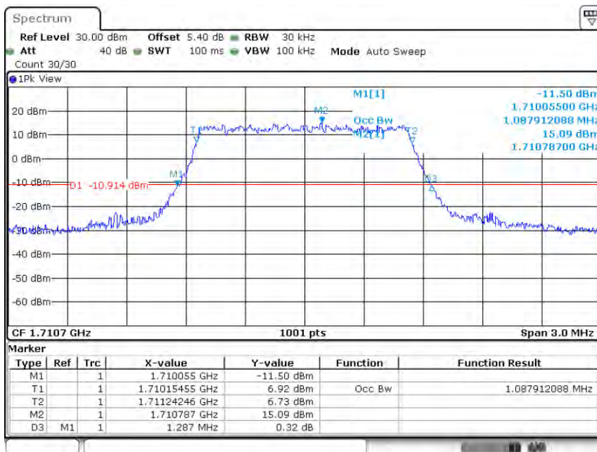
Band66-1.4MHz-QPSK-131979-6RB#0-1.088
