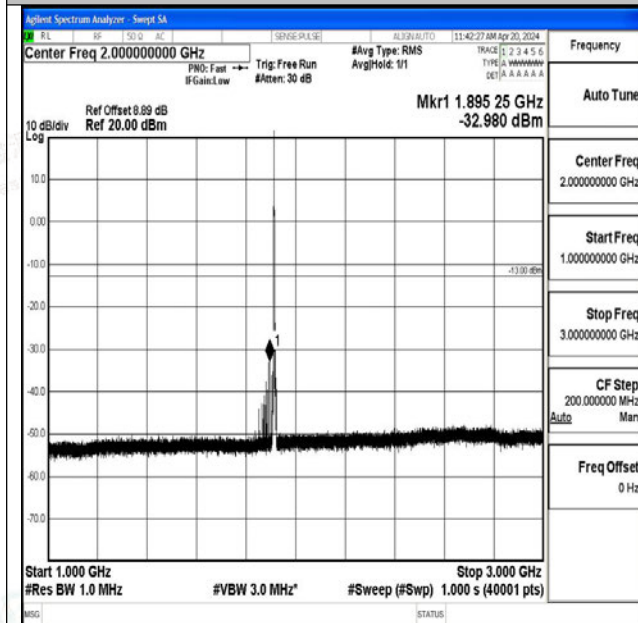
Band25_3MHz_16QAM_26675_1RB#0_1000~3000_100
