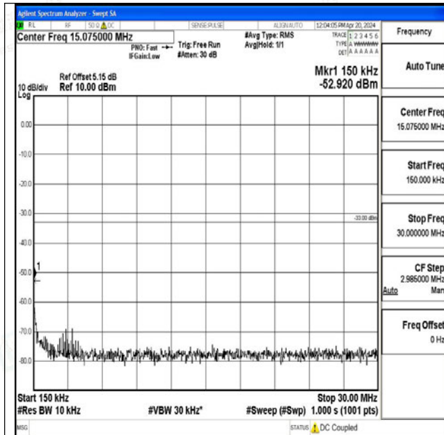
Band25_5MHz_16QAM_26365_1RB#0_0.15~30_0.15~3
