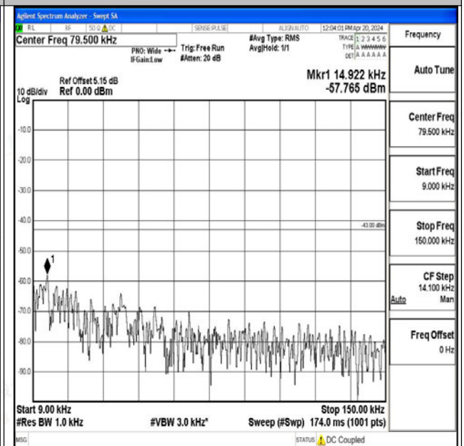
Band25_5MHz_16QAM_26365_1RB#0_0.009~0.15_0.0 09~0.15
