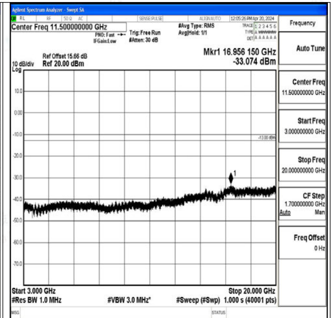
Band25_5MHz_16QAM_26665_1RB#0_3000~20000_30 00~20000
