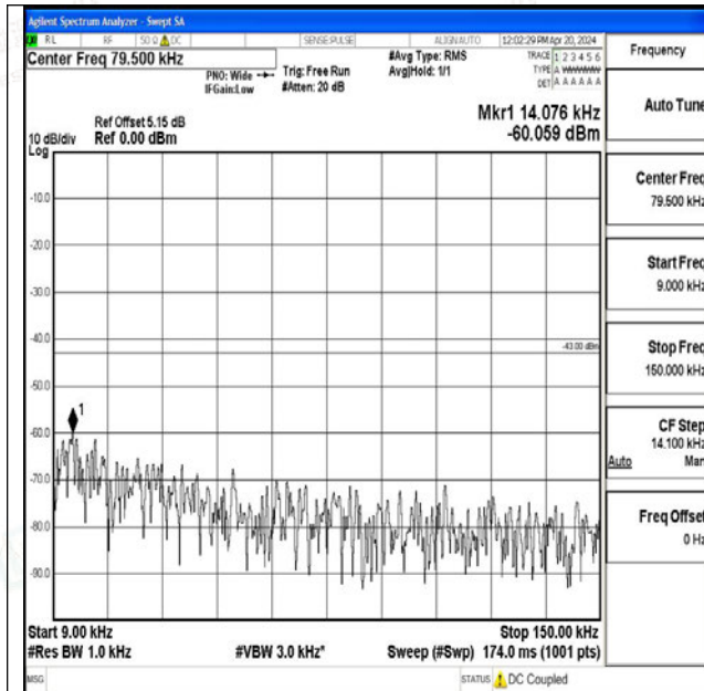
Band25_5MHz_QPSK_26065_1RB#0_0.009~0.15_0.009 ~0.15
