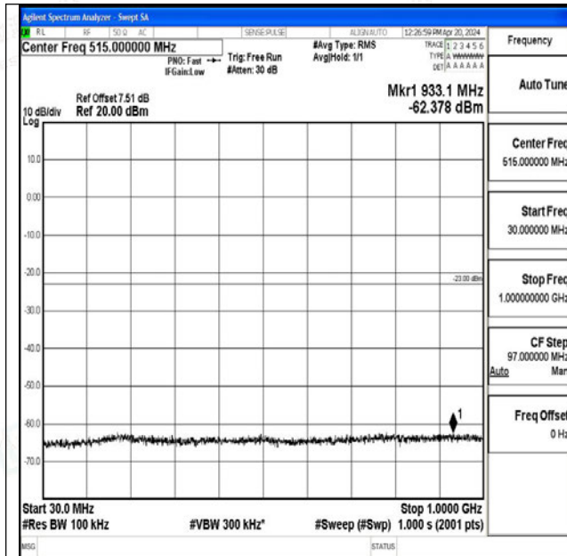
Band25_10MHz_QPSK_26640_1RB#0_30~1000_30~1000
