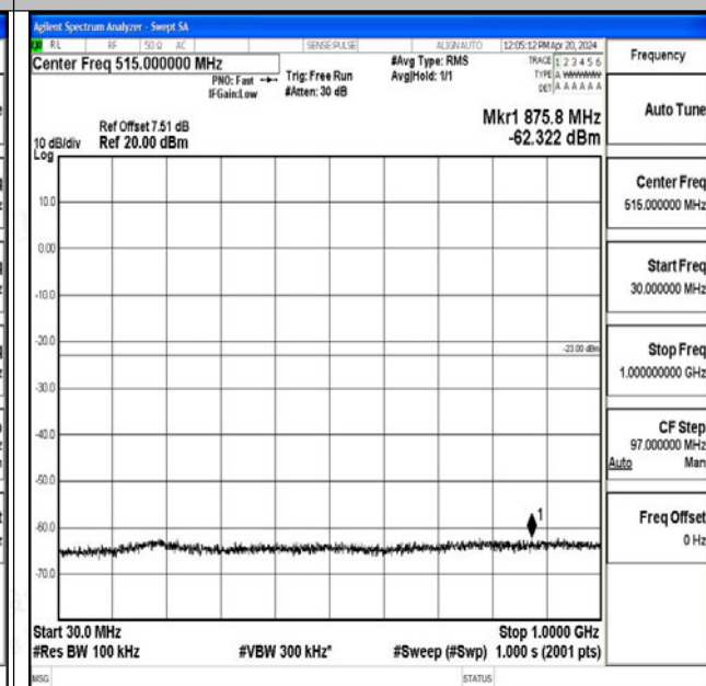
Band25_5MHz_16QAM_26665_1RB#0_30~1000_30~1000
