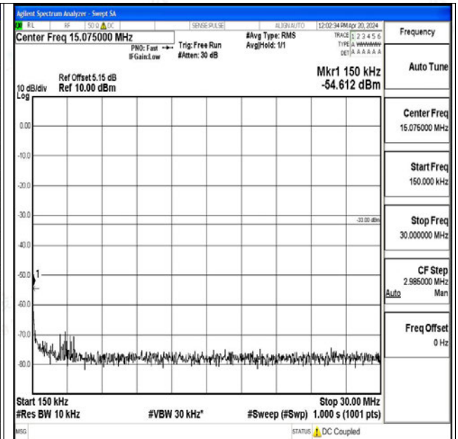
Band25_5MHz_QPSK_26065_1RB#0_0.15~30_0.15~30
