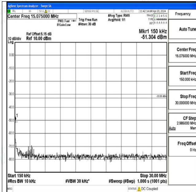
Band25_3MHz_16QAM_26675_1RB#0_0.15~30_0.15~3
