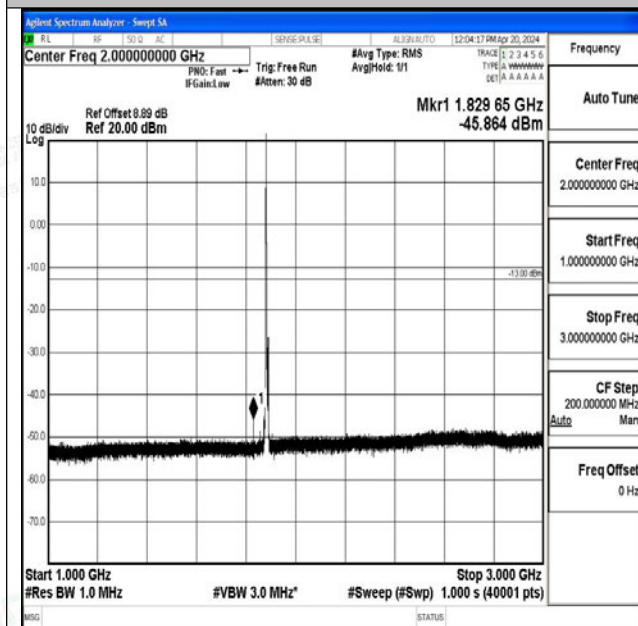
Band25_5MHz_16QAM_26365_1RB#0_1000~3000_100
