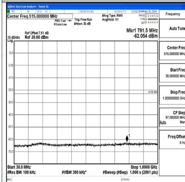
Band25_5MHz_QPSK_26065_1RB#0_30~1000_30~1000 0
