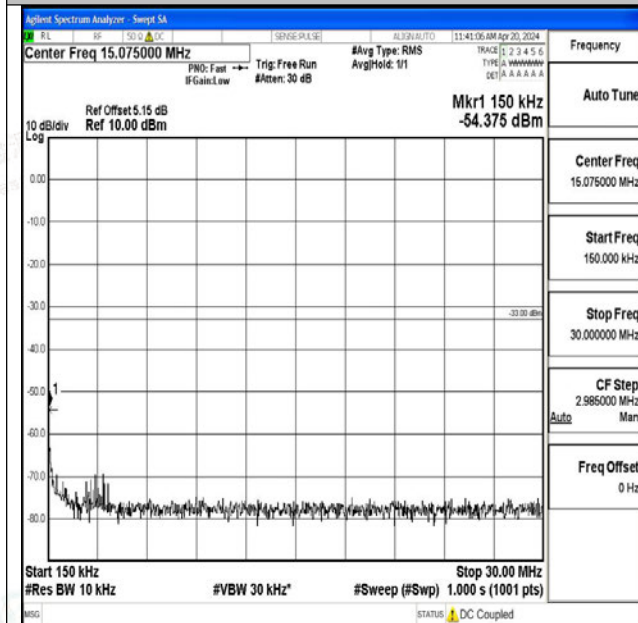
Band25_3MHz_16QAM_26365_1RB#0_0.15~30_0.15~3 0
