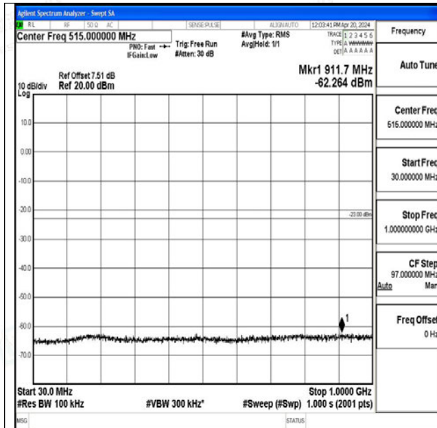
Band25_5MHz_QPSK_26365_1RB#0_30~1000_30~1000 0
