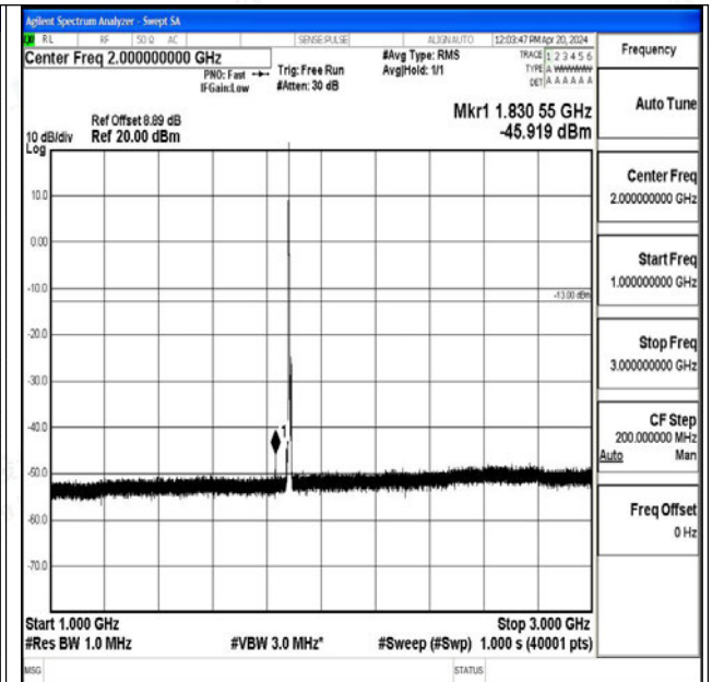
Band25_5MHz_QPSK_26365_1RB#0_1000~3000_1000 ~3000
