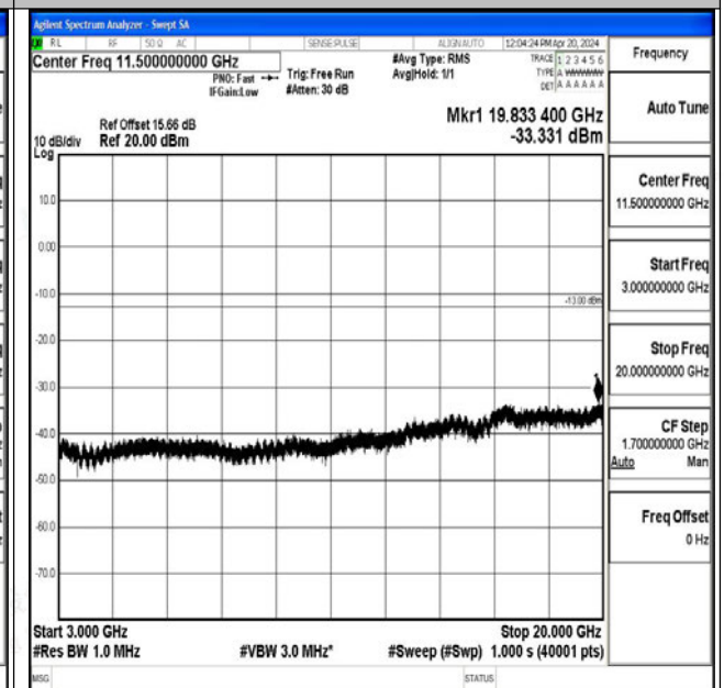
Band25_5MHz_16QAM_26365_1RB#0_3000~20000_30
