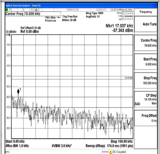
Band25_10MHz_16QAM_26090_1RB#0_0.009~0.15_0.009~0.15
