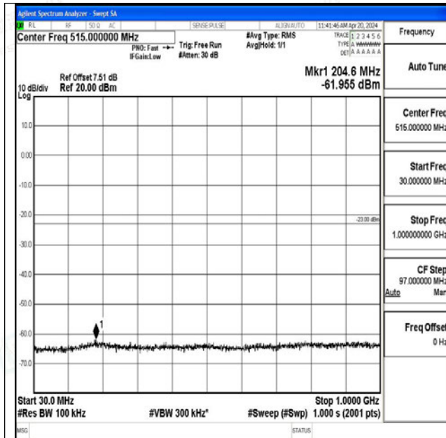
Band25_3MHz_QPSK_26675_1RB#0_30~1000_30~100 0
