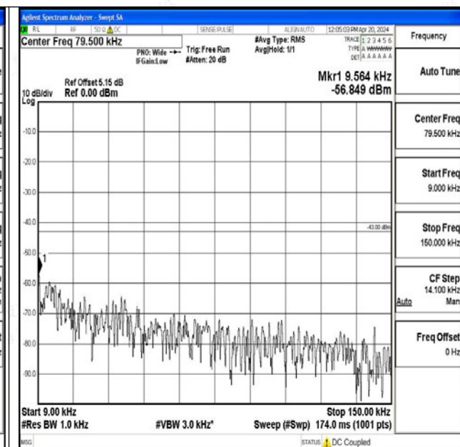
Band25_5MHz_16QAM_26665_1RB#0_0.009~0.15_0.009~0.15
