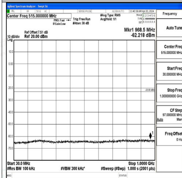
Band25_3MHz_QPSK_26365_1RB#0_30~1000_30~1000 0
