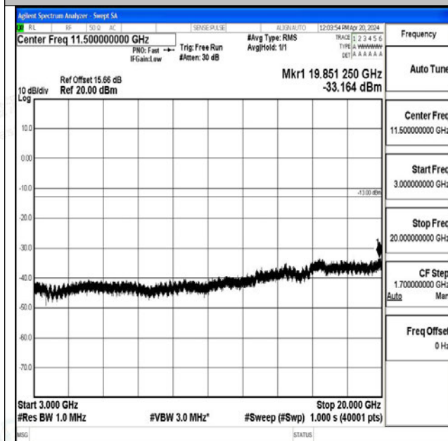
Band25_5MHz_QPSK_26365_1RB#0_3000~20000_300 0~20000
