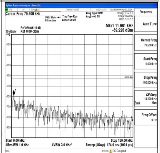
Band25_3MHz_16QAM_26675_1RB#0_0.009~0.15_0.0 09~0.15
