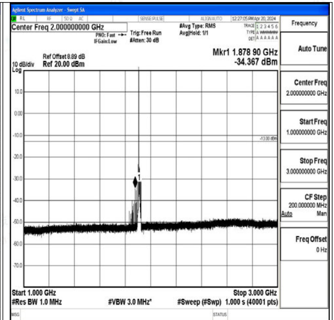
Band25_10MHz_QPSK_26640_1RB#0_1000~3000_1000~3000
