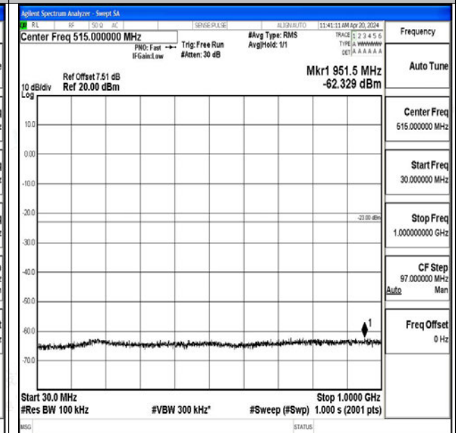
Band25_3MHz_16QAM_26365_1RB#0_30~1000_30~10 00
