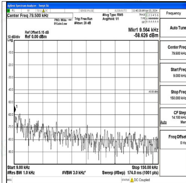
Band25_3MHz_QPSK_26365_1RB#0_0.009~0.15_0.009 ~0.15
