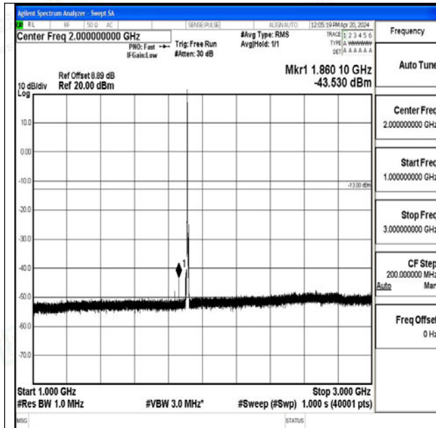
Band25_5MHz_16QAM_26665_1RB#0_1000~3000_100 0~3000
