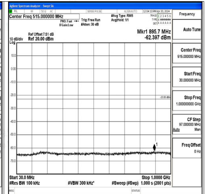
Band25_5MHz_16QAM_26365_1RB#0_30~1000_30~10
