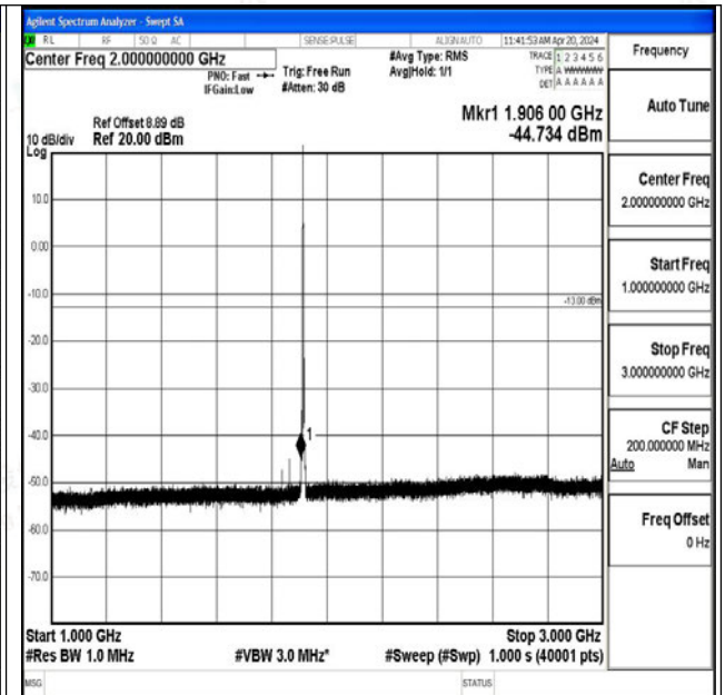
Band25_3MHz_QPSK_26675_1RB#0_1000~3000_1000 ~3000
