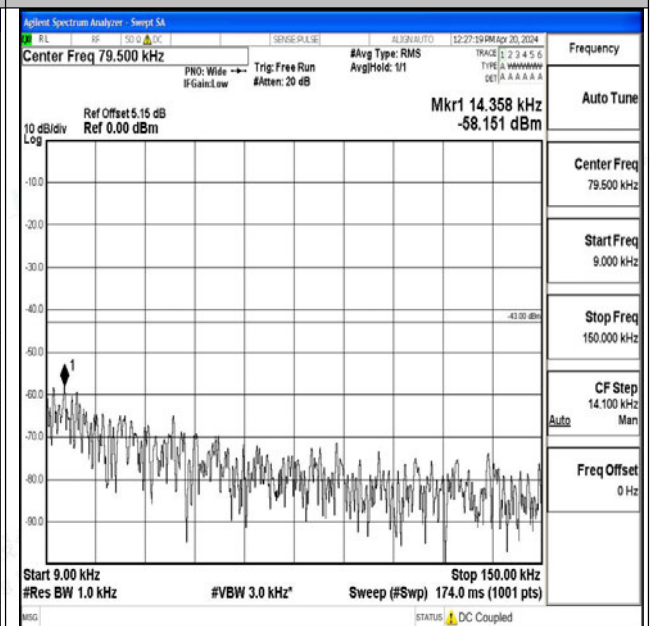
Band25_10MHz_16QAM_26640_1RB#0_0.009~0.15_0.009~0.15
