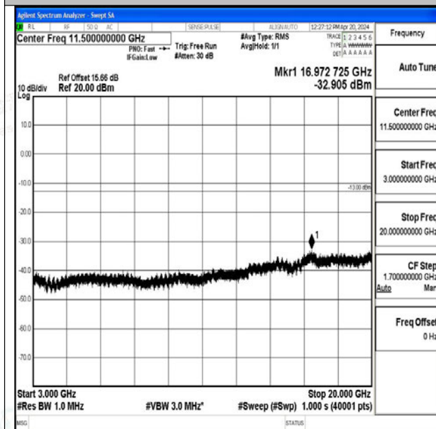
Band25_10MHz_QPSK_26640_1RB#0_3000~20000_3000~20000
