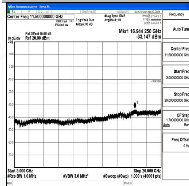
Band25_3MHz_QPSK_26675_1RB#0_3000~20000_300 0~20000
