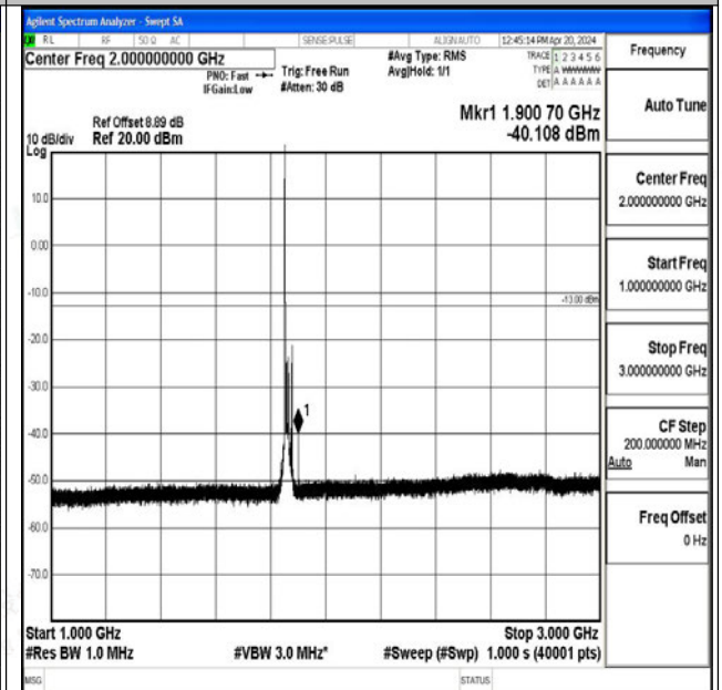
Band25_15MHz_QPSK_26115_1RB#0_1000~3000_100 0~3000
