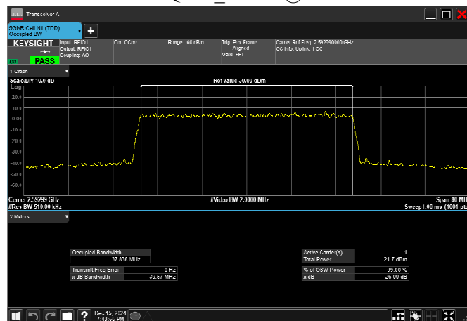
n41_50MHz_30kHz_2592.99MHz_DFT-s-OFDM \pi/2 BPSK RB128@0
