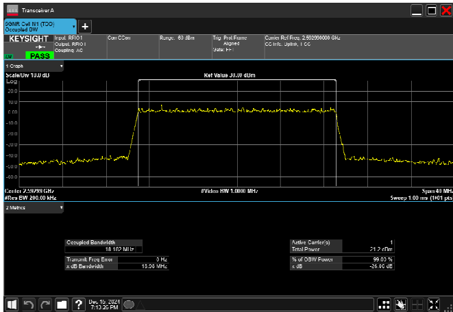
n41_20MHz_30kHz_2592.99MHz_CP-OFDM 256 QAM_RB51@0
