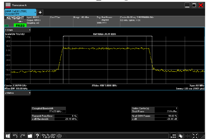
n41_30MHz_30kHz_2592.99MHz_DFT-s-OFDM 16 QAM_RB75@0
