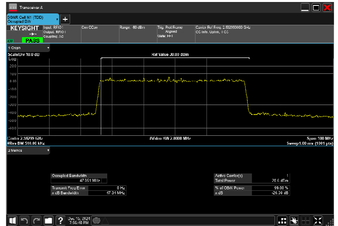
n41_50MHz_30kHz_2592.99MHz_CP-OFDM 16 QAM_RB133@0
