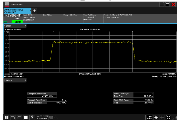
n41_50MHz_30kHz_2592.99MHz_CP-OFDM 256 QAM_RB133@0
