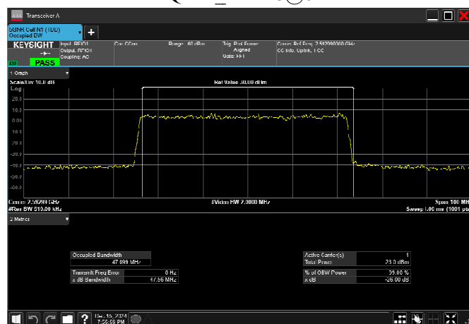
n41_50MHz_30kHz_2592.99MHz_DFT-s-OFDM 16 QAM RB128@0
