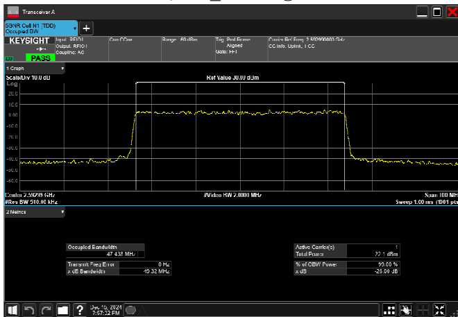
n41_50MHz_30kHz_2592.99MHz_CP-OFDM 64 QAM_RB133@0
