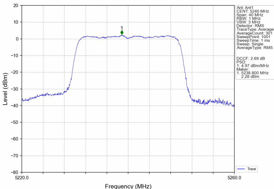
802.11ax(HEW20)_HCH_5240MHz_RU242_Left_MIMO_NTNV
