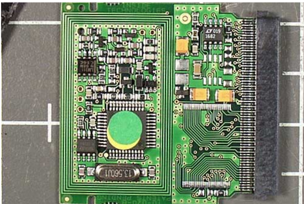
PCB 1 Top
