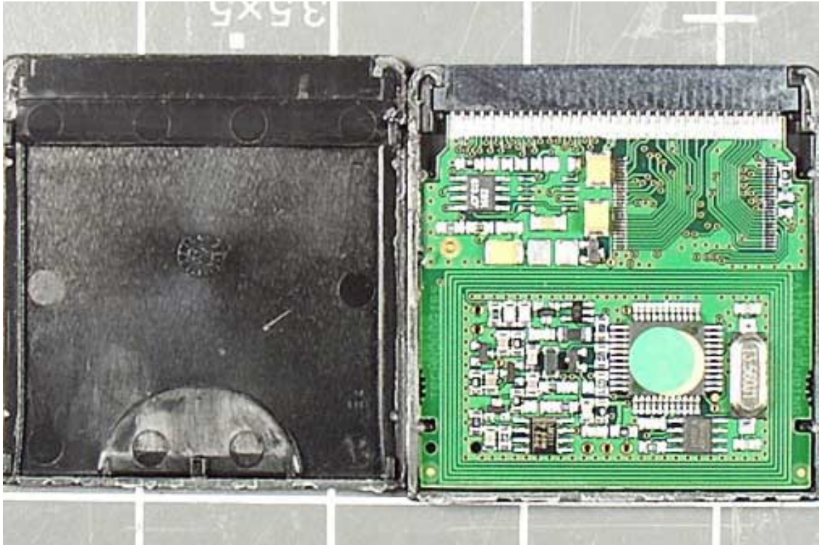
Cover Removed
