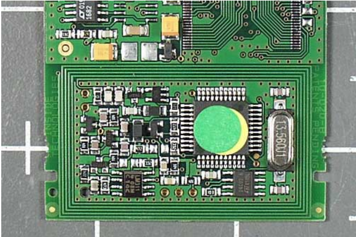
PCB 1 Closeup 2
