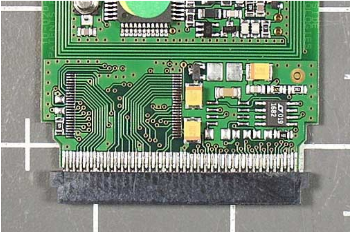
PCB 1 Closeup 1
