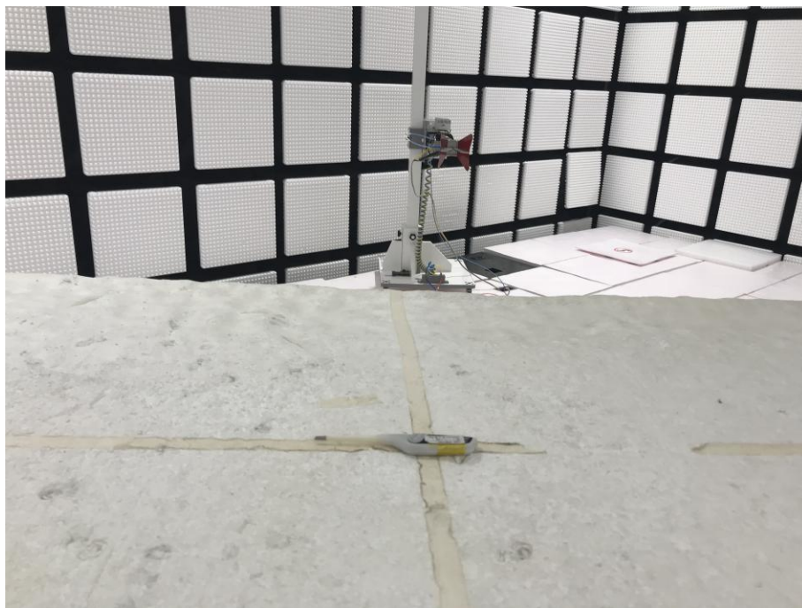
Radiated spurious emission Test Setup-2(Above 1GHz)Close up photos
