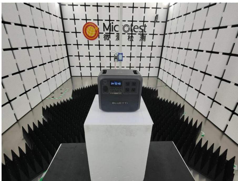
Radiation spurious (above 1GHz)
