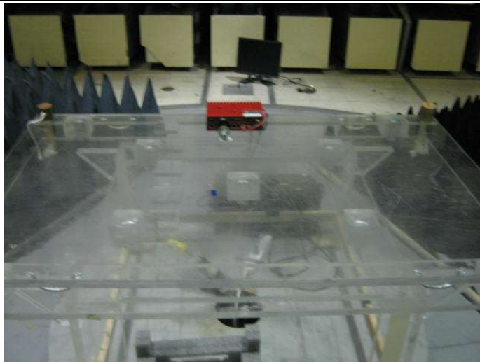
Radiated Emissions up to 1 GHz, Front
