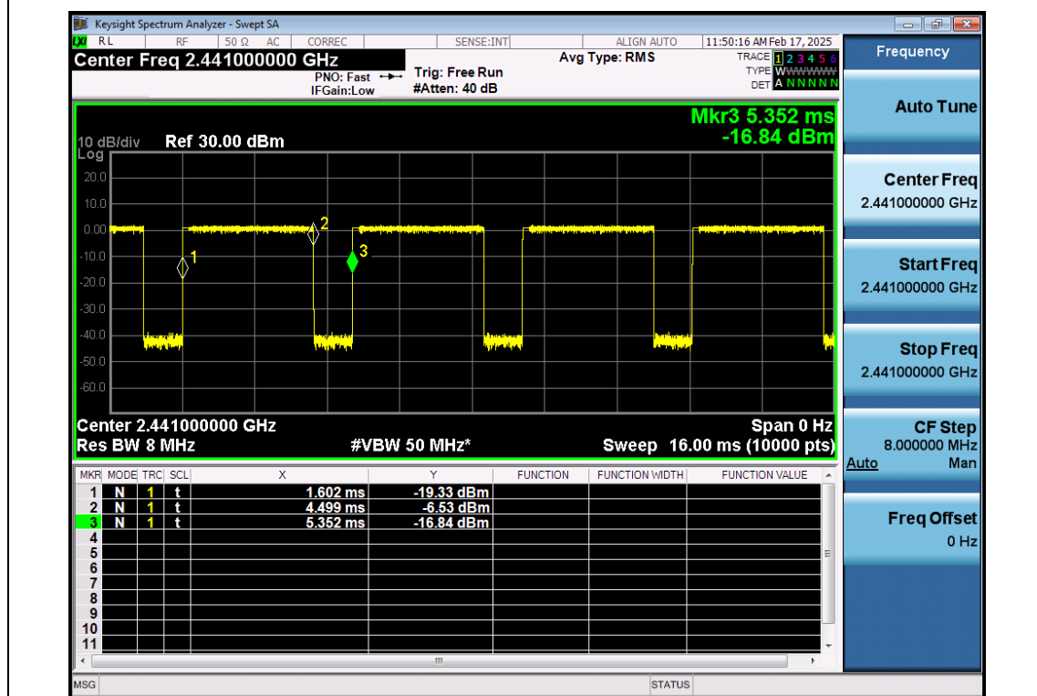
EDR-8DPSK-Ant1-2441
