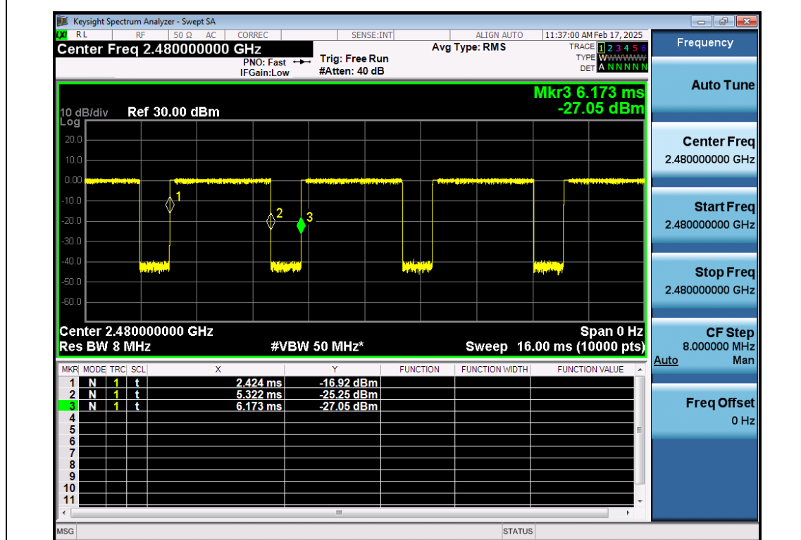
EDR-π /4-DQPSK-Ant1-2480
