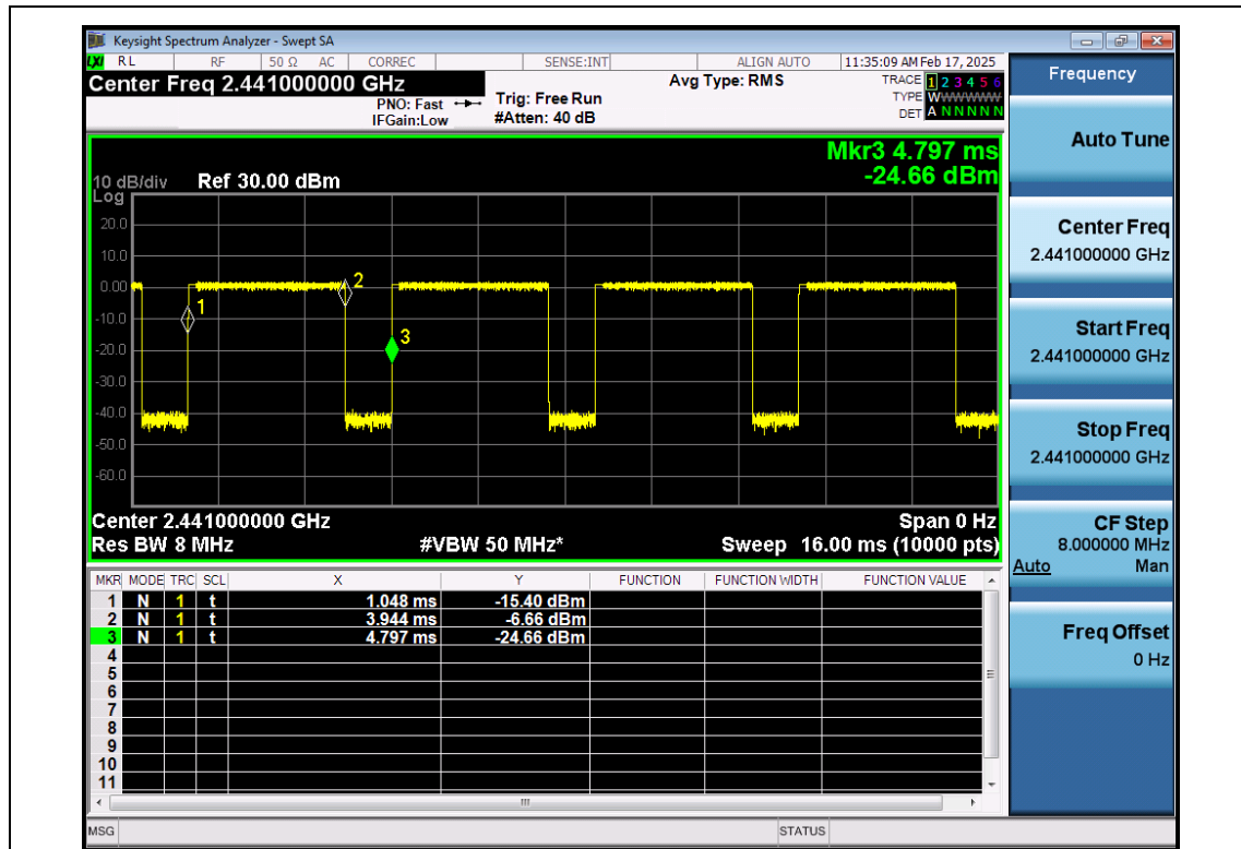
EDR-π /4-DQPSK-Ant1-2441
