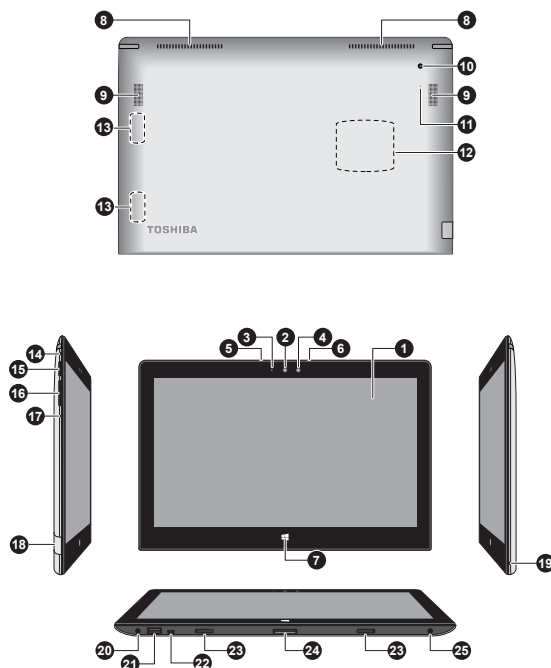
Figure 3-1 The computer in tablet mode
