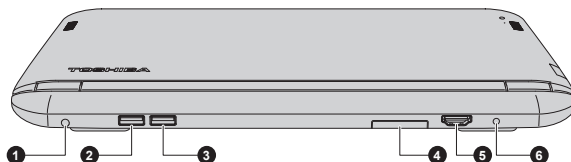
Figure 3-3 The back of the computer
