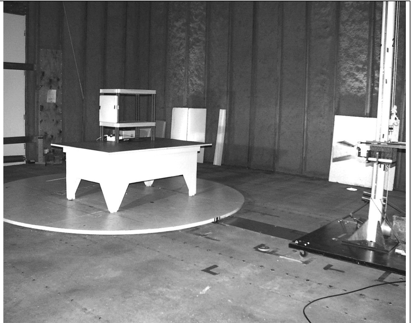
RE Testing with Horn on 3 meter range
