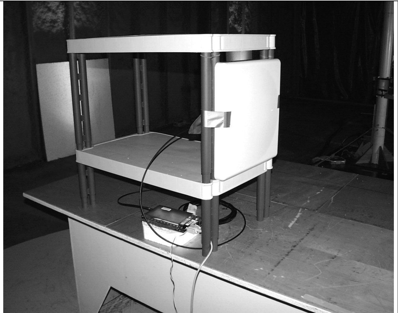
H&S Antenna Mounting Front View
