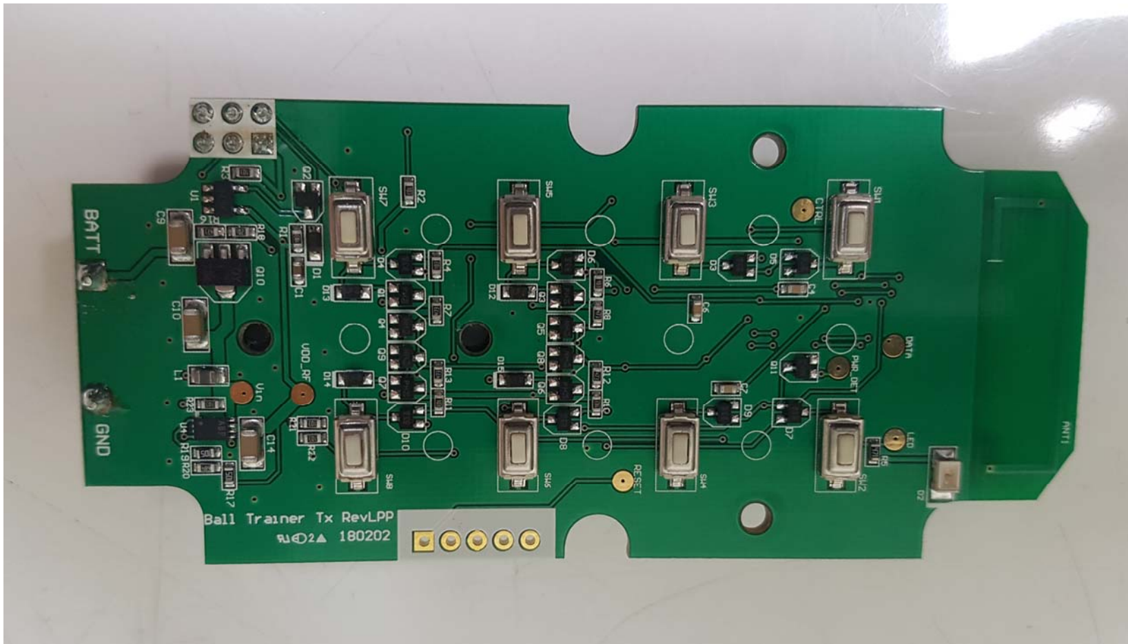
[Main board Front]
