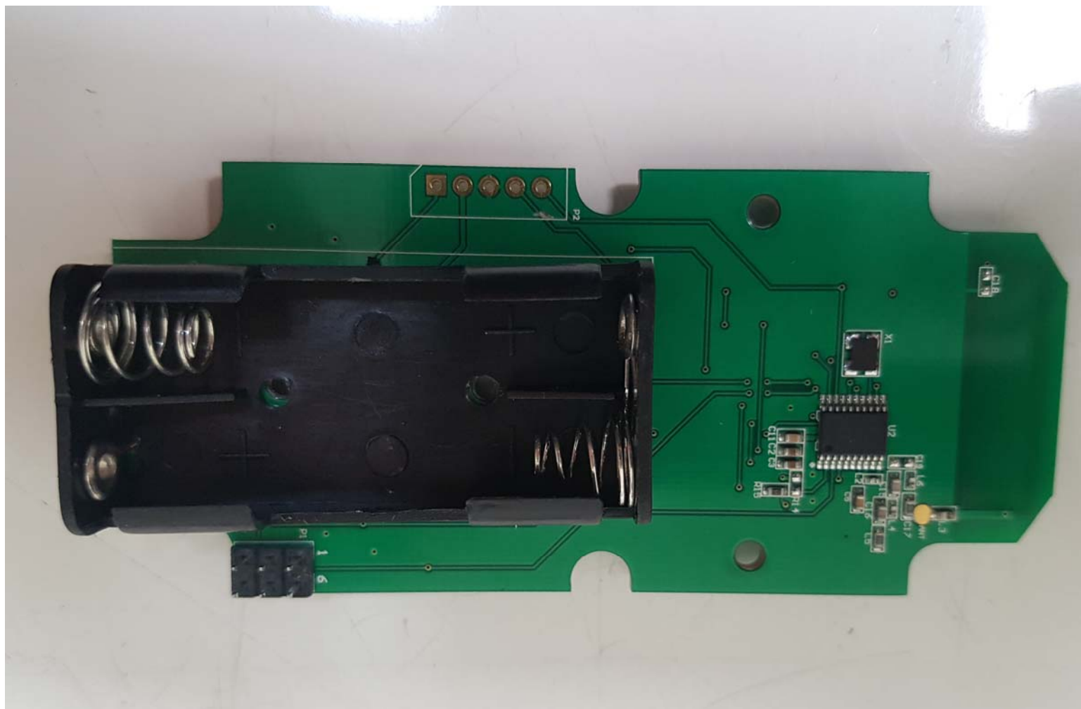
[Main board Rear]
