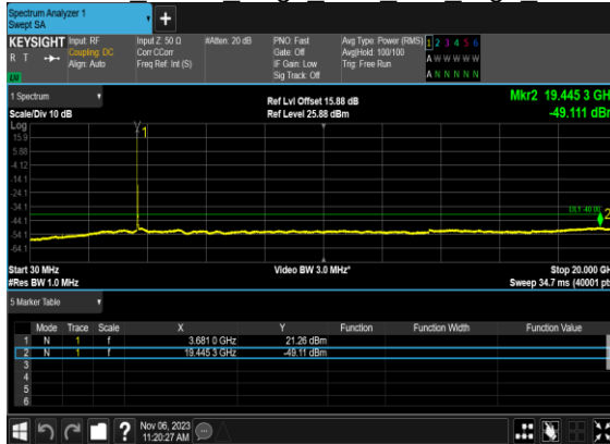
N48(20M)_DFT-s- OFDM BPSK Edge 1RB Left High CH
