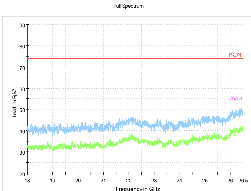
Pic6. Radiated emission (18GHz –26.5GHz)
