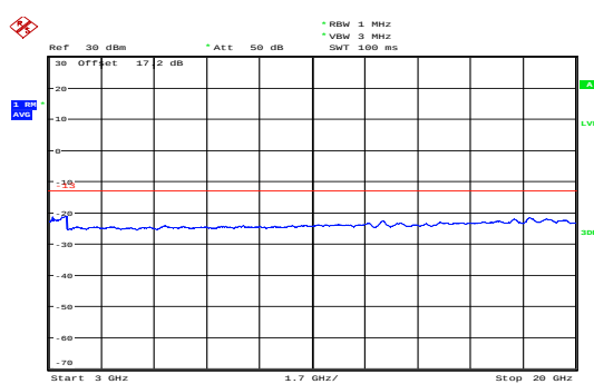
LTE Band 4 1.4MHz CH-Middle 3GHz~20GHz
