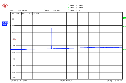
LTE Band 4 1.4MHz CH-Middle 1GHz~3GHz
