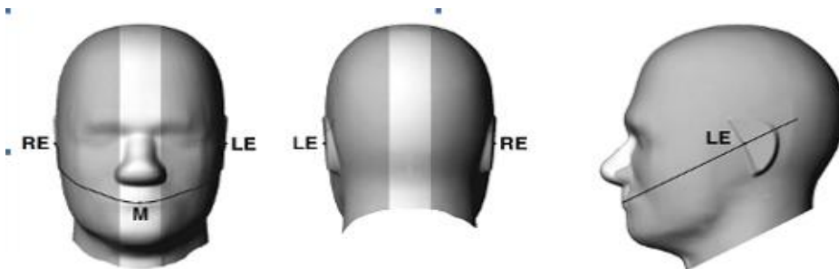
F-2. Front, back, and side views of SAM (model for the phantom shell). Full-head model is for illustration purposes only-procedures in this recommended practice are intended primarily for the phantom setup.
