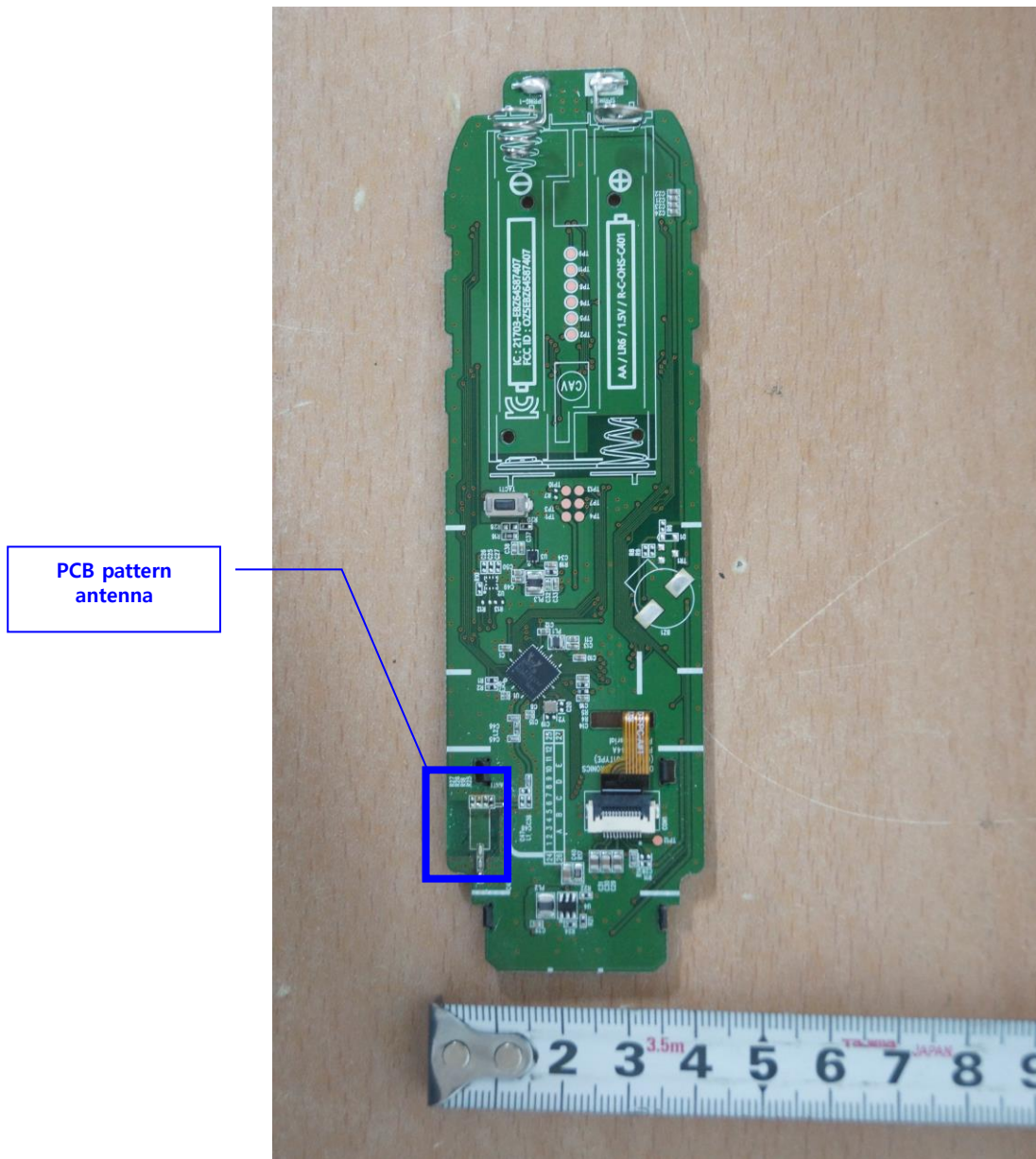
< Main board bottom view >
