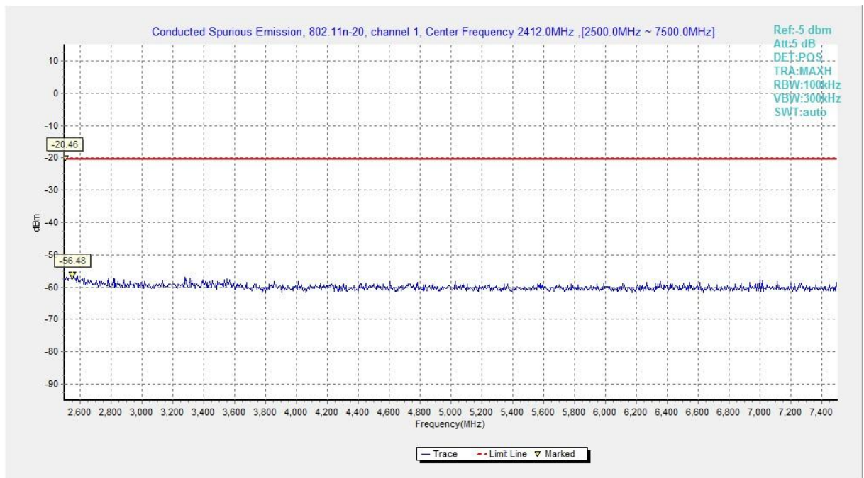
Fig.A.6.1.52 Transmitter Spurious Emission - Conducted (802.11n-HT20, Chain0, Ch1, 2.5 GHz-7.5 GHz)
