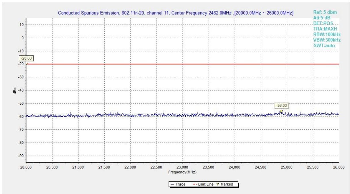
Fig.A.6.1.72 Transmitter Spurious Emission - Conducted (802.11n-HT20, Chain0, Ch11, 20 GHz-26 GHz)
