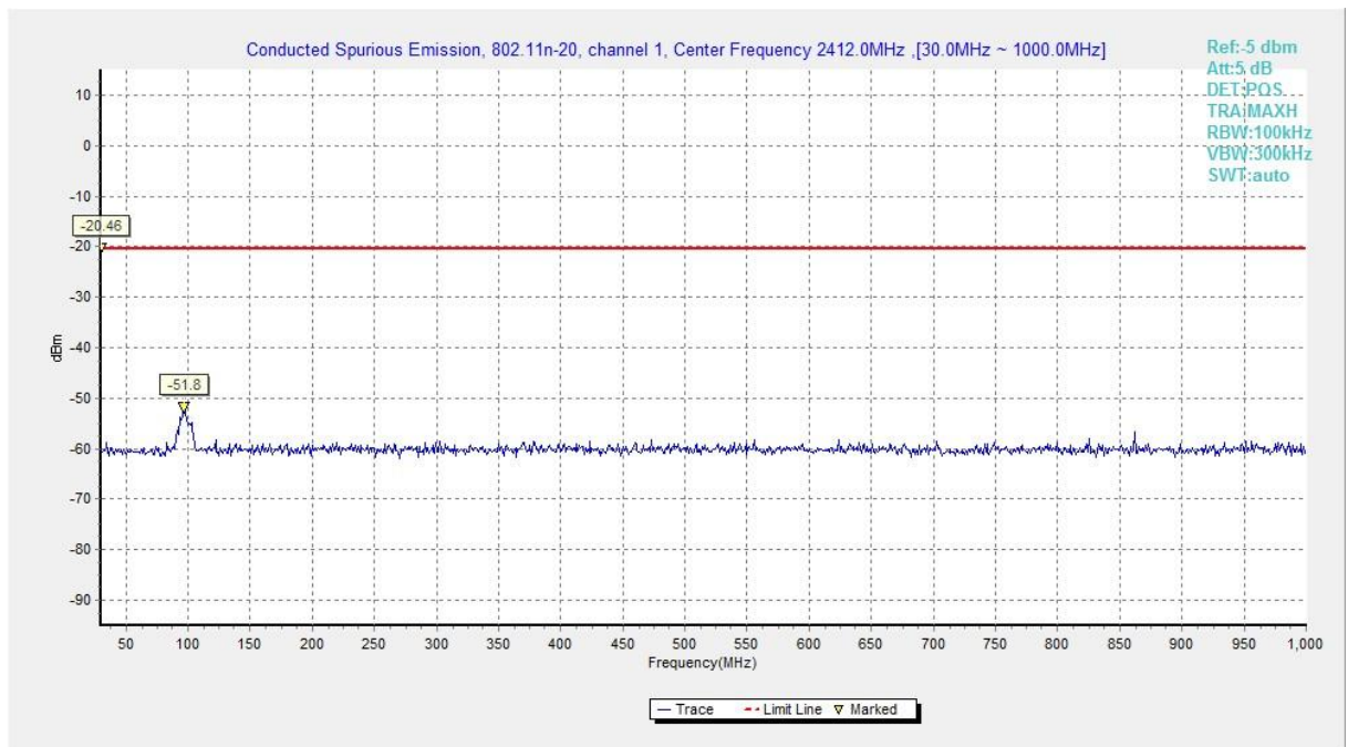
Fig.A.6.1.50 Transmitter Spurious Emission - Conducted (802.11n-HT20, Chain0, Ch1, 30 MHz-1 GHz)
