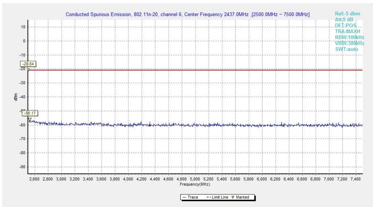
Fig.A.6.1.60 Transmitter Spurious Emission - Conducted (802.11n-HT20, Chain0, Ch6, 2.5 GHz-7.5 GHz)
