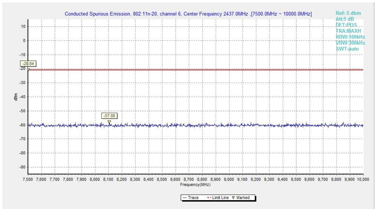
Fig.A.6.1.61 Transmitter Spurious Emission - Conducted (802.11n-HT20, Chain0, Ch6, 7.5 GHz-10 GHz)
