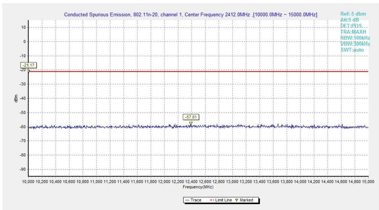
Fig.A.6.1.78 Transmitter Spurious Emission - Conducted (802.11n-HT20, Chain1, Ch1, 10 GHz-15 GHz)
