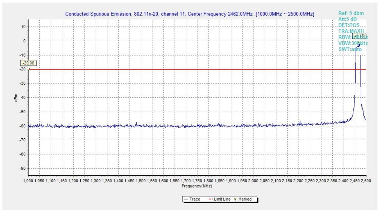
Fig.A.6.1.67 Transmitter Spurious Emission - Conducted (802.11n-HT20, Chain0, Ch11, 1 GHz-2.5 GHz)
