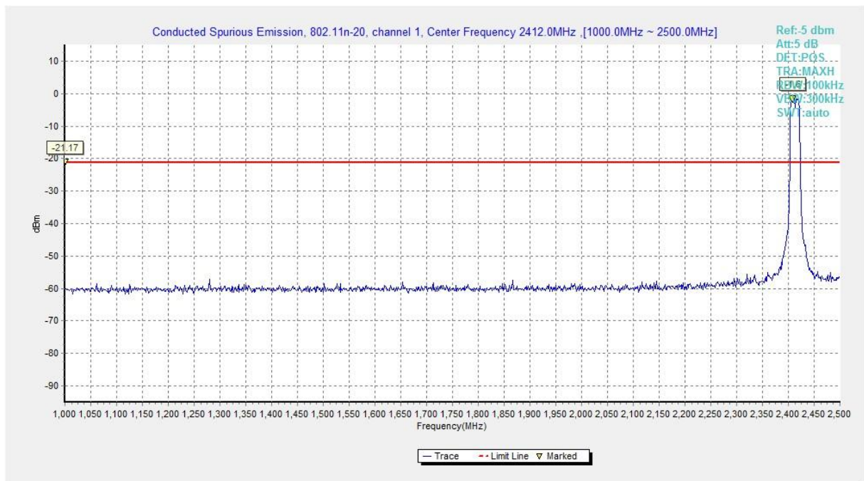
Fig.A.6.1.75 Transmitter Spurious Emission - Conducted (802.11n-HT20, Chain1, Ch1, 1 GHz-2.5 GHz)
