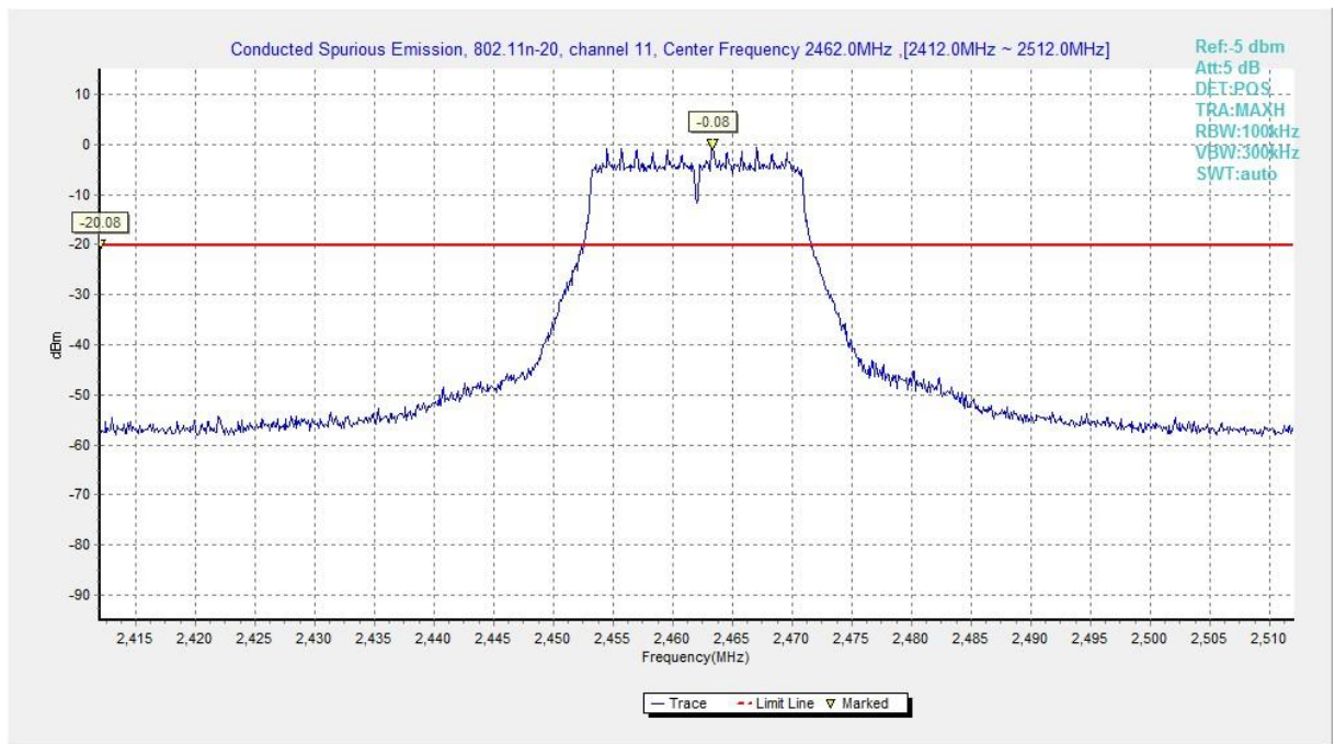
Fig.A.6.1.65 Transmitter Spurious Emission - Conducted (802.11n-HT20, Chain0, Ch11, Center Frequency)
