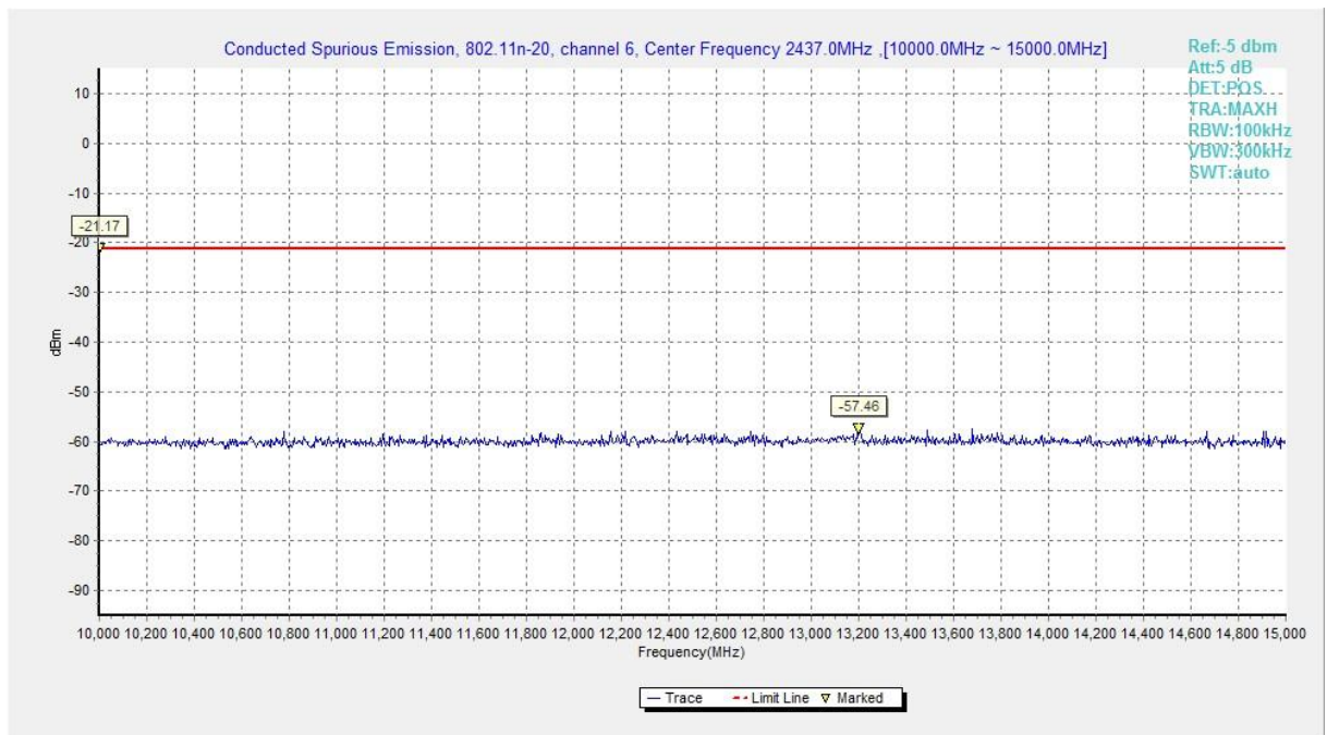
Fig.A.6.1.86 Transmitter Spurious Emission - Conducted (802.11n-HT20, Chain1, Ch6, 10 GHz-15 GHz)
