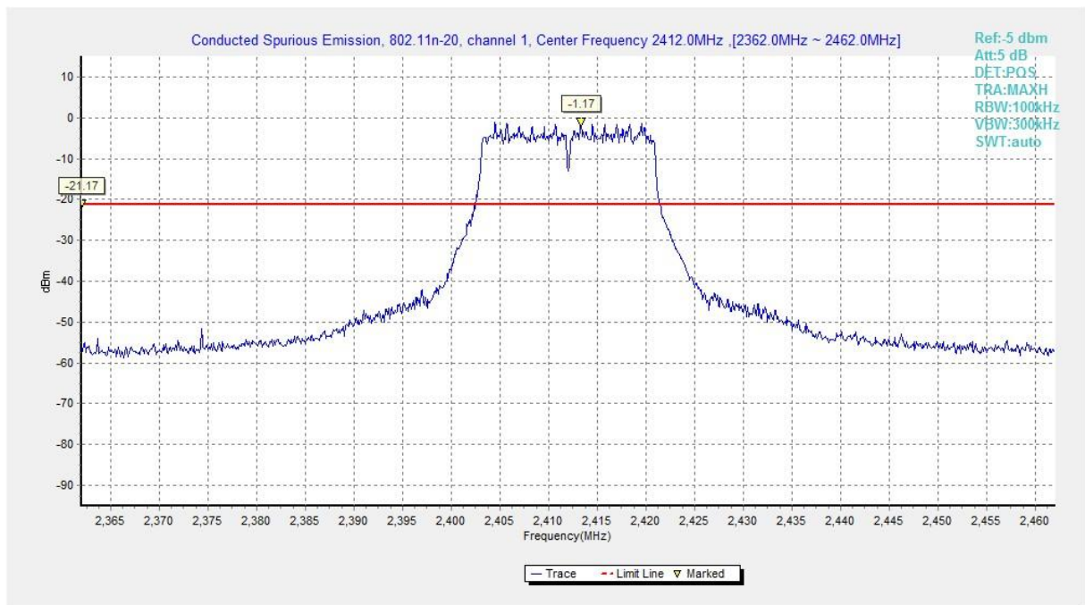
Fig.A.6.1.73 Transmitter Spurious Emission - Conducted (802.11n-HT20, Chain1, Ch1, Center Frequency)
