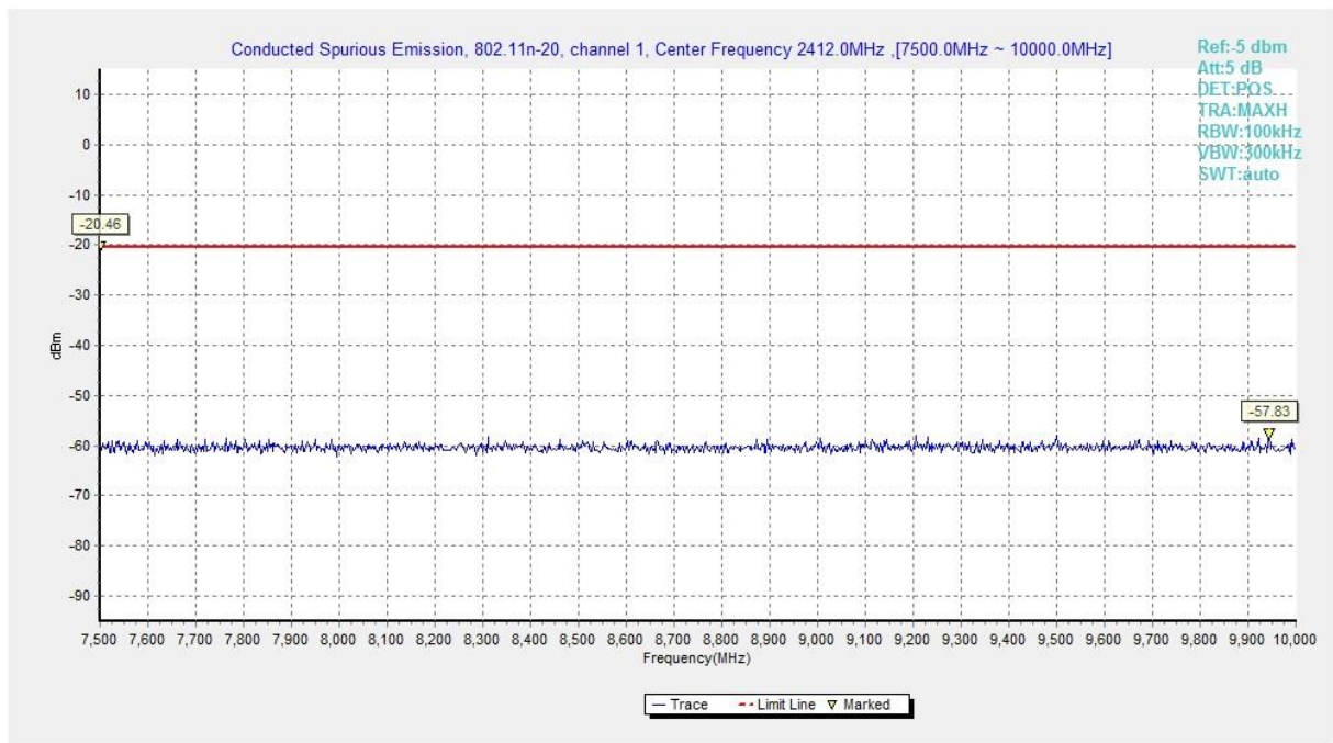
Fig.A.6.1.53 Transmitter Spurious Emission - Conducted (802.11n-HT20, Chain0, Ch1, 7.5 GHz-10 GHz)
