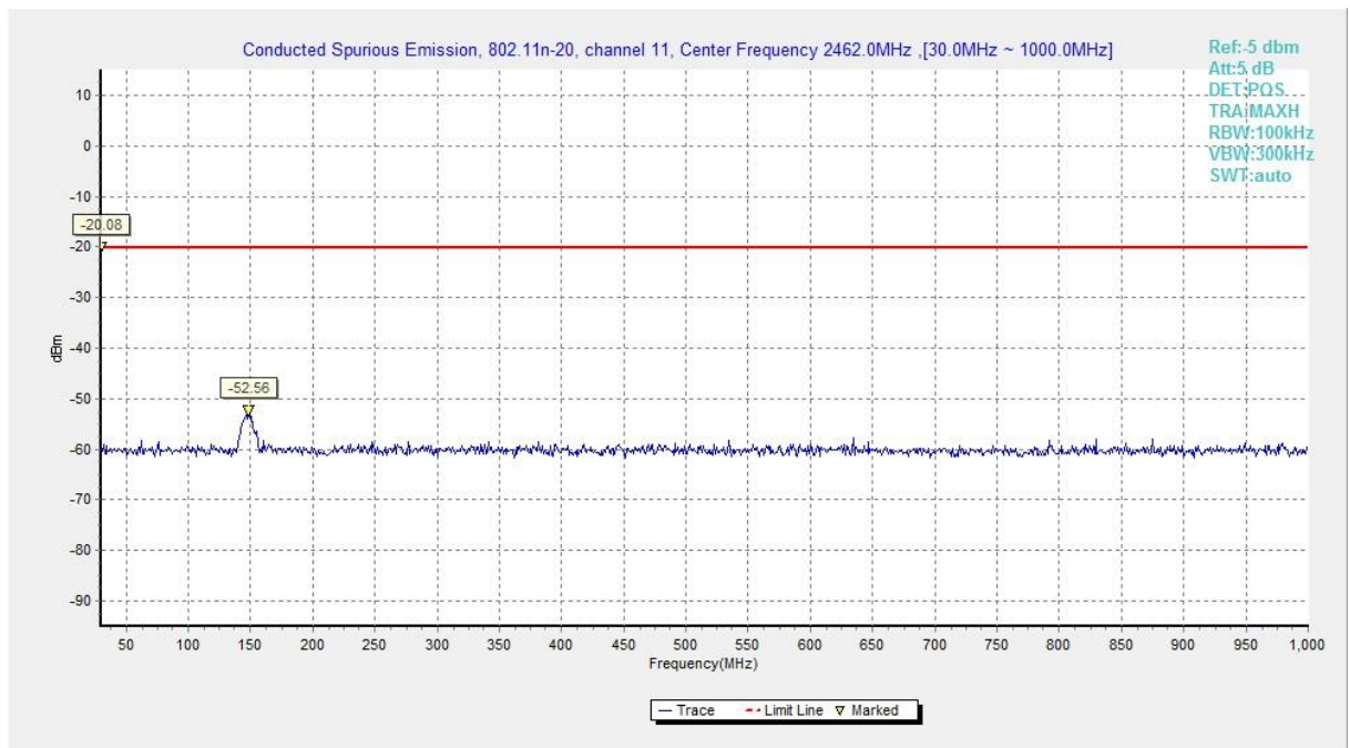
Fig.A.6.1.66 Transmitter Spurious Emission - Conducted (802.11n-HT20, Chain0, Ch11, 30 MHz-1 GHz)
