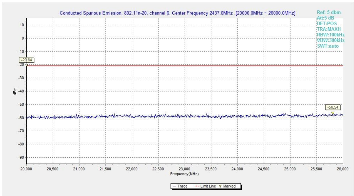
Fig.A.6.1.64 Transmitter Spurious Emission - Conducted (802.11n-HT20, Chain0, Ch6, 20 GHz-26 GHz)
