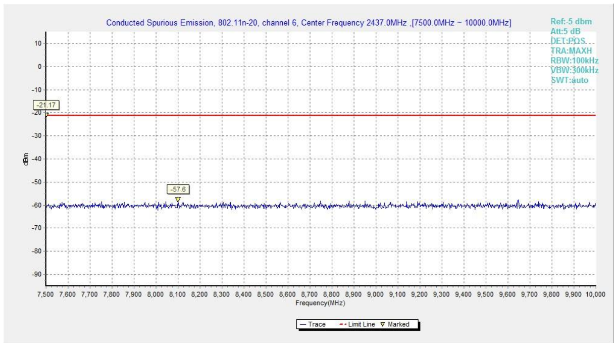
Fig.A.6.1.85 Transmitter Spurious Emission - Conducted (802.11n-HT20, Chain1, Ch6, 7.5 GHz-10 GHz)
