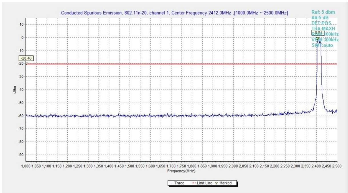
Fig.A.6.1.51 Transmitter Spurious Emission - Conducted (802.11n-HT20, Chain0, Ch1, 1 GHz-2.5 GHz)
