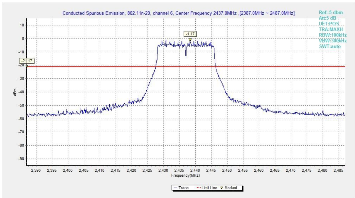
Fig.A.6.1.81 Transmitter Spurious Emission - Conducted (802.11n-HT20, Chain1, Ch6, Center Frequency)
