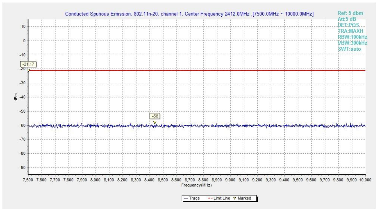
Fig.A.6.1.77 Transmitter Spurious Emission - Conducted (802.11n-HT20, Chain1, Ch1, 7.5 GHz-10 GHz)
