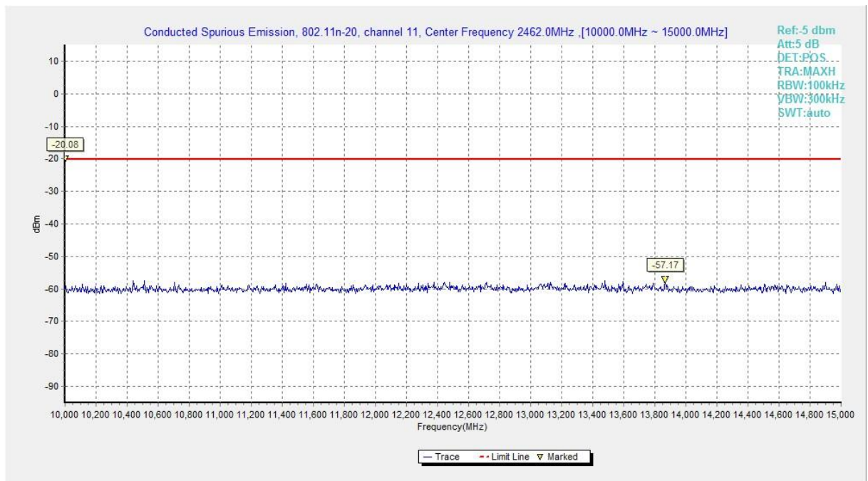
Fig.A.6.1.70 Transmitter Spurious Emission - Conducted (802.11n-HT20, Chain0, Ch11, 10 GHz-15 GHz)
