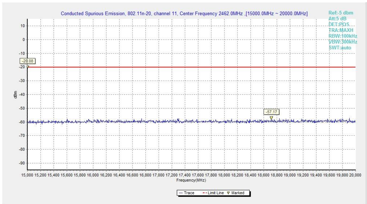
Fig.A.6.1.71 Transmitter Spurious Emission - Conducted (802.11n-HT20, Chain0, Ch11, 15 GHz-20 GHz)
