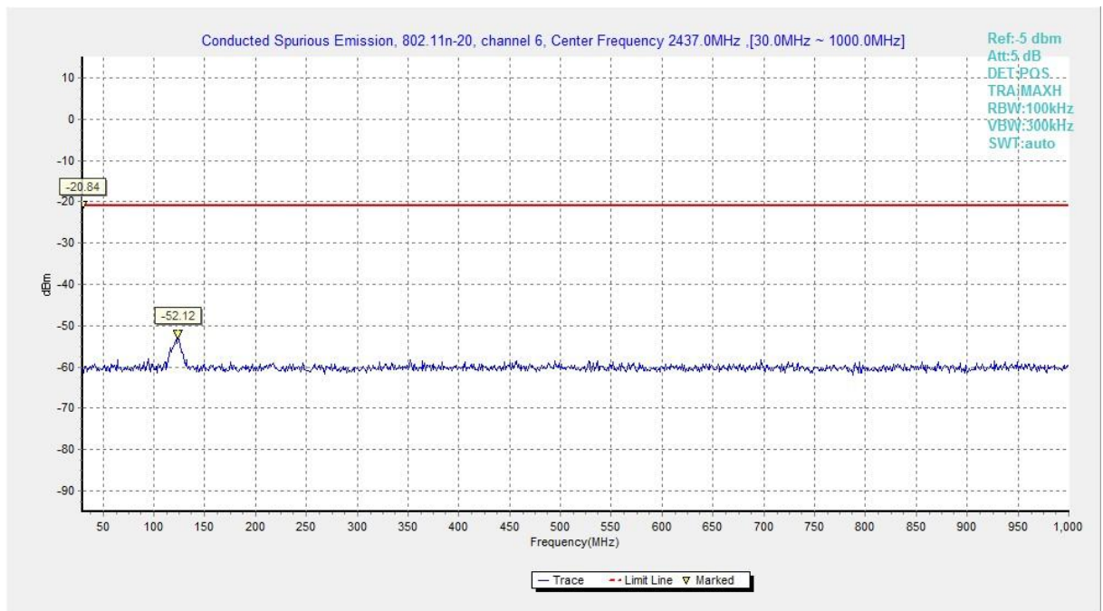
Fig.A.6.1.58 Transmitter Spurious Emission - Conducted (802.11n-HT20, Chain0, Ch6, 30 MHz-1 GHz)
