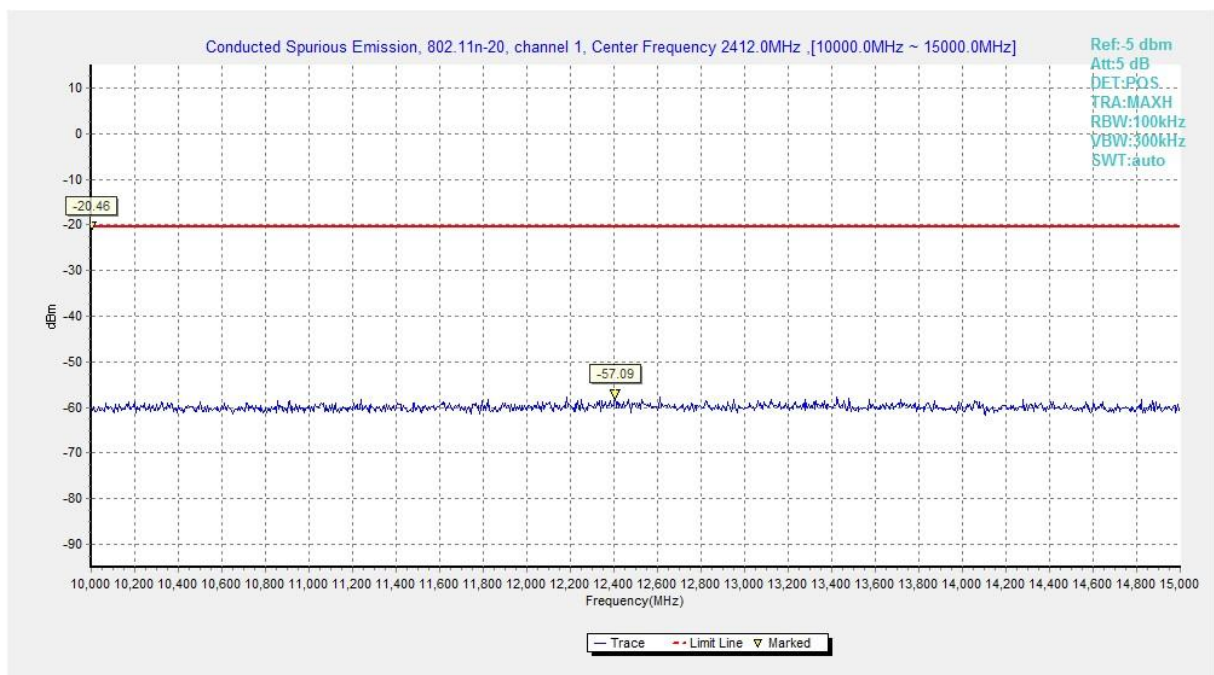
Fig.A.6.1.54 Transmitter Spurious Emission - Conducted (802.11n-HT20, Chain0, Ch1, 10 GHz-15 GHz)
