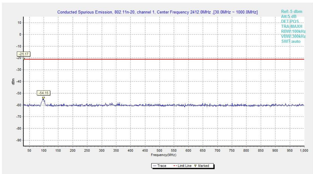
Fig.A.6.1.74 Transmitter Spurious Emission - Conducted (802.11n-HT20, Chain1, Ch1, 30 MHz-1 GHz)
