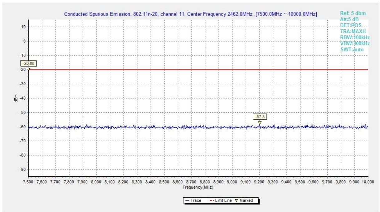
Fig.A.6.1.69 Transmitter Spurious Emission - Conducted (802.11n-HT20, Chain0, Ch11, 7.5 GHz-10 GHz)
