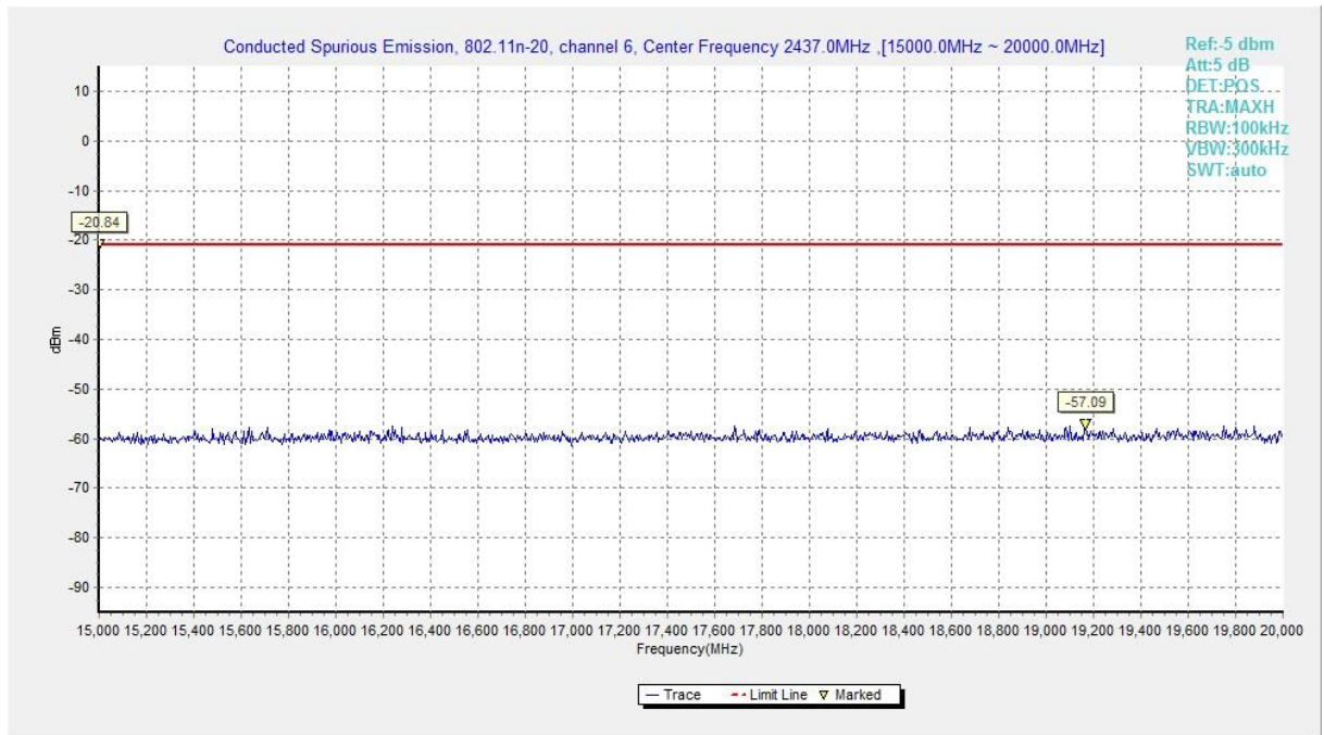
Fig.A.6.1.63 Transmitter Spurious Emission - Conducted (802.11n-HT20, Chain0, Ch6, 15 GHz-20 GHz)
