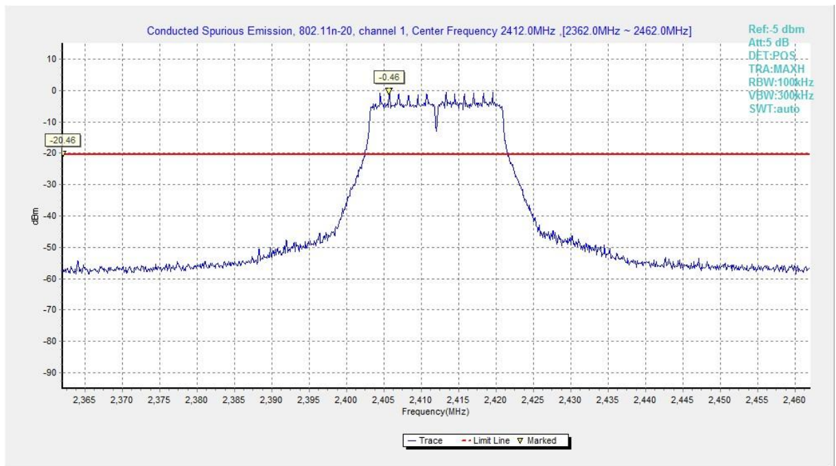
Fig.A.6.1.49 Transmitter Spurious Emission - Conducted (802.11n-HT20, Chain0, Ch1, Center Frequency)
