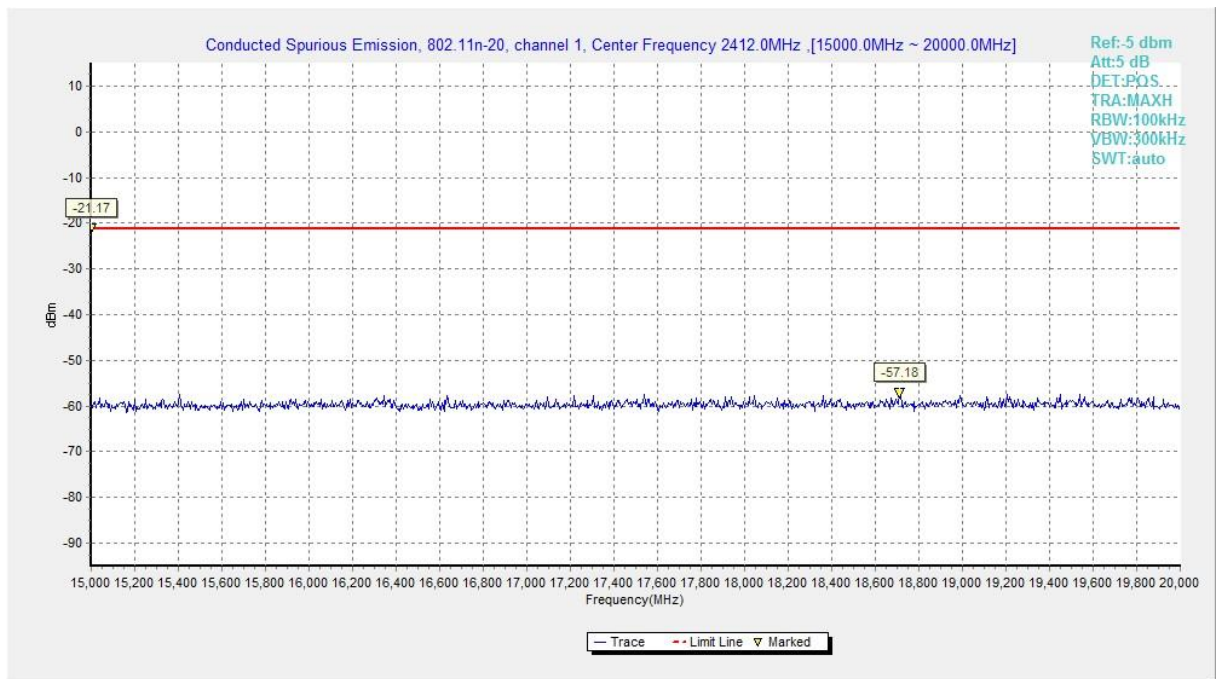
Fig.A.6.1.79 Transmitter Spurious Emission - Conducted (802.11n-HT20, Chain1, Ch1, 15 GHz-20 GHz)
