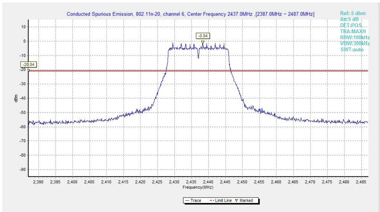
Fig.A.6.1.57 Transmitter Spurious Emission - Conducted (802.11n-HT20, Chain0, Ch6, Center Frequency)
