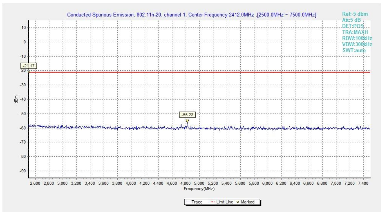
Fig.A.6.1.76 Transmitter Spurious Emission - Conducted (802.11n-HT20, Chain1, Ch1, 2.5 GHz-7.5 GHz)
