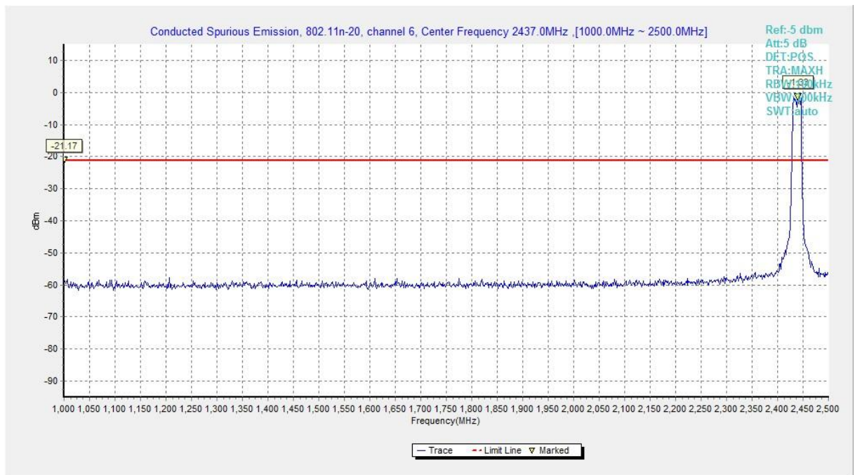
Fig.A.6.1.83 Transmitter Spurious Emission - Conducted (802.11n-HT20, Chain1, Ch6, 1 GHz-2.5 GHz)
