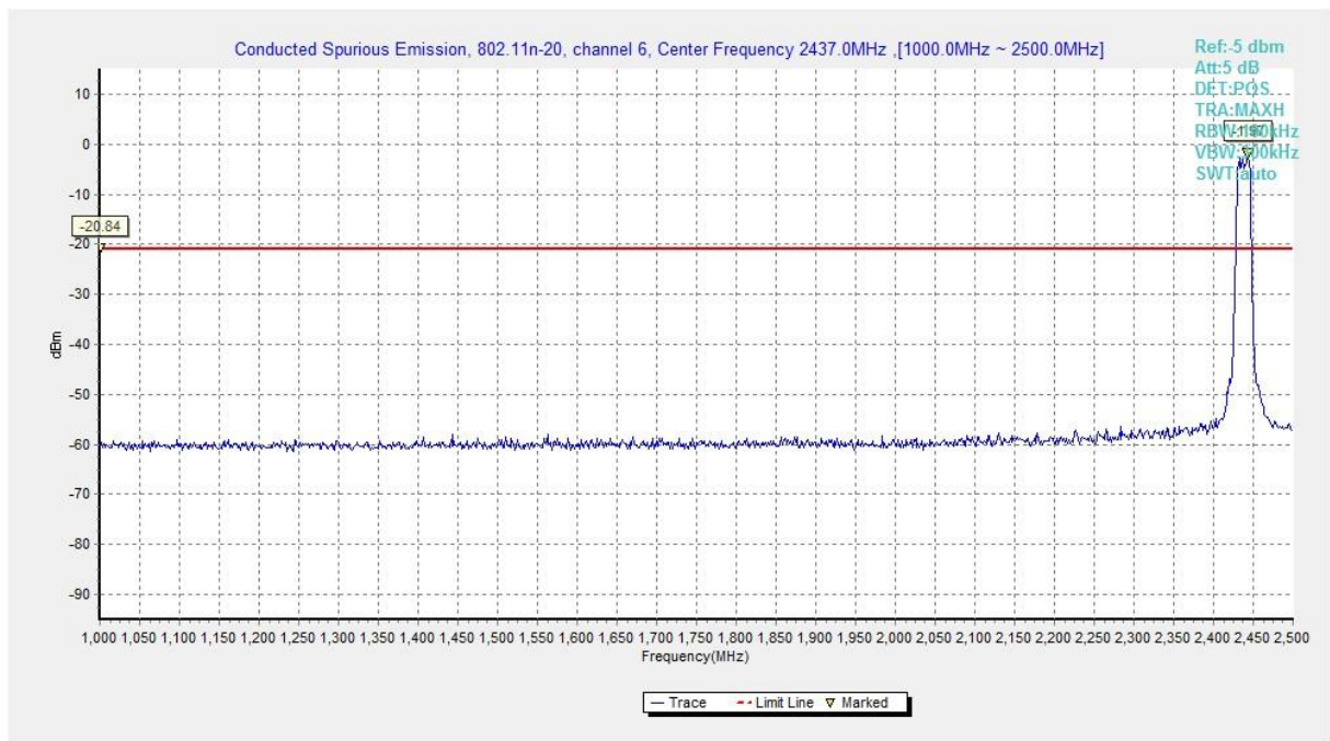
Fig.A.6.1.59 Transmitter Spurious Emission - Conducted (802.11n-HT20, Chain0, Ch6, 1 GHz-2.5 GHz)
