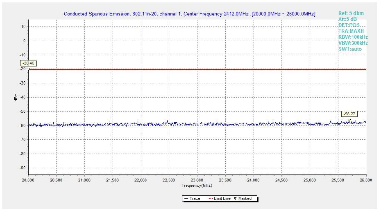
Fig.A.6.1.56 Transmitter Spurious Emission - Conducted (802.11n-HT20, Chain0, Ch1, 20 GHz-26 GHz)
