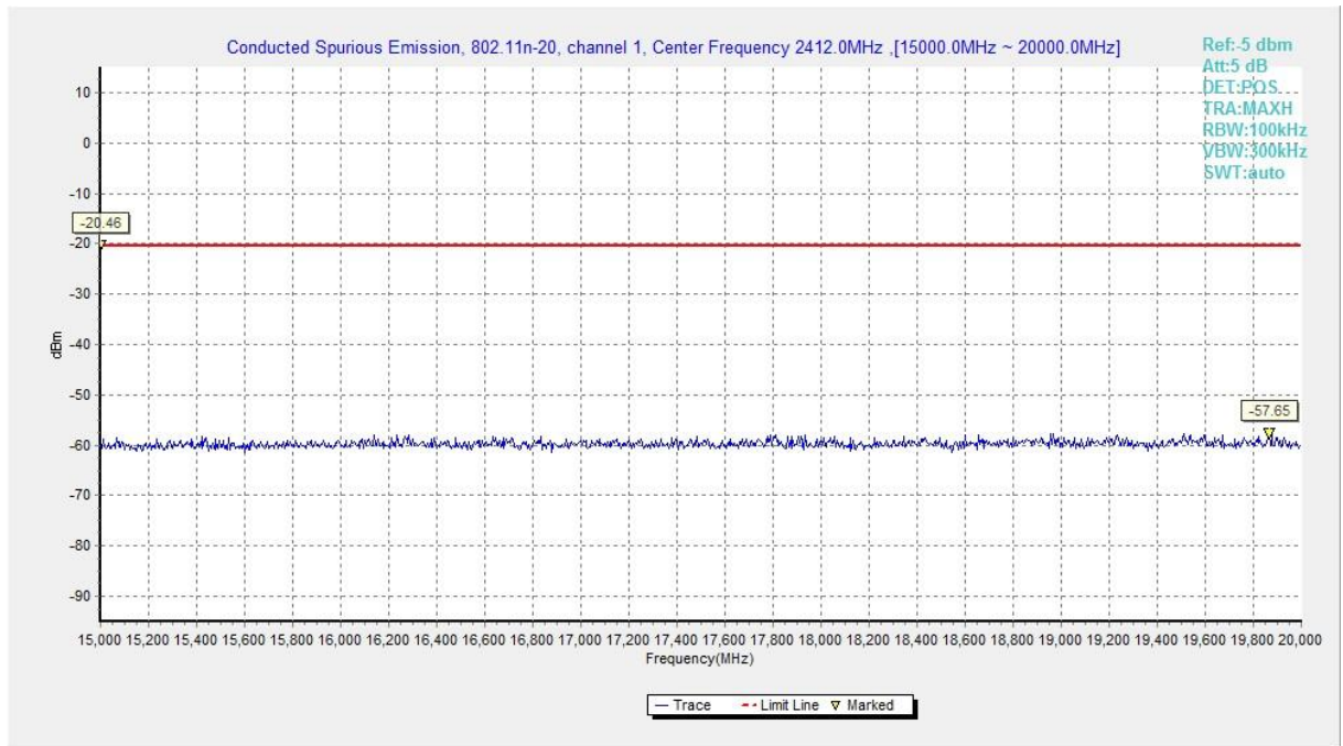
Fig.A.6.1.55 Transmitter Spurious Emission - Conducted (802.11n-HT20, Chain0, Ch1, 15 GHz-20 GHz)
