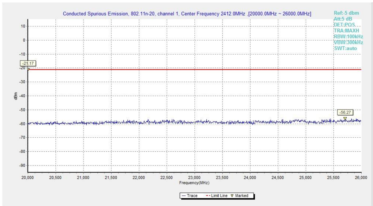
Fig.A.6.1.80 Transmitter Spurious Emission - Conducted (802.11n-HT20, Chain1, Ch1, 20 GHz-26 GHz)
