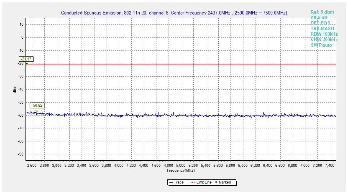
Fig.A.6.1.84 Transmitter Spurious Emission - Conducted (802.11n-HT20, Chain1, Ch6, 2.5 GHz-7.5 GHz)
