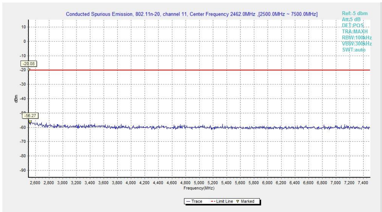
Fig.A.6.1.68 Transmitter Spurious Emission - Conducted (802.11n-HT20, Chain0, Ch11, 2.5 GHz-7.5 GHz)
