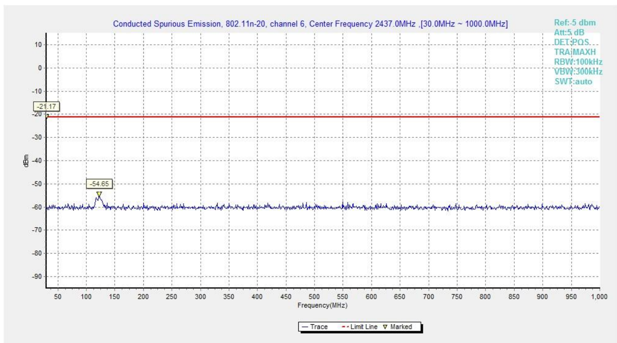
Fig.A.6.1.82 Transmitter Spurious Emission - Conducted (802.11n-HT20, Chain1, Ch6, 30 MHz-1 GHz)
