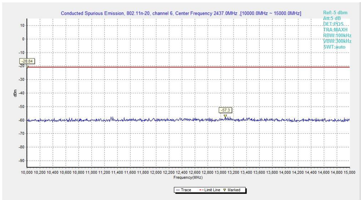
Fig.A.6.1.62 Transmitter Spurious Emission - Conducted (802.11n-HT20, Chain0, Ch6, 10 GHz-15 GHz)
