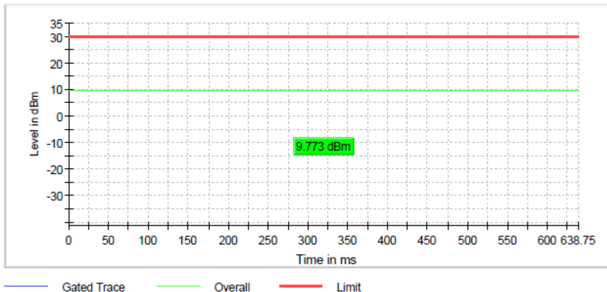
Figure 6: Conducted power, RF I/O port 1_802.11g_9Mbps_Channel 1
