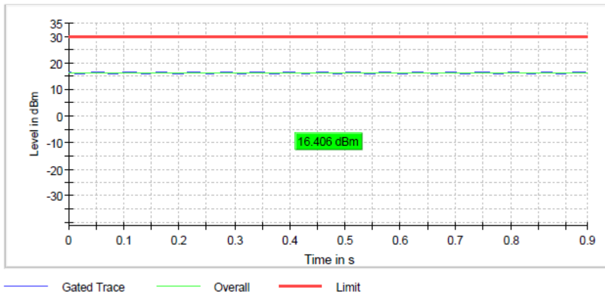
Figure 4: Conducted power, RF I/O port 1_802.11b_1Mbps_Channel 6
