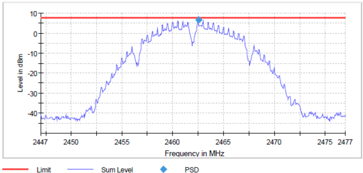
Figure 118: Power spectral density, RF I/O port 1_802.11b_1Mbps_Channel 11
