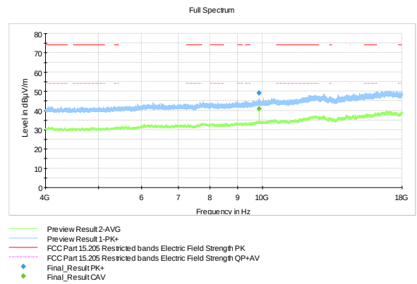
Figure 65: HIGH channel (4 GHz – 18 GHz)
