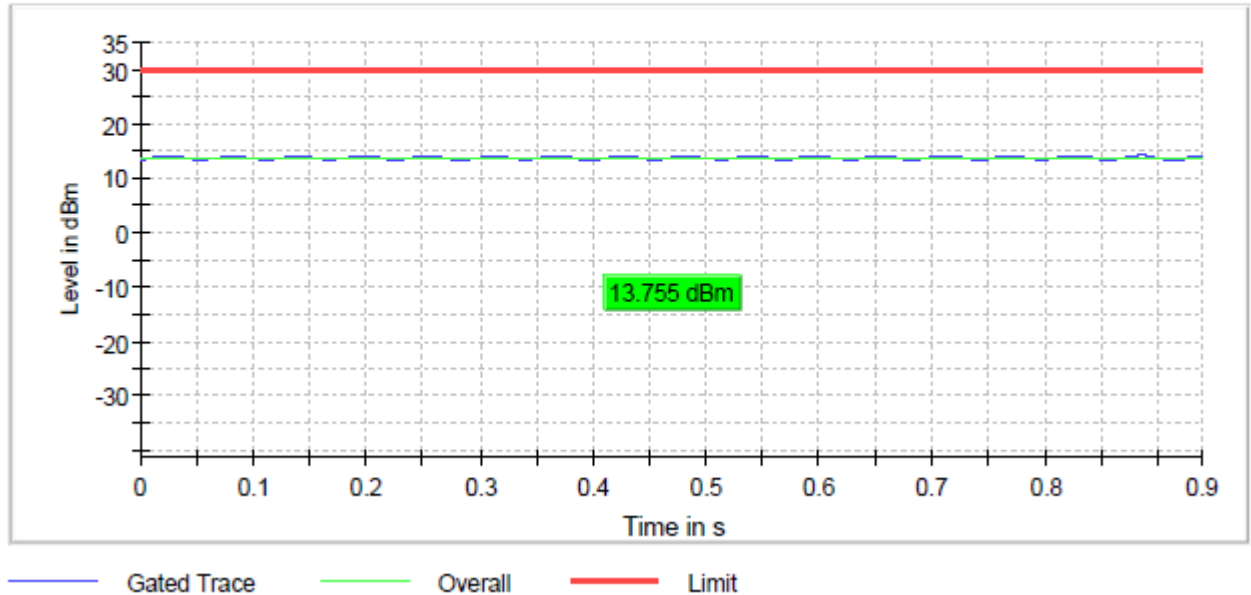
Figure 13: Conducted power, RF I/O port 2_802.11b_1Mbps_Channel 11
