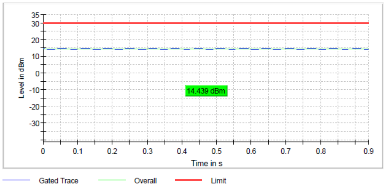
Figure 3: Conducted power, RF I/O port 1_802.11b_1Mbps_Channel 1
