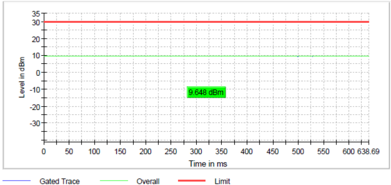
Figure 8: Conducted power, RF I/O port 1_802.11g_9Mbps_Channel 11
