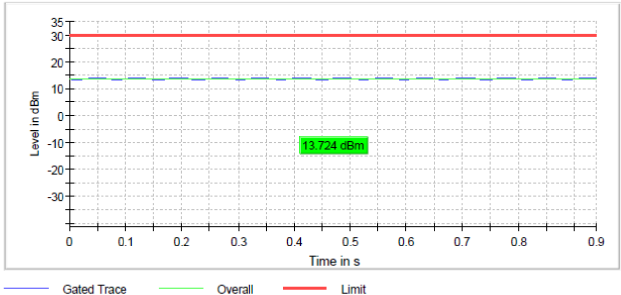
Figure 12: Conducted power, RF I/O port 2_802.11b_1Mbps_Channel 1
