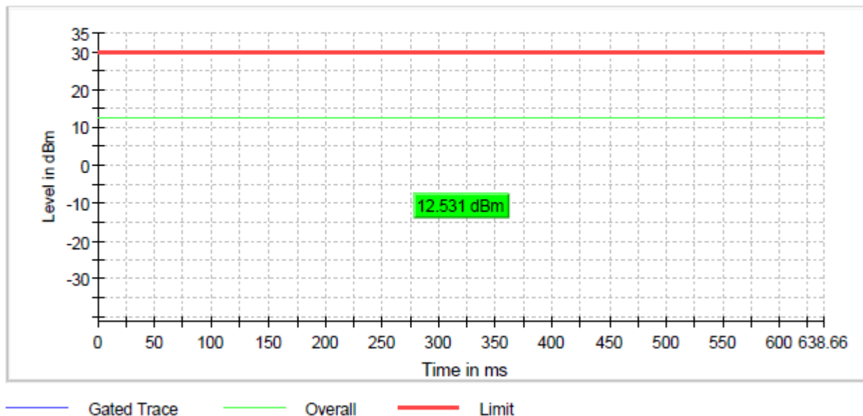
Figure 15: Conducted power, RF I/O port 2_802.11g_9Mbps_Channel 6
