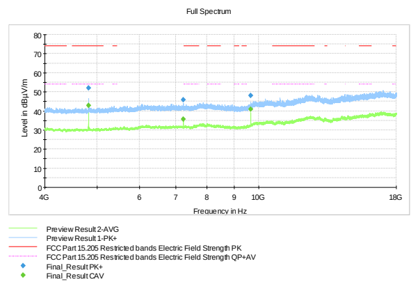
Figure 23: LOW channel (4 GHz – 18 GHz)
