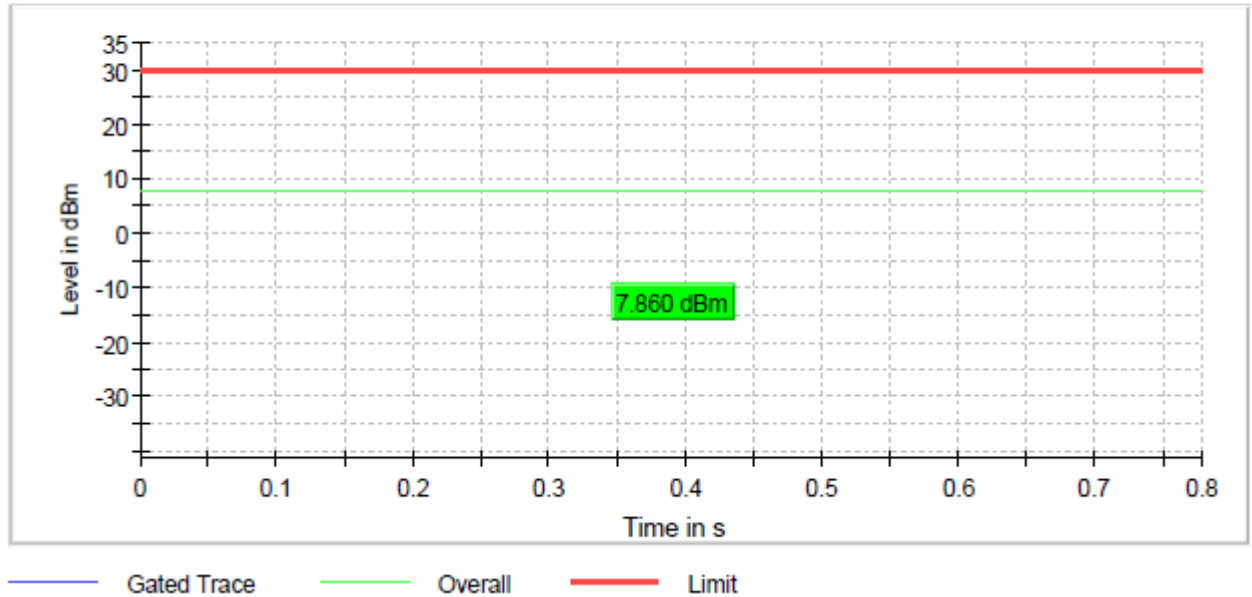
Figure 19: Conducted power, RF I/O port 2_802.11n_14.4Mbps (MCS1)_Channel 11
