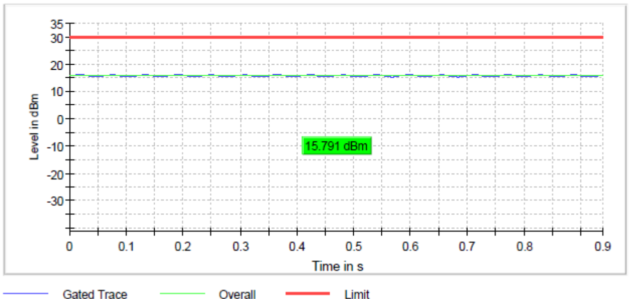
Figure 4: Conducted power, RF I/O port 2_802.11b_1Mbps_Channel 6
