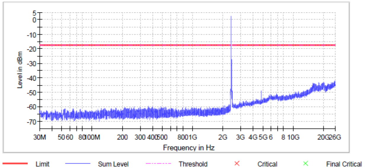
Figure 80: Conducted spurious emissions 30 - 26500 MHz LOW channel
