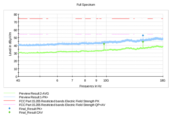
Figure 60: MID channel (4 GHz – 18 GHz)
