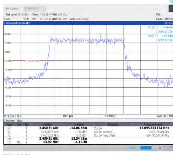
1-N78-3450-3550--30-15-L-1-DFT-QPSK-Outer_Full- 36@0-Ant1-12.895-13.920-≤15-PASS
