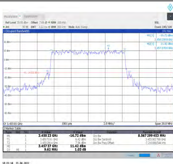
1-N78-3450-3550--30-10-L-7-CP-16QAM-Outer_Full -24@0-Ant1-8.567-9.620-≤10-PASS
