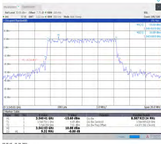
1-N78-3450-3550--30-10-H-7-CP-16QAM-Outer_Full -24@0-Ant1-8.588-9.320-≤10-PASS
