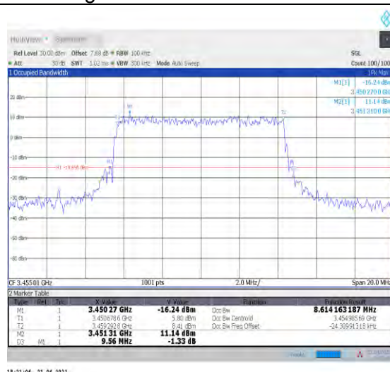
1-N78-3450-3550--30-10-L-6-CP-QPSK-Outer_Full -24@0-Ant1-8.614-9.560-≤10-PASS
