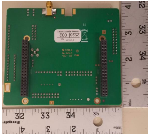
Figure B3. DUT Module only rear view
