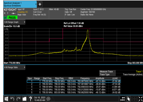
N14(5M)_DFT-s- OFDM_QPSK_Edge_1RB_Right_Low_CH
