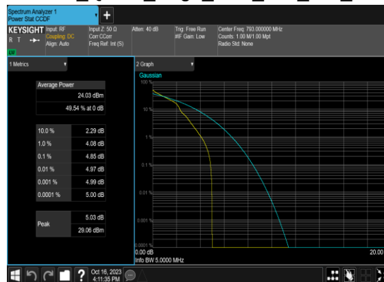
N14(5M)_DFT-s-OFDM_QPSK_Edge_1RB_Left_Mid_CH
