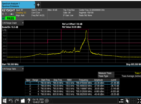
N14(5M)_DFT-s- OFDM_BPSK_Edge_1RB_Right_Mid_CH
