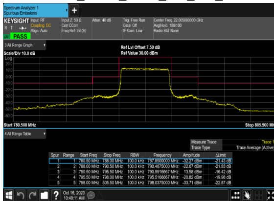
N14(5M)_DFT-s- OFDM_BPSK_Outer_Full_Mid_CH
