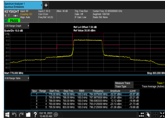
N14(5M)_DFT-s- OFDM_QPSK_Outer_Full_Low_CH
