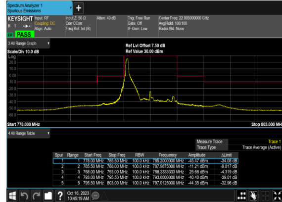
N14(5M)_DFT-s- OFDM_QPSK_Edge_1RB_Left_Low_CH
