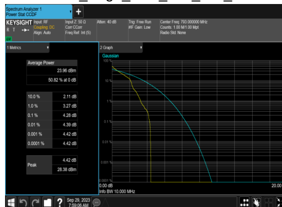
N14(10M)_DFT-s-OFDM_PI_2-BPSK_Edge_1RB_Left_Mid_CH
