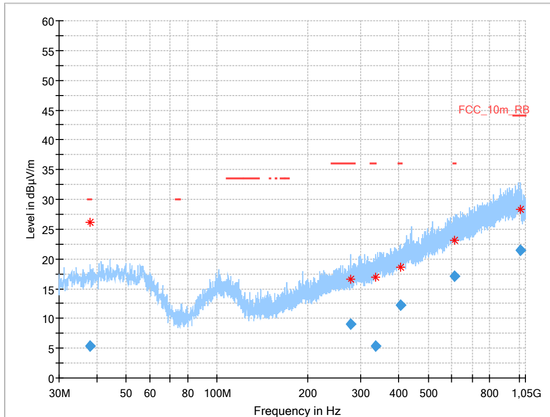
Plot 2: 30 MHz to 1 GHz, vertical & horizontal polarization, valid for all channels of 2 Msps mode
