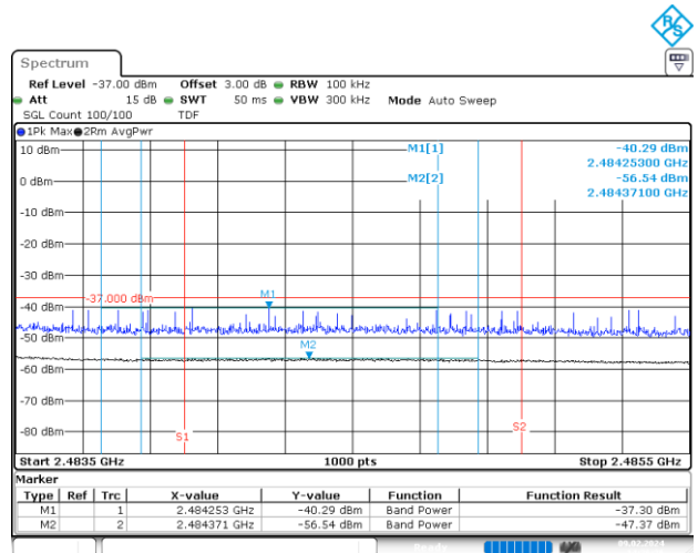
-BE-R-HIGH-2MHz, SISO-A, 802.11ax20-HE0, Ch13
