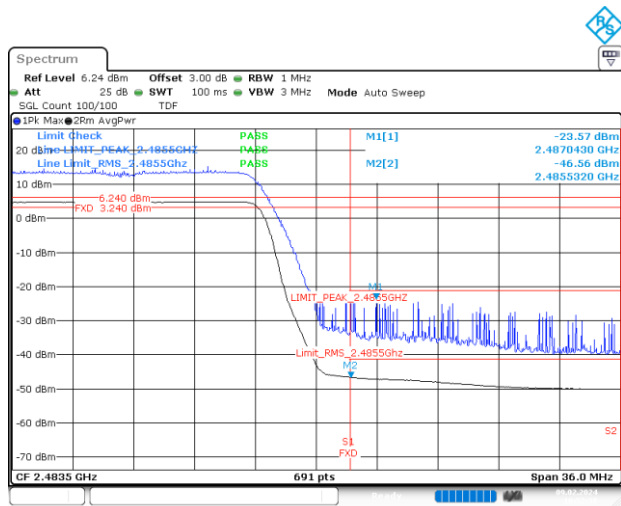
BE-R-HIGH, SISO-A, 802.11g-6Mbps, Ch13
