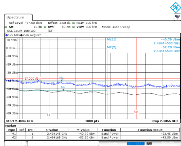
BE-R-HIGH-2MHz, SISO-A, 802.11g-6Mbps, Ch12
