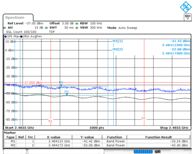
BE-R-HIGH-2MHz, SISO-A, 802.11n20-HT0, Ch12
