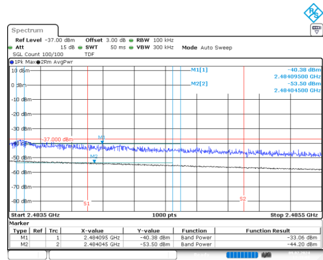
BE-R-HIGH-2MHz, SISO-A, 802.11ax40-HE0, Ch10
