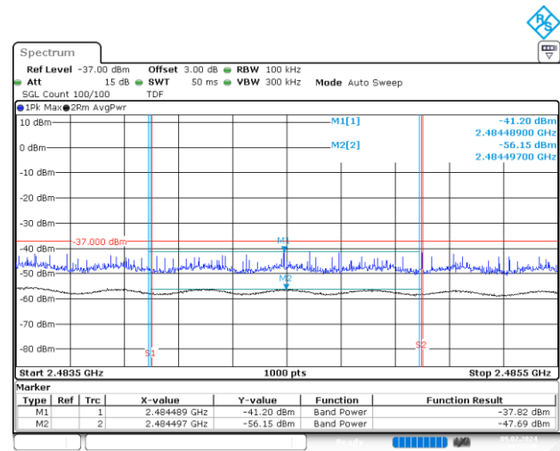
BE-R-HIGH-2MHz, SISO-A, 802.11g-6Mbps, Ch13
