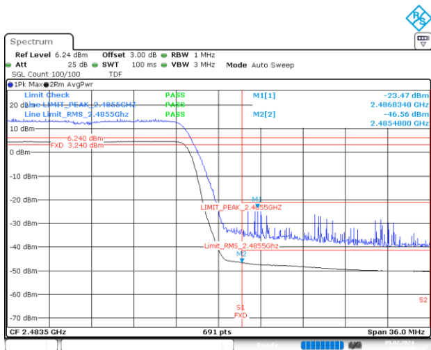
BE-R-HIGH, SISO-A, 802.11n20-HT0, Ch13
