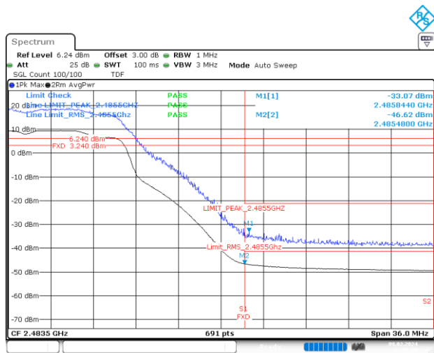
BE-R-HIGH, SISO-A, 802.11g-6Mbps, Ch12
