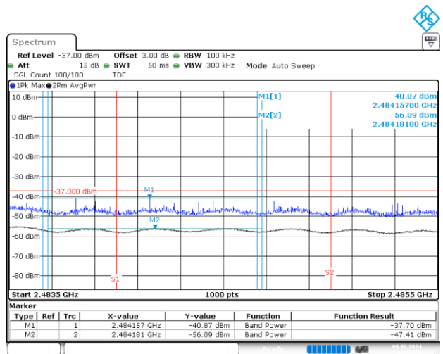
BE-R-HIGH-2MHz, SISO-A, 802.11n20-HT0, Ch13
