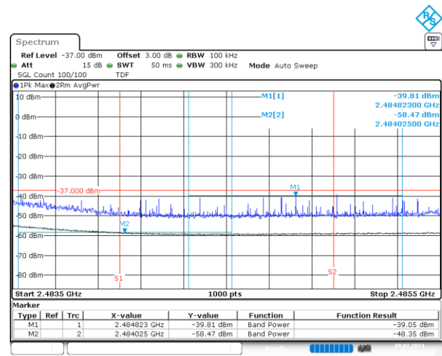
BE-R-HIGH-2MHz, SISO-A, 802.11ax40-HE0, Ch11
