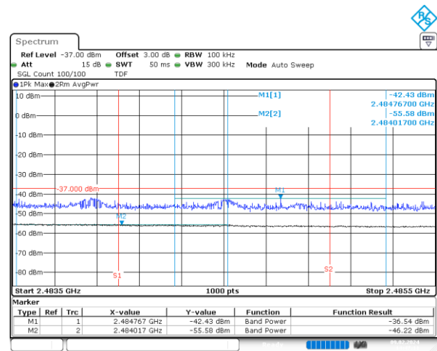
BE-R-HIGH-2MHz, SISO-A, 802.11ax40-HE0, Ch9
