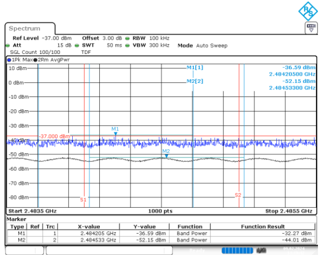
BE-R-HIGH-2MHz, SISO-A, 802.11n20-HT0, Ch11
