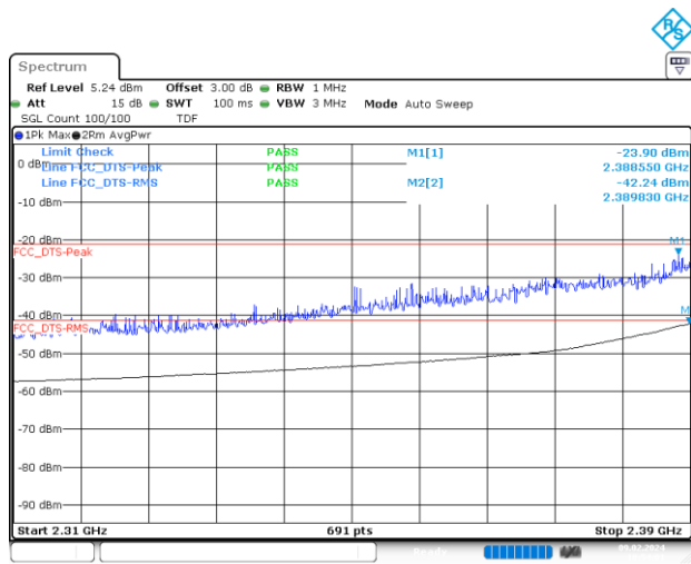
BE-R-LOW, SISO-A, 802.11n20-HT0, Ch1
