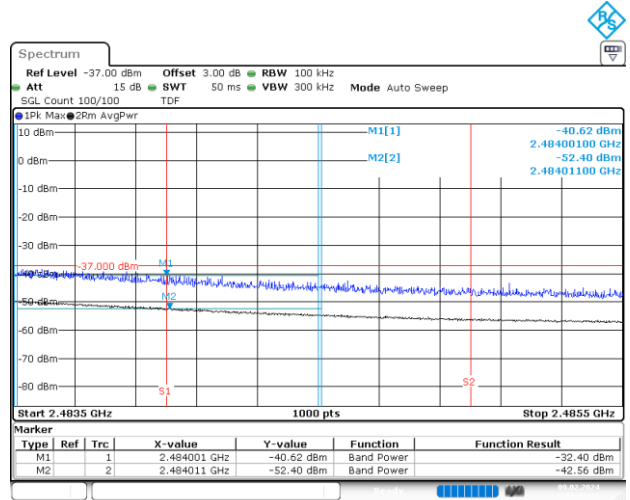
BE-R-HIGH-2MHz, SISO-A, 802.11ax20-HE0, Ch12
