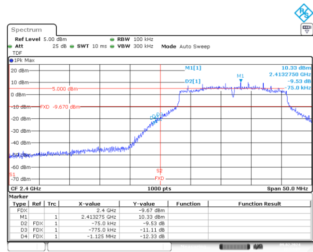
BE-NR, SISO-A, 802.11n20-HT0, Ch1
