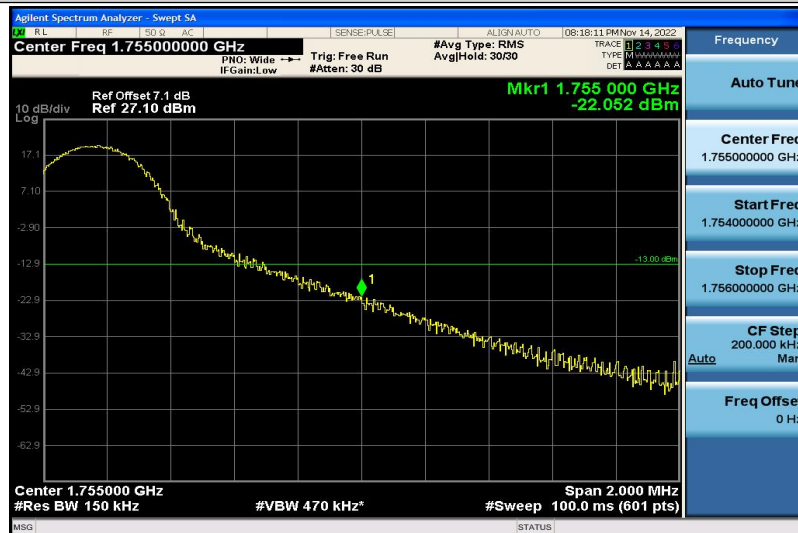
Band4-15MHz-16QAM-20325-1RB#74
