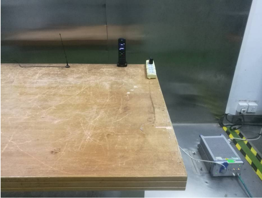
Conducted Emissions - Front View(Adapter: HJ-0600400A1-US)
