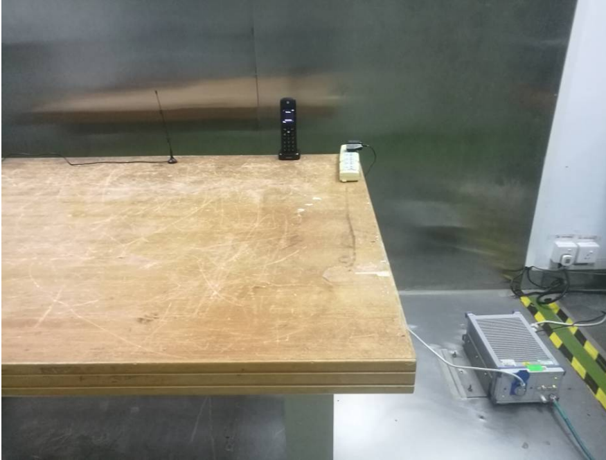
Conducted Emissions - Front View(Adapter: BLJ05W060040P-UA)
