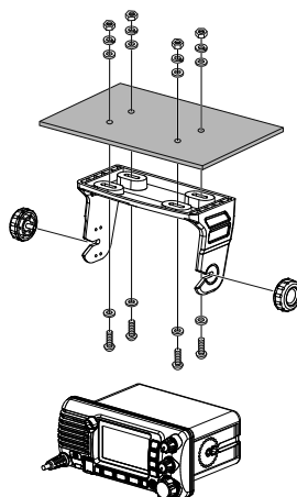
Overhead Mounting
