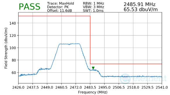
Plot 7-114. Radiated Restricted Upper Band Edge Measurement (Peak)
