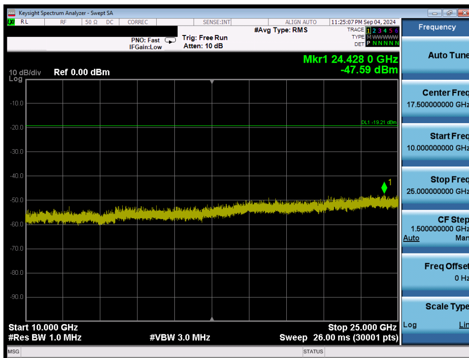
Plot 7-97. Conducted Spurious Plot (802.11b – Ch. 6) SISO ANT2
