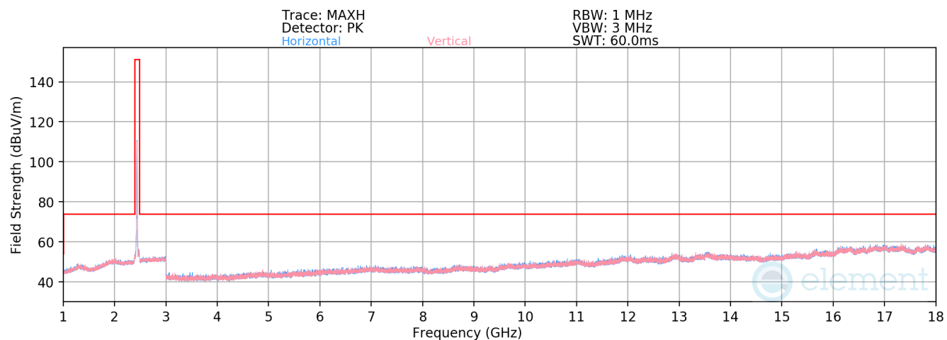
Plot 7-102. Radiated Spurious Plot above 1GHz (802.11n – Ch. 6) MIMO
