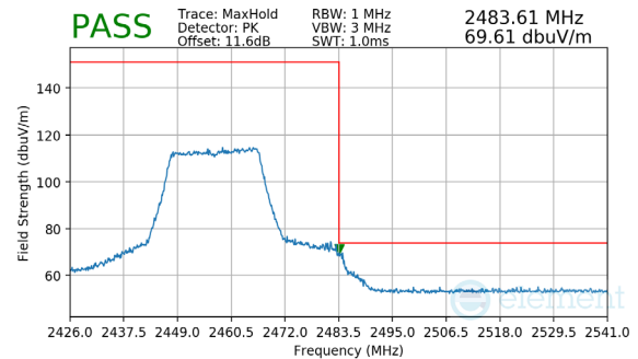
Plot 7-110. Radiated Restricted Upper Band Edge Measurement (Peak)
