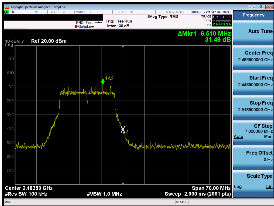
Plot 7-81. Band Edge Plot (802.11n/ac (2.4GHz) - Ch. 13) MIMO ANT2
