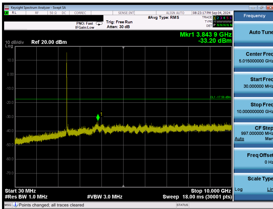
Plot 7-88. Conducted Spurious Plot (802.11b – Ch. 1) SISO ANT1
