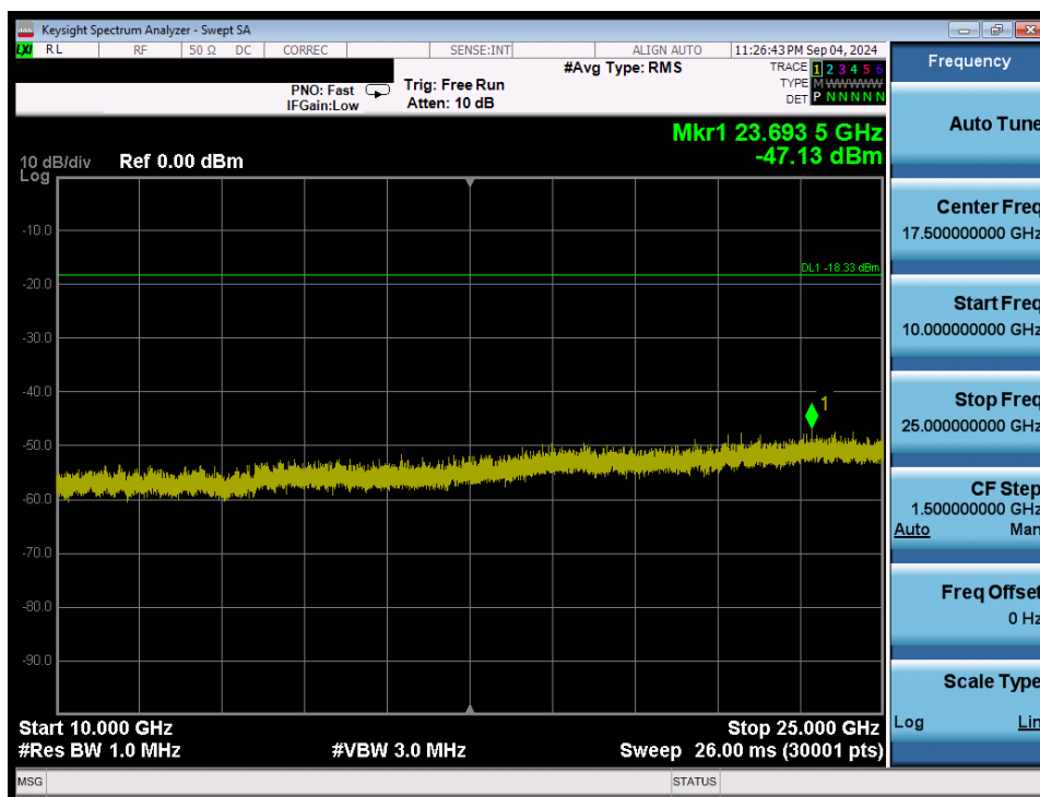
Plot 7-95. Conducted Spurious Plot (802.11b – Ch. 1) SISO ANT2
