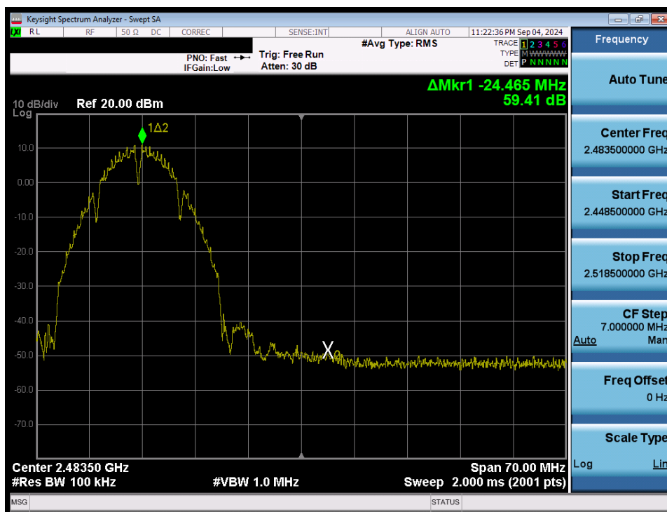
Plot 7-71. Band Edge Plot (802.11b – Ch. 11) SISO ANT2
