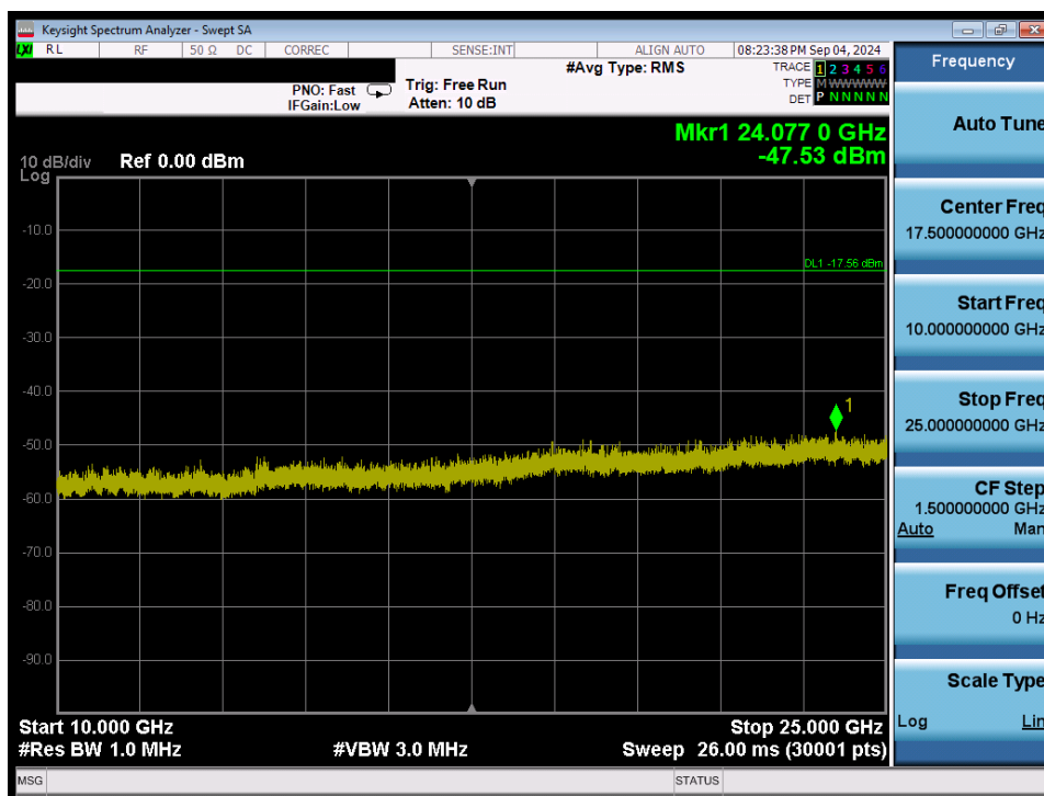
Plot 7-89. Conducted Spurious Plot (802.11b – Ch. 1) SISO ANT1
