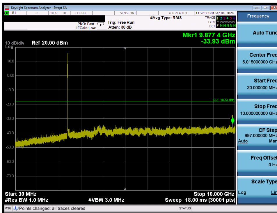
Plot 7-94. Conducted Spurious Plot (802.11b – Ch. 1) SISO ANT2
