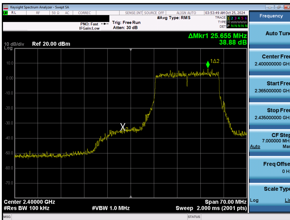
Plot 7-83. Band Edge Plot (802.11ax/be (2.4GHz) – Ch. 2) MIMO ANT2
