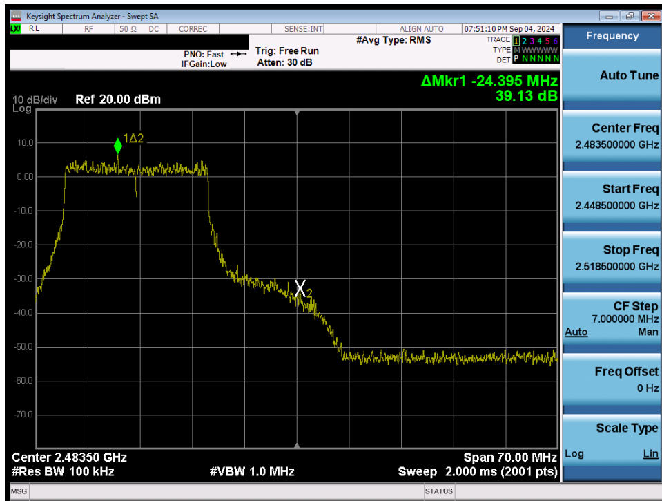
Plot 7-67. Band Edge Plot (802.11ax/be (2.4GHz) – Ch. 11) MIMO ANT1
