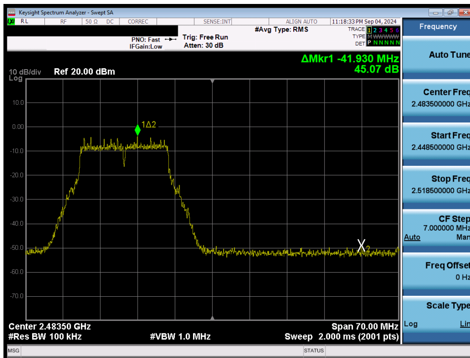
Plot 7-76. Band Edge Plot (802.11g – Ch. 12) MIMO ANT2
