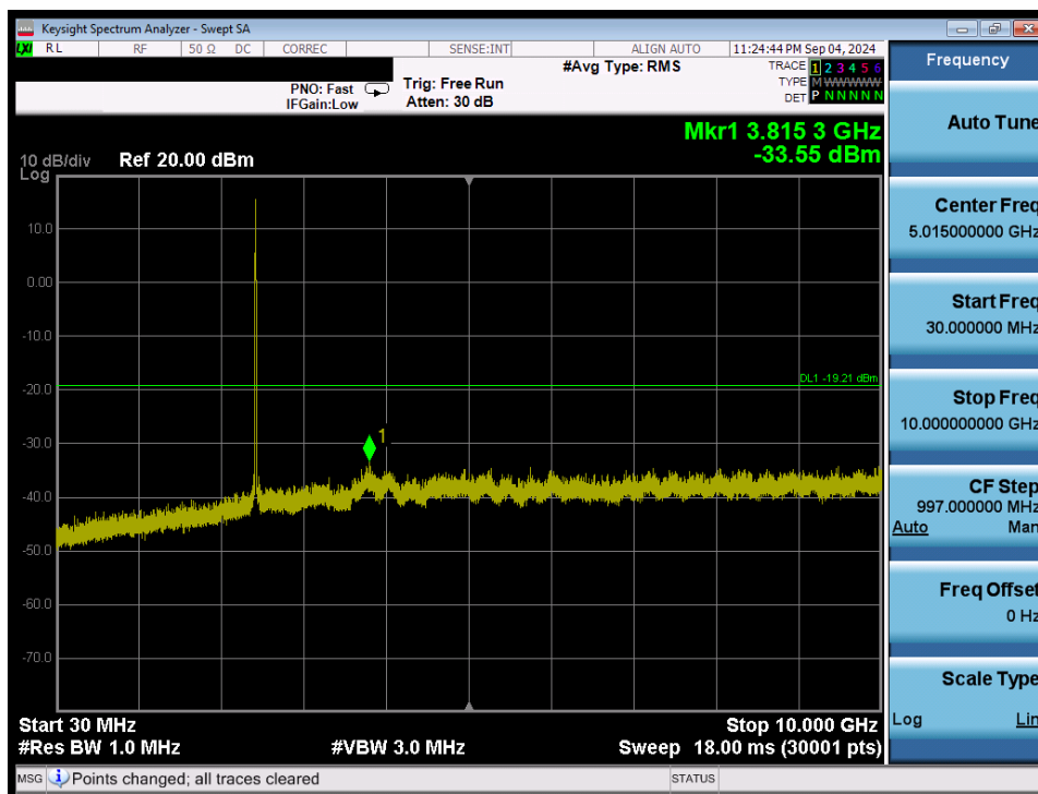
Plot 7-96. Conducted Spurious Plot (802.11b – Ch. 6) SISO ANT2
