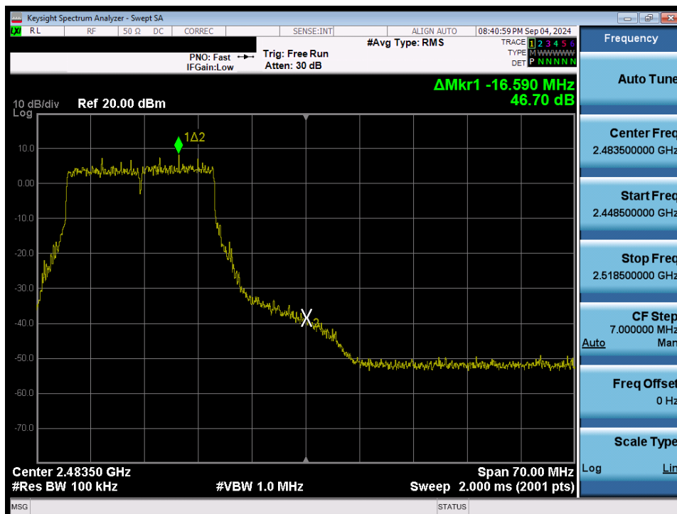
Plot 7-85. Band Edge Plot (802.11ax/be (2.4GHz) – Ch. 11) MIMO ANT2
