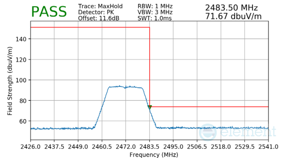
Plot 7-116. Radiated Restricted Upper Band Edge Measurement (Peak)
