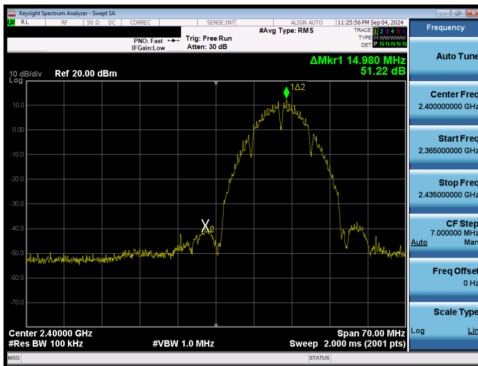
Plot 7-70. Band Edge Plot (802.11b – Ch. 1) – SISO ANT2
