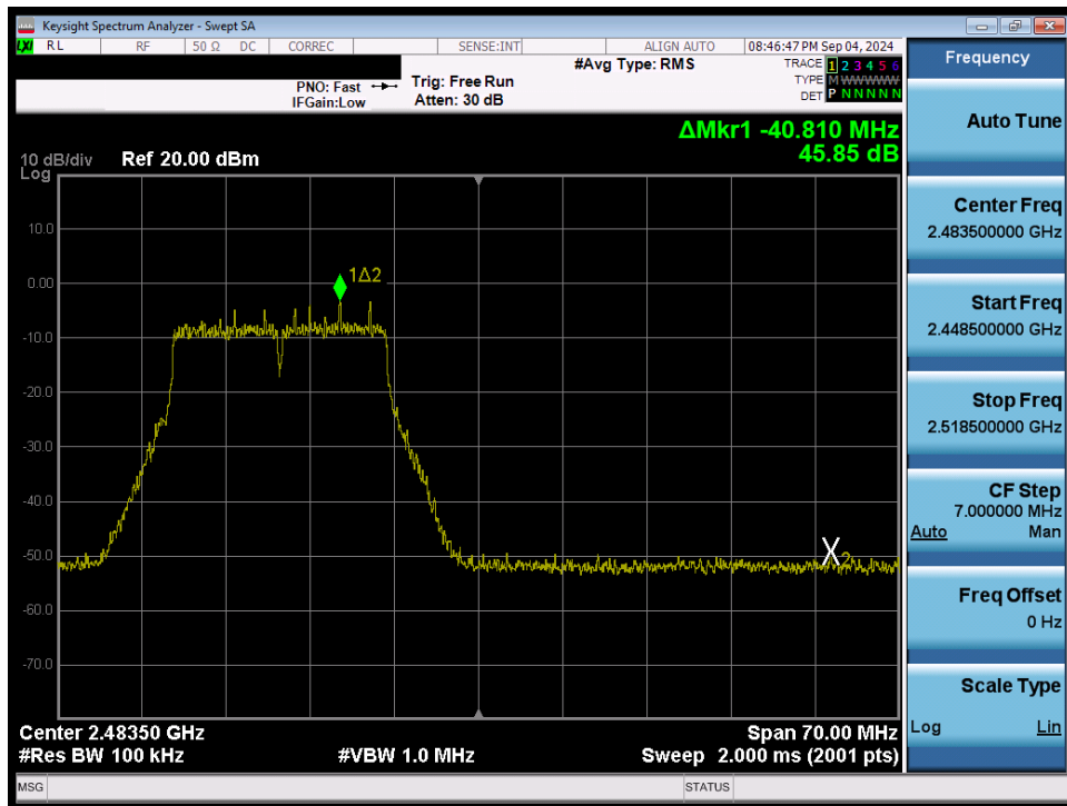
Plot 7-80. Band Edge Plot (802.11n/ac (2.4GHz) - Ch. 12) MIMO ANT2
