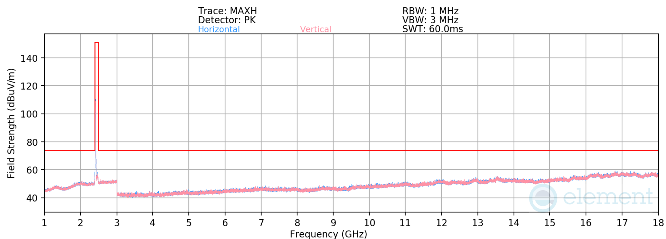
Plot 7-101. Radiated Spurious Plot above 1GHz (802.11n – Ch. 1) MIMO
