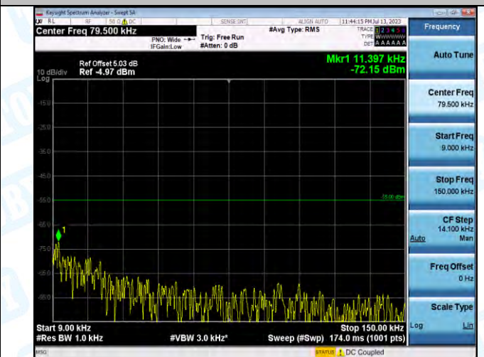
Band7_Band7_10MHz_16QAM_20800_1RB#0_0.009-0.15_0.009-0.15
