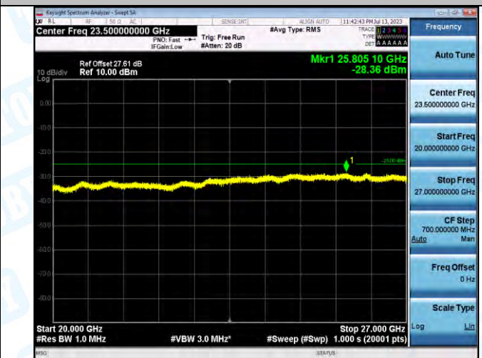
Band7_Band7_5MHz_16QAM_21425_1RB#0_20000~27000_20000~27000
