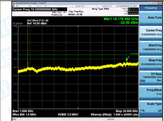
Band7_Band7_10MHz_QPSK_21100_1RB#0_1000~20000_1000~20000
