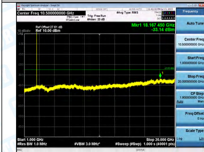
Band7_Band7_5MHz_16QAM_21425_1RB#0_1000~20000_1000~20000
