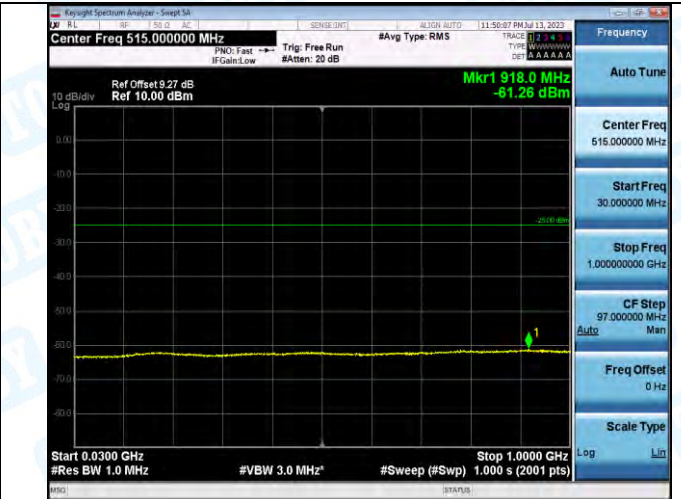
Band7_Band7_15MHz_16QAM_20825_1RB#0_30-1000_30-1000
