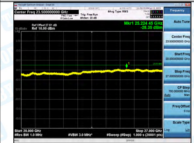
Band7_Band7_15MHz_16QAM_20825_1RB#0_20000~27000_20000~27000
