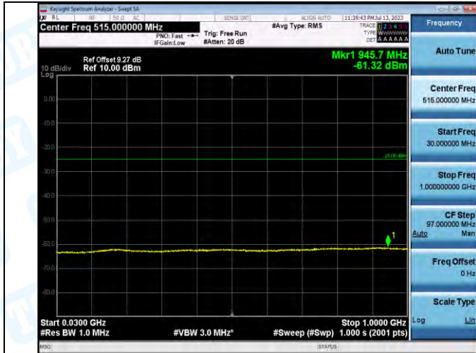
Band7_5MHz_QPSK_21100_1RB#0_30~1000_30~1000
