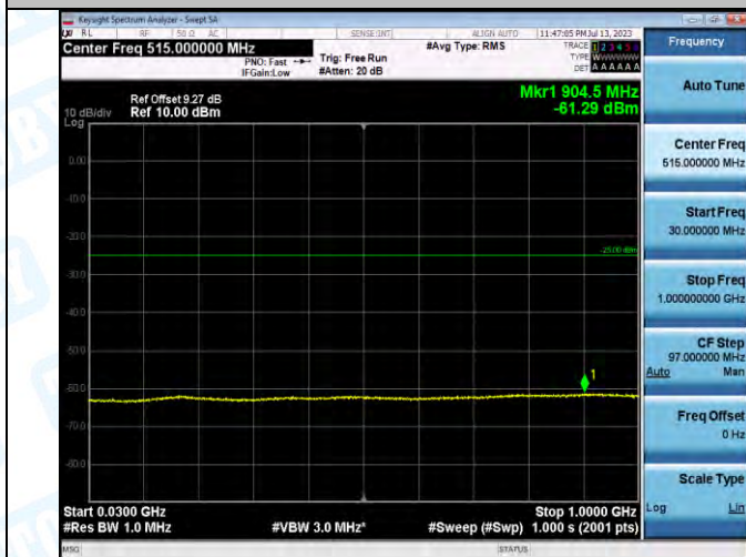
Band7_Band7_10MHz_QPSK_21400_1RB#0_30~1000_30~1000
