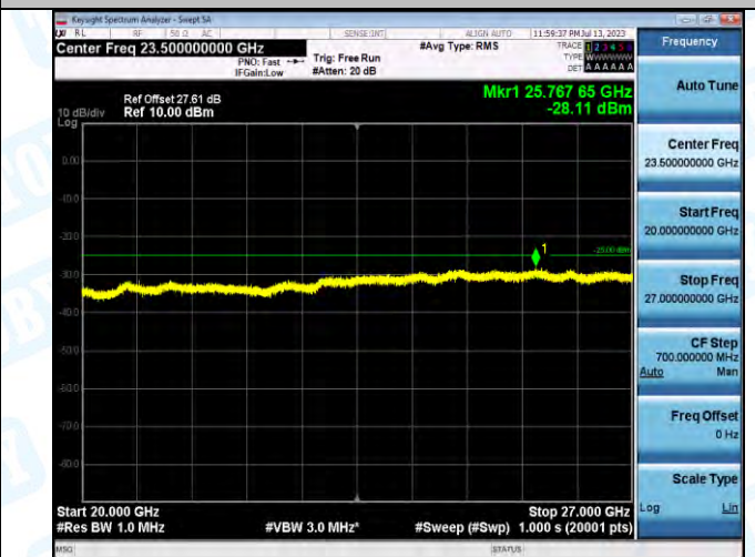
Band7_Band7_20MHz_16QAM_21350_1RB#0_20000~27000_20000~27000
