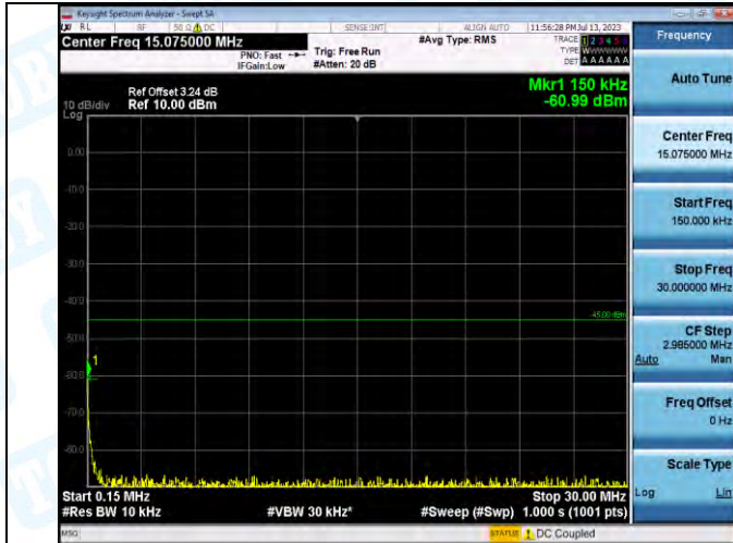
Band7_Band7_20MHz_QPSK_21100_1RB#0_0.15~30.0.15~30
