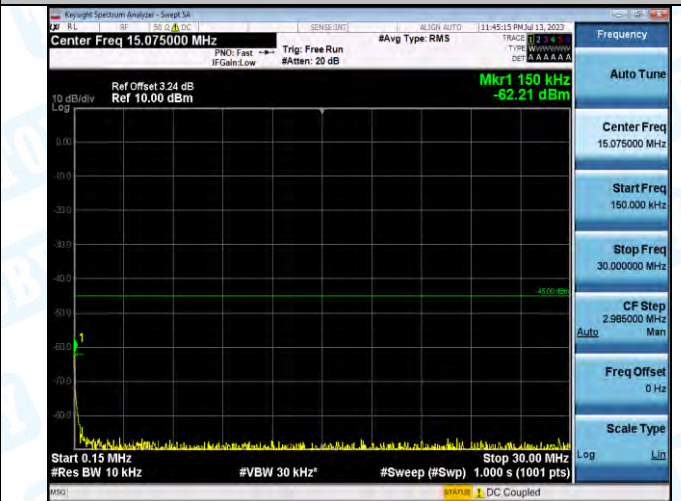
Band7_Band7_10MHz_QPSK_21100_1RB#0_0.15~30.0.15~30
