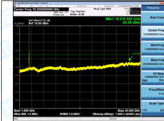
Band7_20MHz_QPSK_20850_1RB#0_1000~20000_1000~20000
