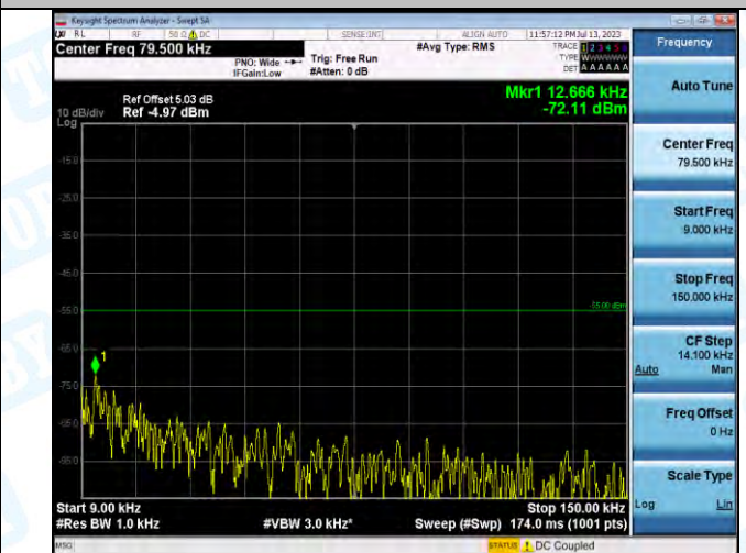
Band7_Band7_20MHz_16QAM_21100_1RB#0_0.009-0.15_0.009-0.15
