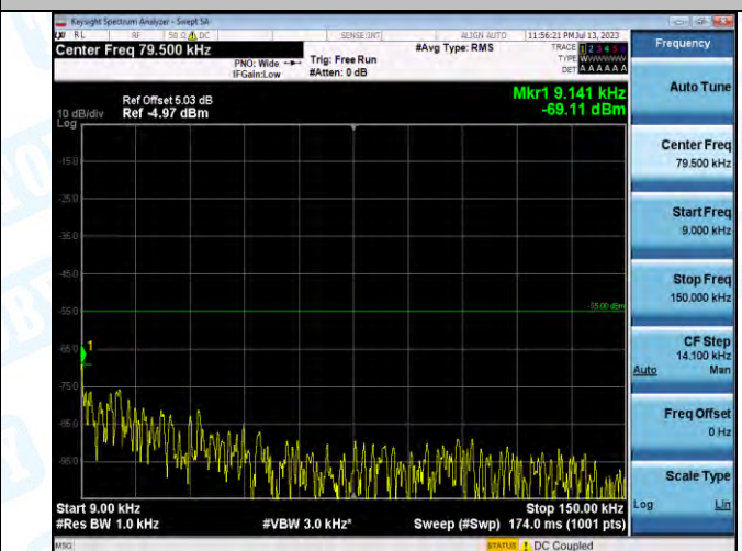
Band7_20MHz_QPSK_21100_1RB#0_0.009~0.15_0.009~0.15
