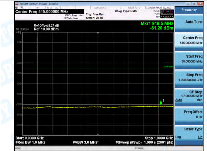
Band7_Band7_15MHz_QPSK_20825_1RB#0_30~1000_30~1000
