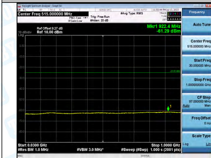
Band7_20MHz_16QAM_20850_1RB#0_30~1000_30~1000
