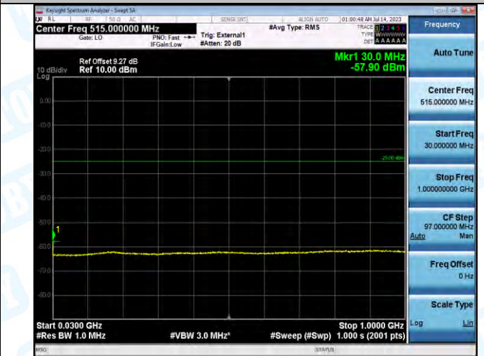
Band41_Band41_5MHz_16QAM_40620_1RB#0_30~1000_30~1000
