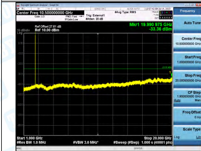
Band41_Band41_5MHz_16QAM_39675_1RB#0_1000-20000_1000-20000
