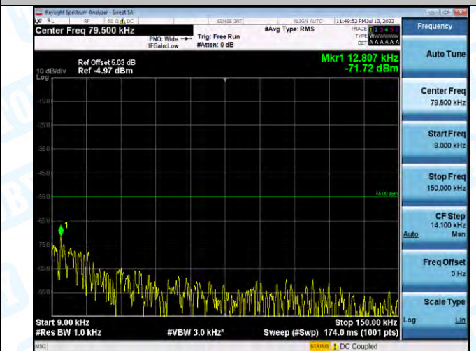
Band7_Band7_15MHz_16QAM_20825_1RB#0_0.009~0.15_0.009~0.15
