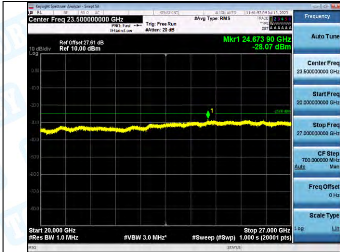
Band7_Band7_5MHz_QPSK_21425_1RB#0_20000~27000_20000~27000
