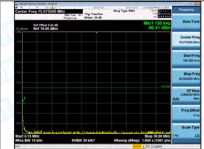
Band7_Band7_10MHz_QPSK_20800_1RB#0_0.15-30_0.15-30
