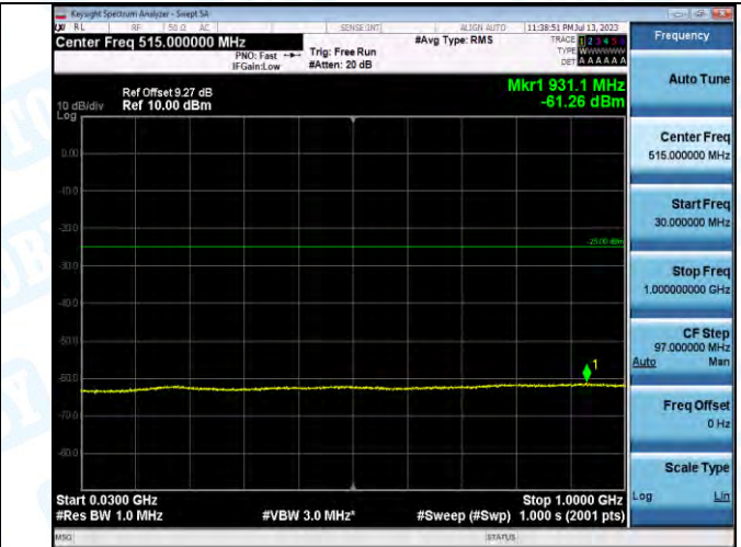
Band7_5MHz_16QAM_20775_1RB#0_30-1000_30-1000
