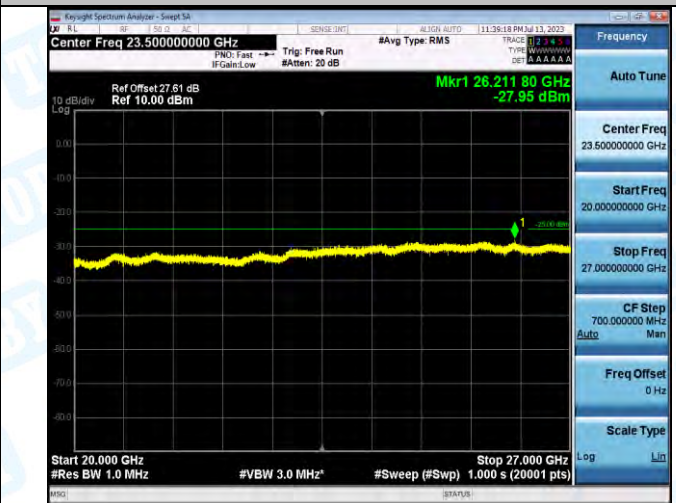
Band7_5MHz_16QAM_20775_1RB#0_20000-27000_20000-27000
