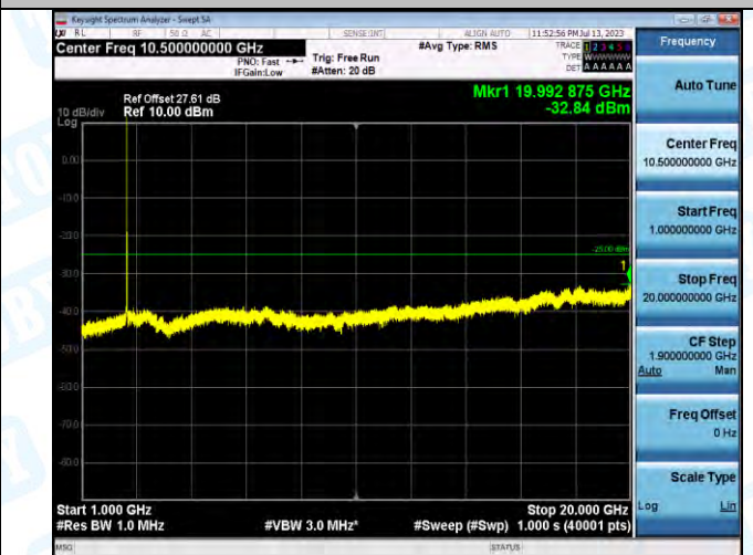
Band7_Band7_15MHz_QPSK_21375_1RB#0_1000-20000_1000-20000
