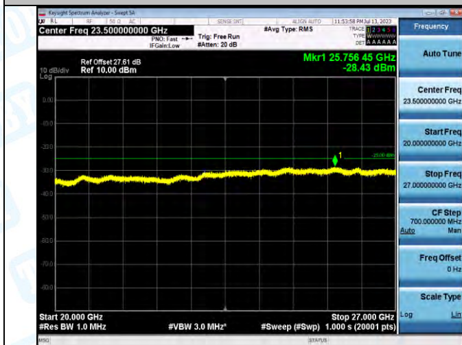
Band7_Band7_15MHz_16QAM_21375_1RB#0_20000~27000_20000~27000
