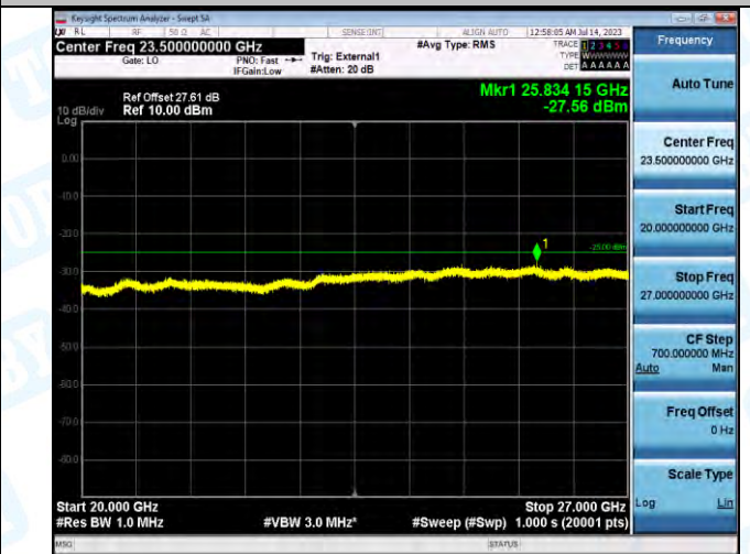
Band41_Band41_5MHz_16QAM_39675_1RB#0_20000-27000_20000-27000
