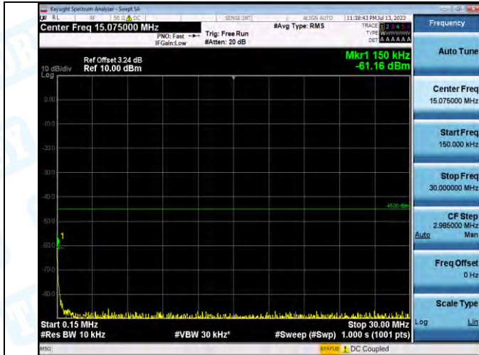
Band7_5MHz_16QAM_20775_1RB#0_0.15-0.15-30
