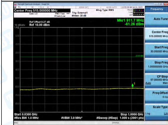
Band41_Band41_5MHz_QPSK_39675_1RB#0_30~1000_30~1000
