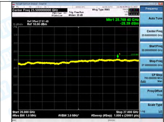
Band7_Band7_10MHz_16QAM_21100_1RB#0_20000~27000_20000~27000
