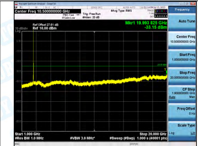
Band7_Band7_15MHz_QPSK_21100_1RB#0_1000~20000_1000~20000
