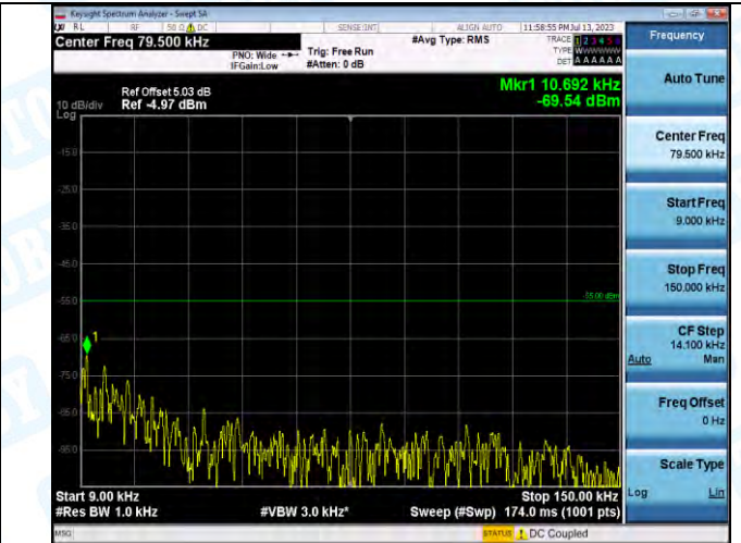
Band7_Band7_20MHz_16QAM_21350_1RB#0_0.009~0.15_0.009~0.15
