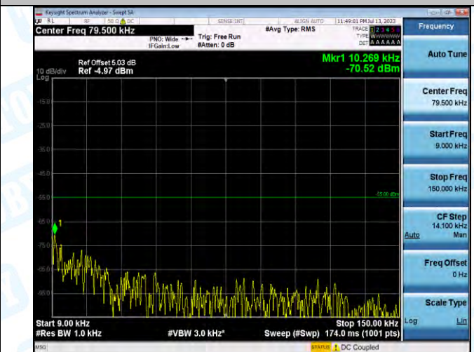
Band7_Band7_15MHz_QPSK_20825_1RB#0_0.009~0.15_0.009~0.15
