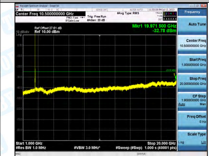
Band7_20MHz_16QAM_20850_1RB#0_1000~20000_1000~20000
