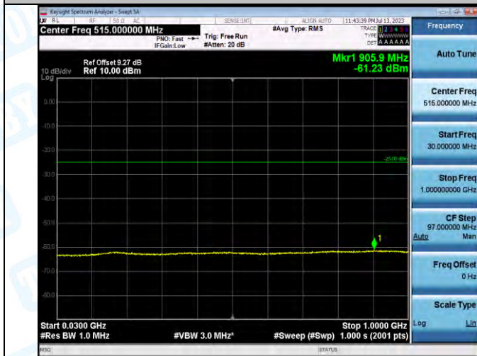
Band7_Band7_10MHz_QPSK_20800_1RB#0_30-1000_30-1000
