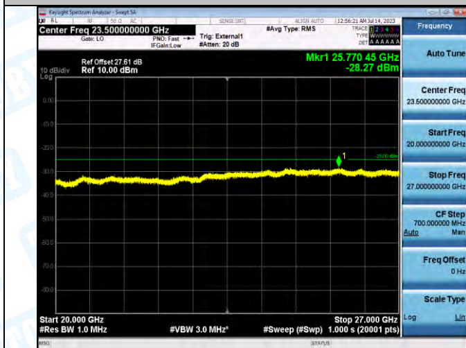
Band41_Band41_5MHz_QPSK_39675_1RB#0_20000~27000_20000~27000
