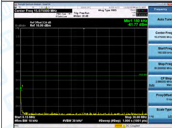
Band7_Band7_15MHz_QPSK_21375_1RB#0_0.15~30_0.15~30
