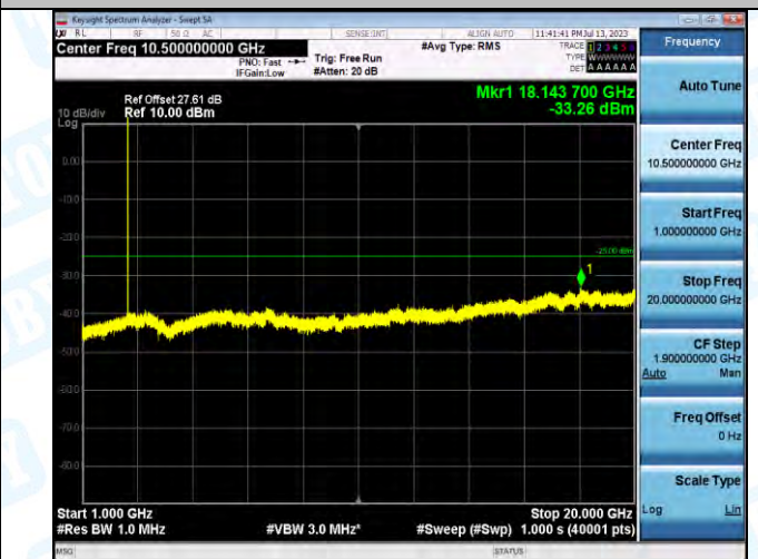
Band7_Band7_5MHz_QPSK_21425_1RB#0_1000~20000_1000~20000
