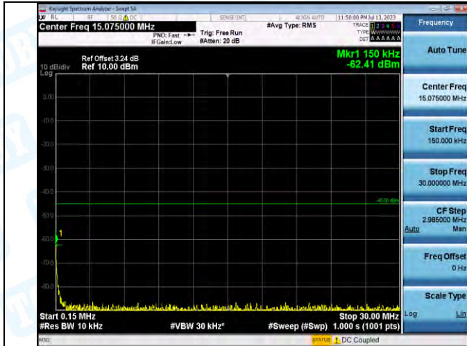
Band7_Band7_15MHz_16QAM_20825_1RB#0_0.15-30.0_15-30
