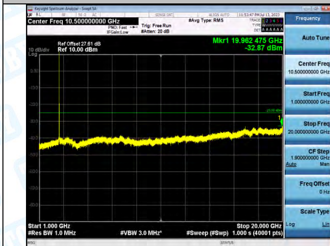
Band7_Band7_15MHz_16QAM_21375_1RB#0_1000~20000_1000~20000
