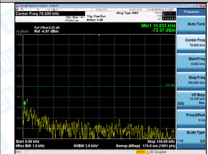
Band7_Band7_10MHz_16QAM_21100_1RB#0_0.009~0.15_0.009~0.15
