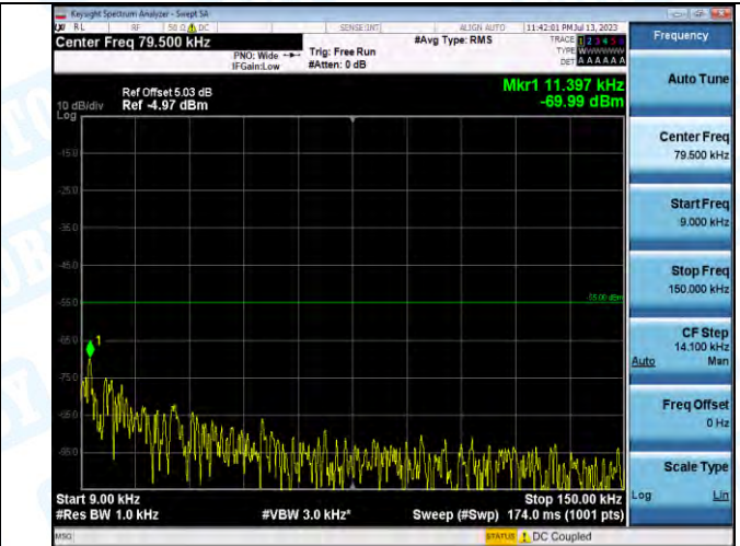
Band7_Band7_5MHz_16QAM_21425_1RB#0_0.009~0.15_0.009~0.15
