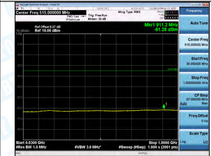
Band7_Band7_20MHz_QPSK_21350_1RB#0_30~1000.30~1000
