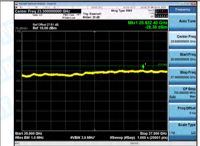
Band41_Band41_5MHz_16QAM_40620_1RB#0_20000~27000_20000~27000
