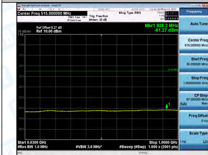
Band7_Band7_5MHz_QPSK_21425_1RB#0_30~1000_30~1000
