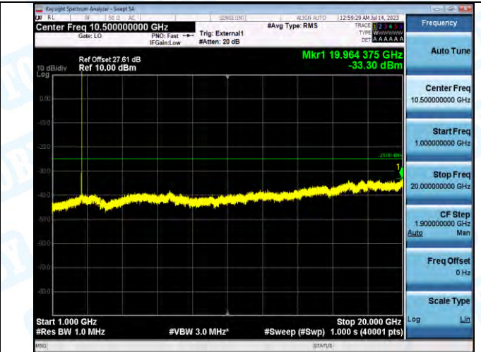
Band41_Band41_5MHz_QPSK_40620_1RB#0_1000~20000_1000~20000
