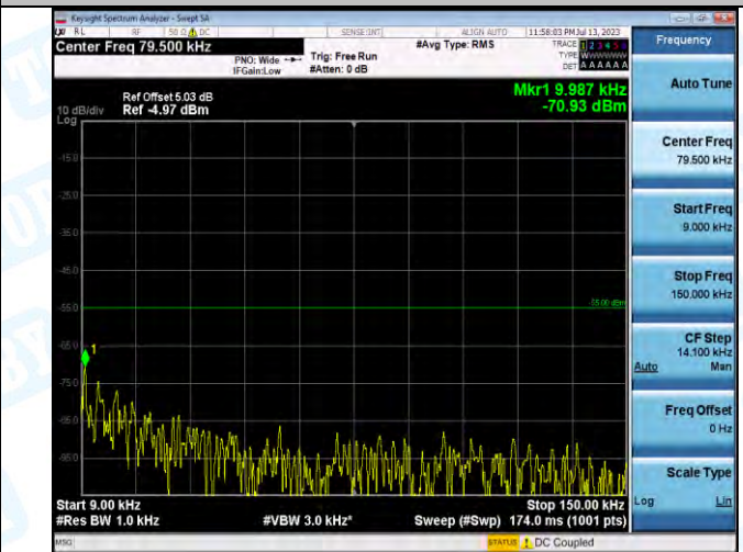
Band7_Band7_20MHz_QPSK_21350_1RB#0_0.009~0.15.0.009~0.15
