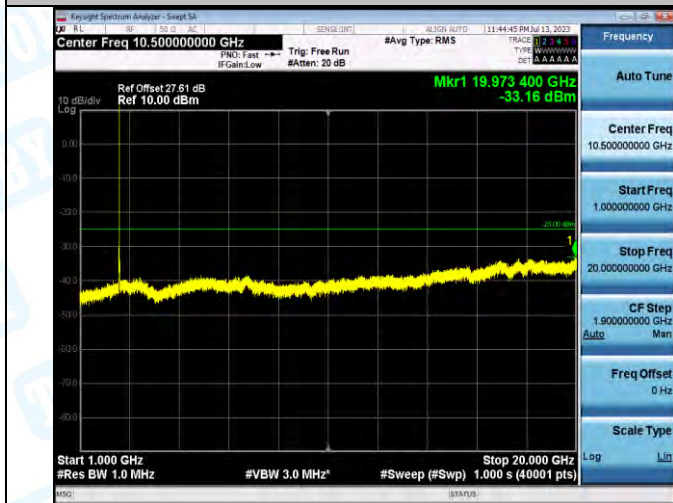
Band7_Band7_10MHz_16QAM_20800_1RB#0_1000~20000.1000~20000
