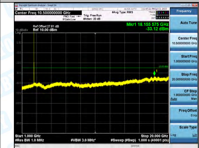
Band7_Band7_10MHz_QPSK_21400_1RB#0_1000~20000_1000~20000
