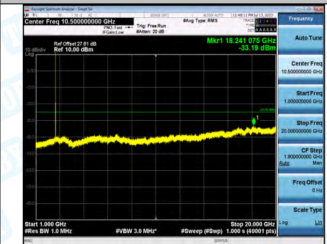
Band7_Band7_10MHz_16QAM_21400_1RB#0_1000~20000_1000~20000
