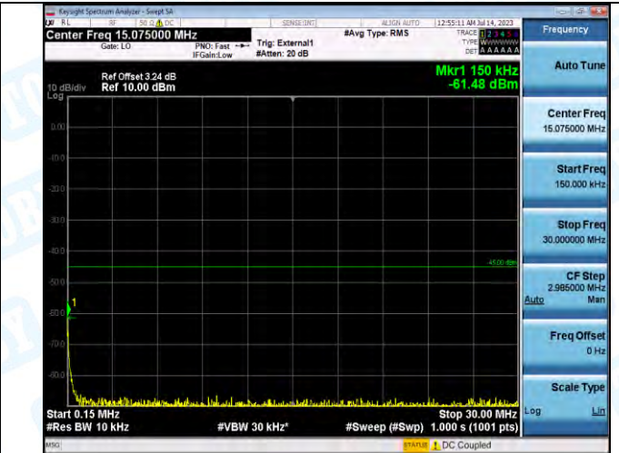
Band41_Band41_5MHz_QPSK_39675_1RB#0_0.15~30_0.15~30
