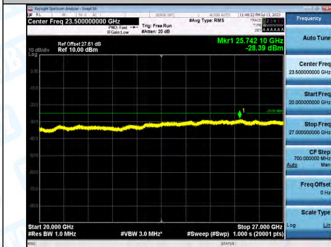
Band7_Band7_10MHz_16QAM_21400_1RB#0_20000~27000_20000~27000
