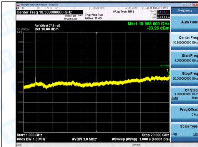
Band7_Band7_10MHz_16QAM_21100_1RB#0_1000~20000_1000~20000
