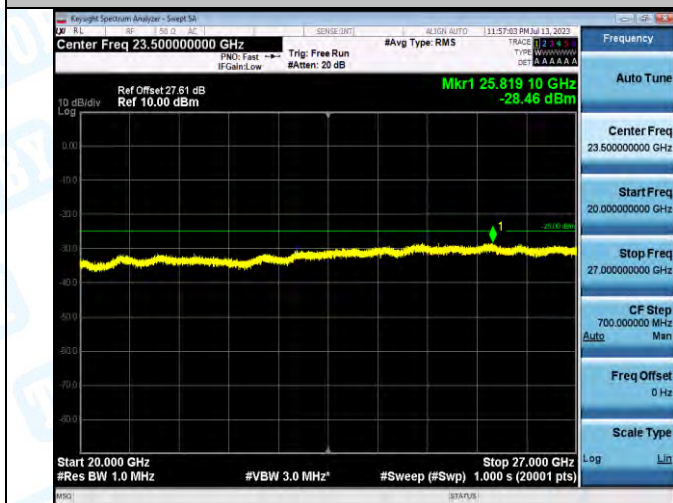
Band7_Band7_20MHz_QPSK_21100_1RB#0_20000-27000_20000-27000
