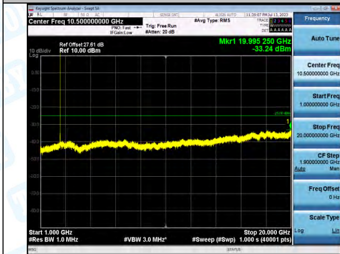
Band7_5MHz_16QAM_20775_1RB#0_1000-20000_1000-20000
