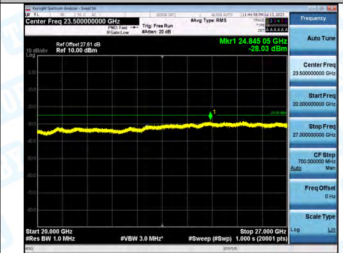
Band7_Band7_10MHz_16QAM_20800_1RB#0_20000~27000.20000~27000
