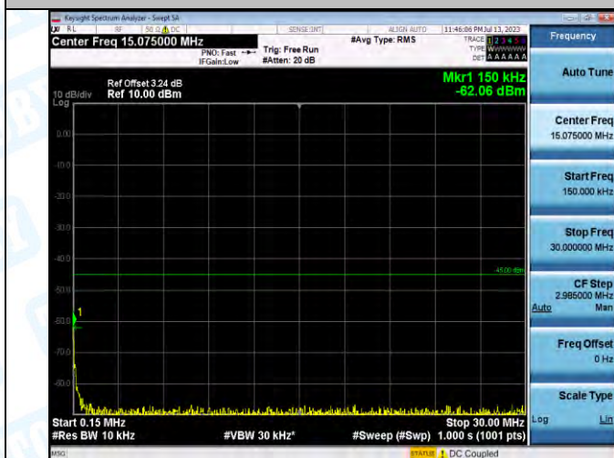
Band7_Band7_10MHz_16QAM_21100_1RB#0_0.15~30_0.15~30
