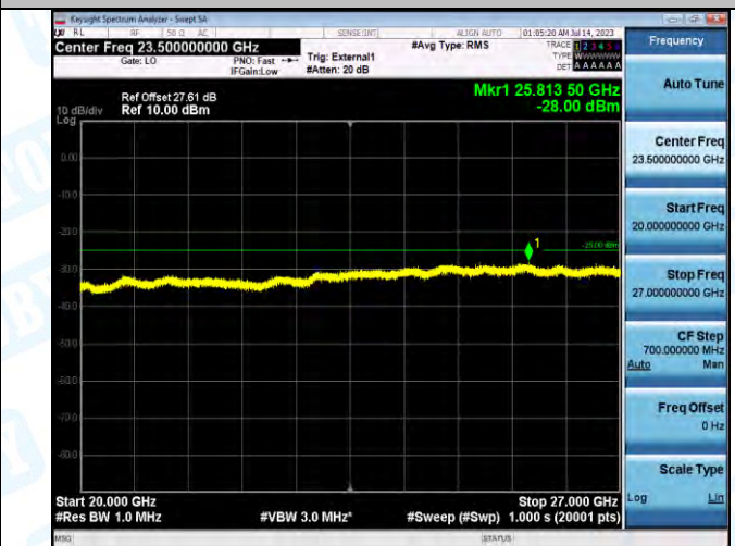
Band41_Band41_5MHz_16QAM_41565_1RB#0_20000~27000_20000~27000
