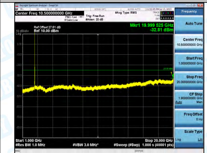
Band7_Band7_15MHz_16QAM_21100_1RB#0_1000~20000_1000~20000
