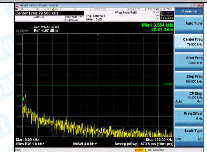
Band41_Band41_5MHz_16QAM_39675_1RB#0_0.009~0.15_0.009~0.15
