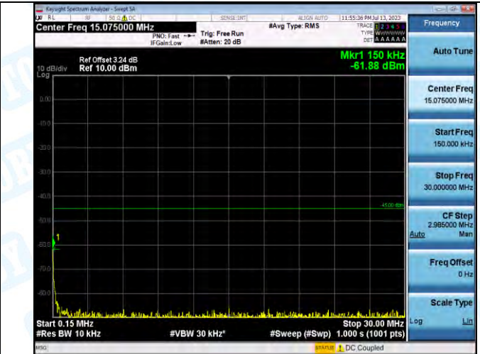
Band7_20MHz_16QAM_20850_1RB#0_0.15~30.0_0.15~30.0
