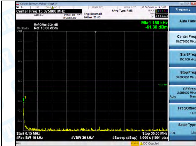
Band41_Band41_5MHz_16QAM_39675_1RB#0_0.15-30_0.15-30
