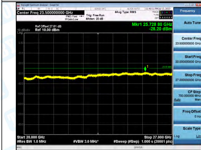
Band7_5MHz_QPSK_21100_1RB#0_20000~27000_20000~27000
