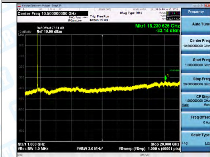
Band7_Band7_20MHz_16QAM_21350_1RB#0_1000~20000_1000~20000
