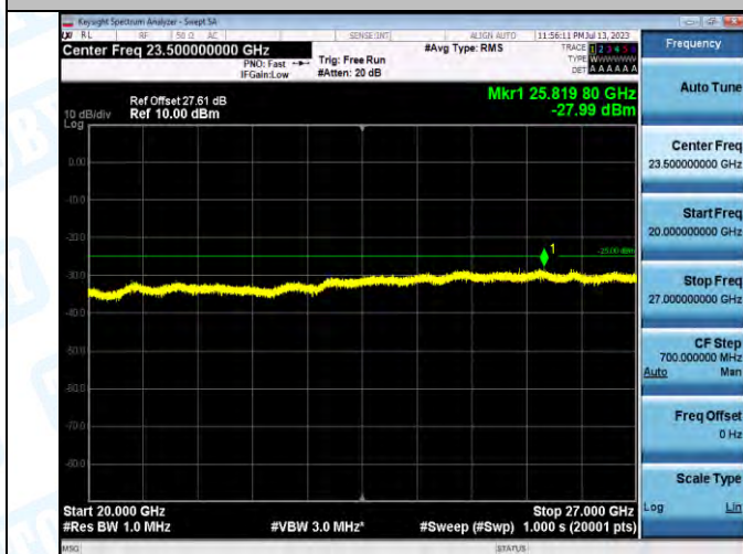
Band7_20MHz_16QAM_20850_1RB#0_20000~27000_20000~27000
