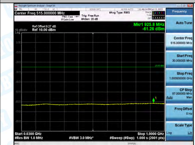
Band7_Band7_10MHz_16QAM_21100_1RB#0_30~1000_30~1000
