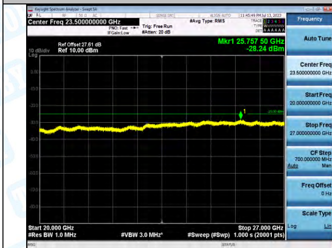
Band7_Band7_10MHz_QPSK_21100_1RB#0_20000~27000_20000~27000
