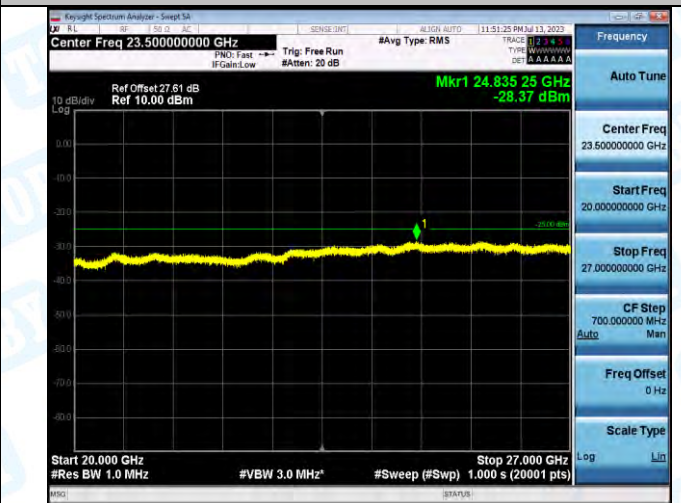
Band7_Band7_15MHz_QPSK_21100_1RB#0_20000-27000_20000-27000
