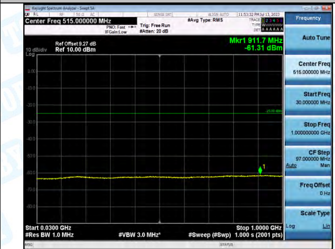
Band7_Band7_15MHz_16QAM_21375_1RB#0_30~1000_30~1000
