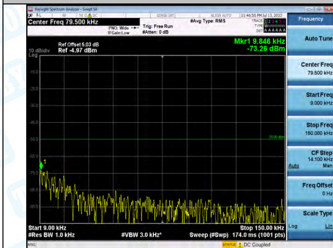
Band7_Band7_10MHz_QPSK_21400_1RB#0_0.009~0.15_0.009~0.15
