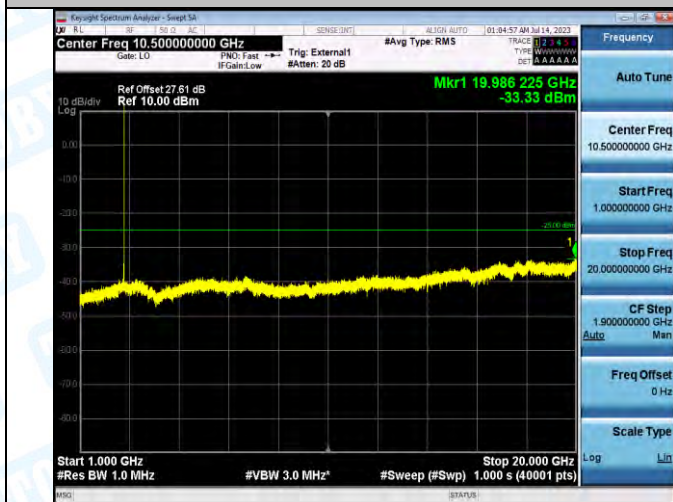
Band41_Band41_5MHz_16QAM_41565_1RB#0_1000~20000_1000~20000
