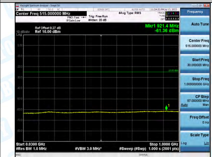
Band7_Band7_20MHz_QPSK_20850_1RB#0_30~1000_30~1000
