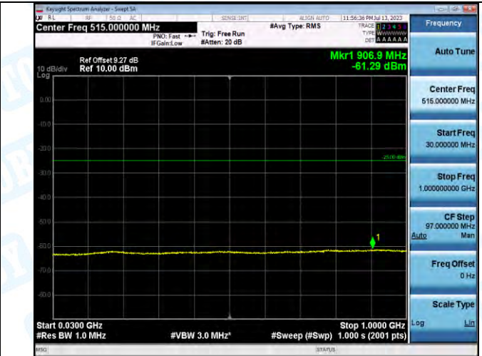
Band7_Band7_20MHz_QPSK_21100_1RB#0_30~1000.30~1000
