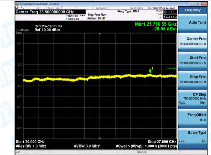
Band7_Band7_5MHz_16QAM_21100_1RB#0_20000~27000_20000~27000
