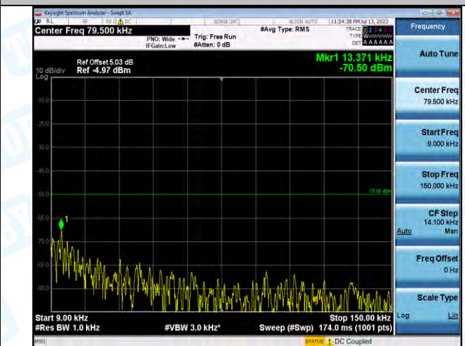
Band7_Band7_20MHz_QPSK_20850_1RB#0_0.009~0.15_0.009~0.15
