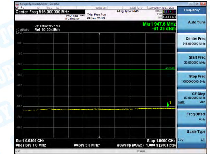
Band7_Band7_10MHz_16QAM_20800_1RB#0_30~1000.30~1000
