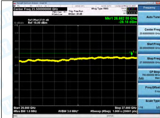
Band7_Band7_15MHz_16QAM_21100_1RB#0_20000~27000_20000~27000
