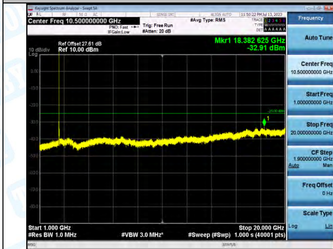
Band7_Band7_15MHz_16QAM_20825_1RB#0_1000-20000_1000-20000
