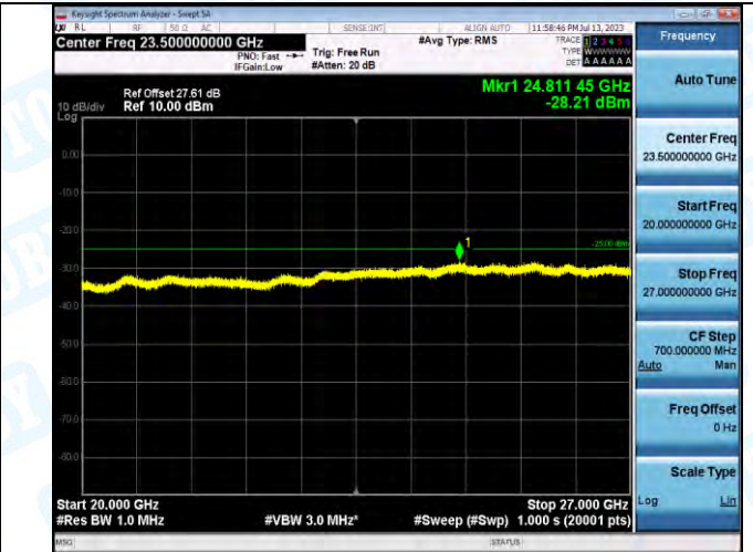
Band7_Band7_20MHz_QPSK_21350_1RB#0_20000~27000_20000~27000
