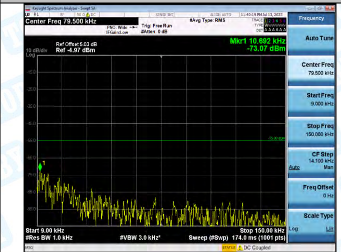
Band7_5MHz_16QAM_21100_1RB#0_0.009~0.15_0.009~0.15
