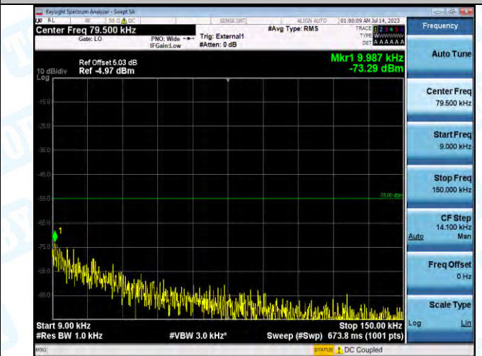
Band41_Band41_5MHz_16QAM_40620_1RB#0_0.009~0.15_0.009~0.15
