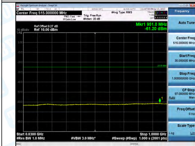
Band7_Band7_10MHz_16QAM_21400_1RB#0_30~1000_30~1000
