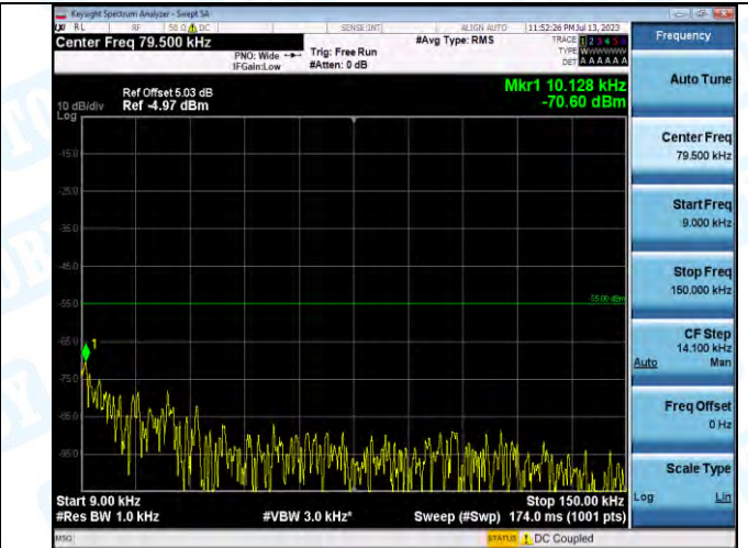
Band7_Band7_15MHz_QPSK_21375_1RB#0_0.009~0.15_0.009~0.15
