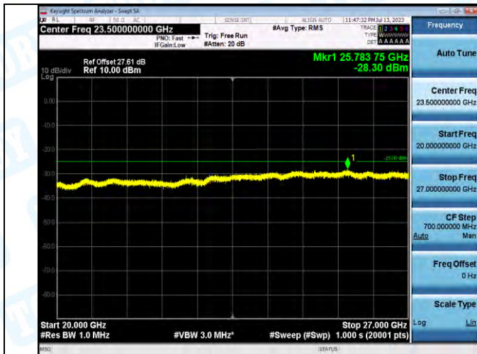
Band7_Band7_10MHz_QPSK_21400_1RB#0_20000~27000_20000~27000
