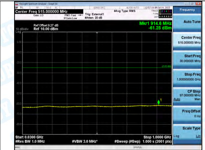
Band41_Band41_5MHz_16QAM_39675_1RB#0_30-1000_30-1000
