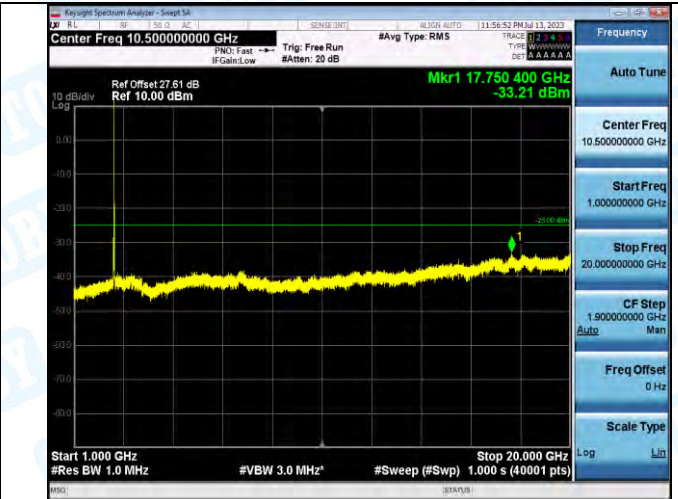
Band7_Band7_20MHz_QPSK_21100_1RB#0_1000-20000_1000-20000
