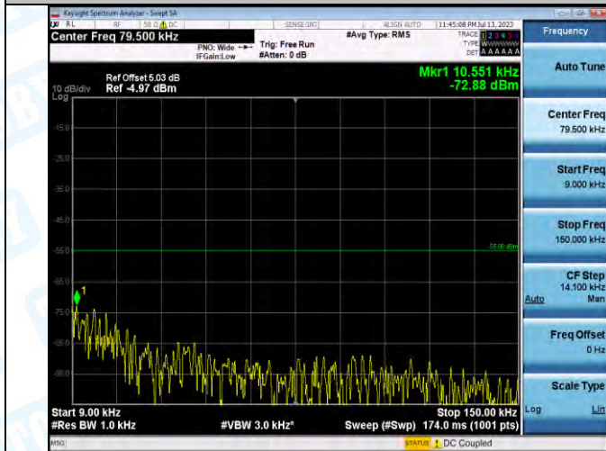
Band7_Band7_10MHz_QPSK_21100_1RB#0_0.009~0.15.0.009~0.15
