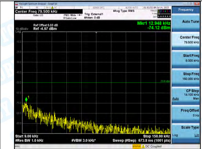
Band41_Band41_5MHz_16QAM_41565_1RB#0_0.009~0.15_0.009~0.15
