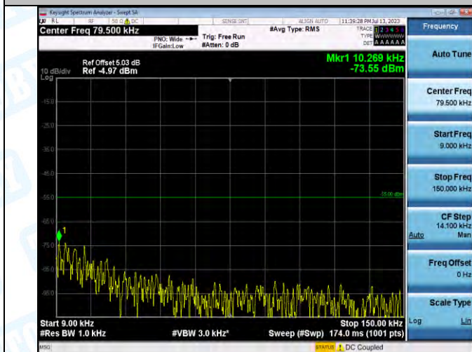
Band7_5MHz_QPSK_21100_1RB#0_0.009-0.15_0.009-0.15
