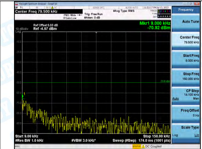
Band7_Band7_15MHz_16QAM_21375_1RB#0_0.009~0.15_0.009~0.15
