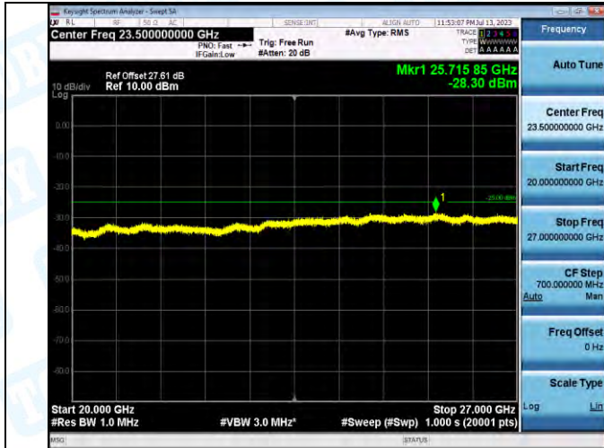
Band7_Band7_15MHz_QPSK_21375_1RB#0_20000~27000_20000~27000
