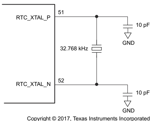
Figure 8-9. RTC Crystal Connections
