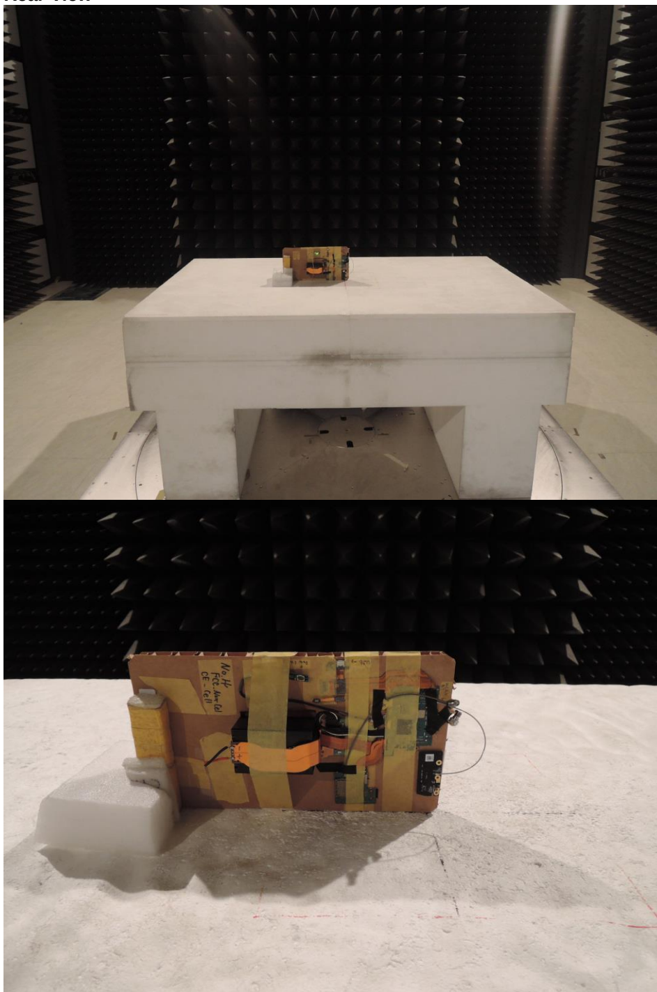
Rear View
