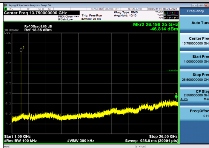
BLE_1M_Ant1_2480_0~Reference
