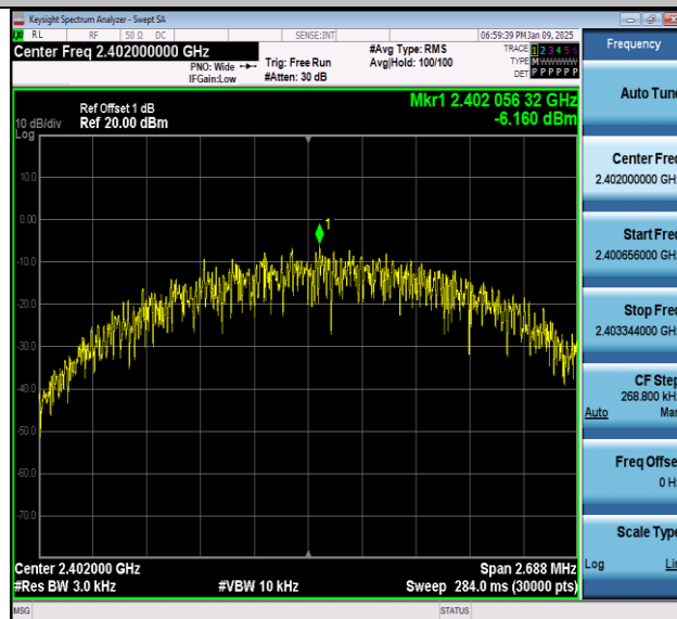
BLE_2M-Ant1-2402-PASS
