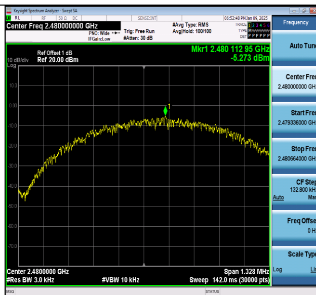
BLE_1M-Ant1-2480-PASS
