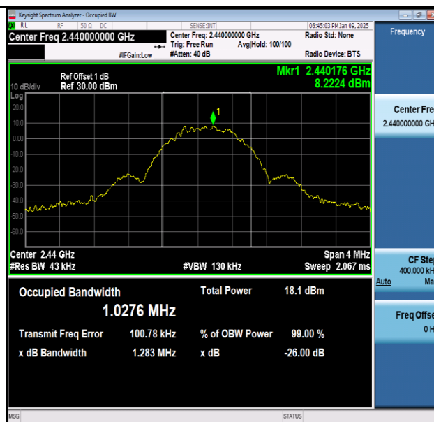
BLE_1M-Ant1-2440
