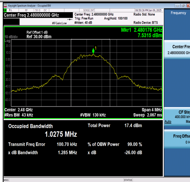
BLE_1M-Ant1-2480
