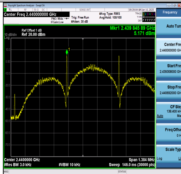
BLE_125K-Ant1-2440-PASS
