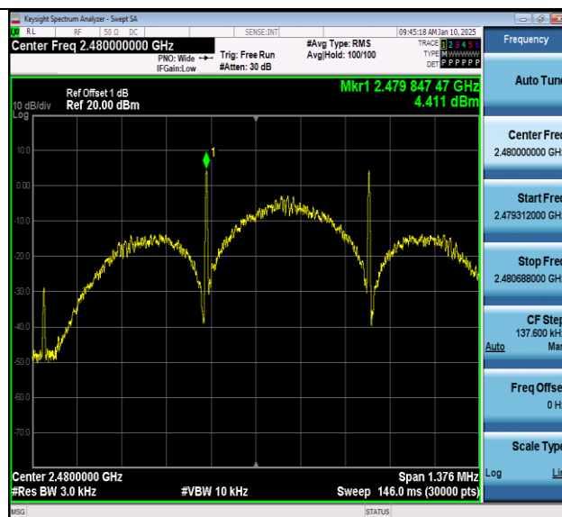
BLE_125K-Ant1-2480-PASS
