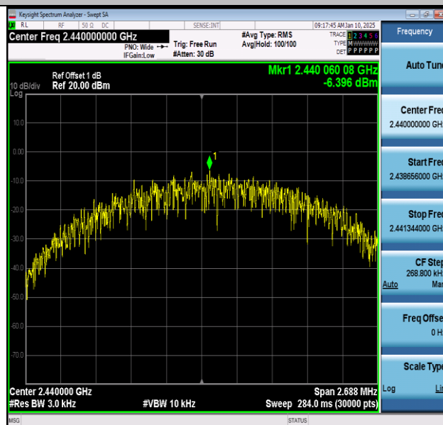
BLE_2M-Ant1-2440-PASS
