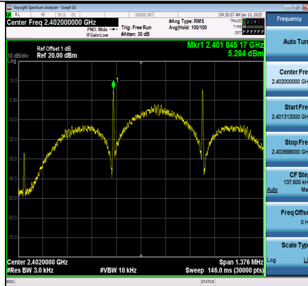
BLE_125K-Ant1-2402-PASS
