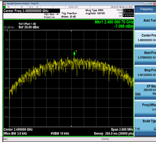
BLE_2M-Ant1-2480-PASS
