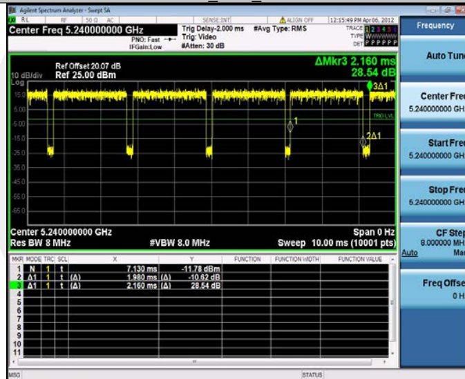
11A_Ant4_5240
