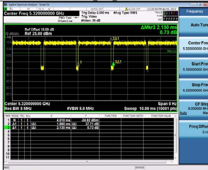
11A_Ant4_5320
