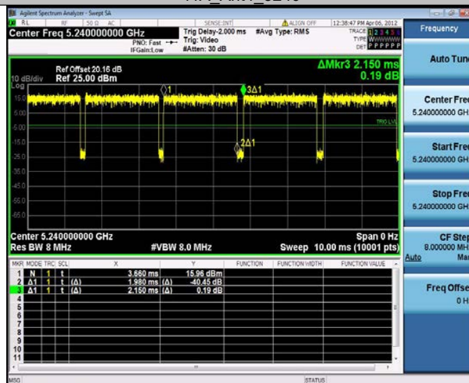
11A_Ant4_5240
