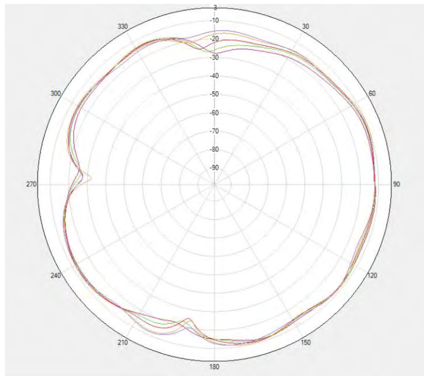
END C Flip LTE3/B4/B66 PRX \Phi = 0^\circ
