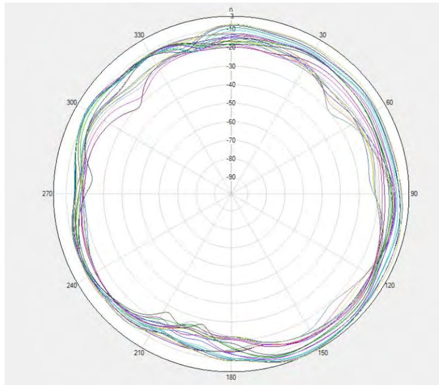
ENDC Flip LTEB1/B7/B38/40/41 PRX \Phi=0^\circ
