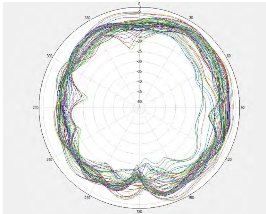
Flip- N77/N78 PRX \Phi = 0^\circ
