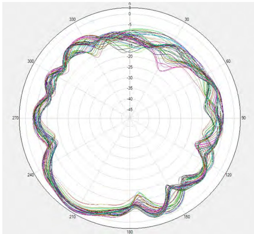
Unflip- N77/N78 DRX1 \Phi=90^\circ
