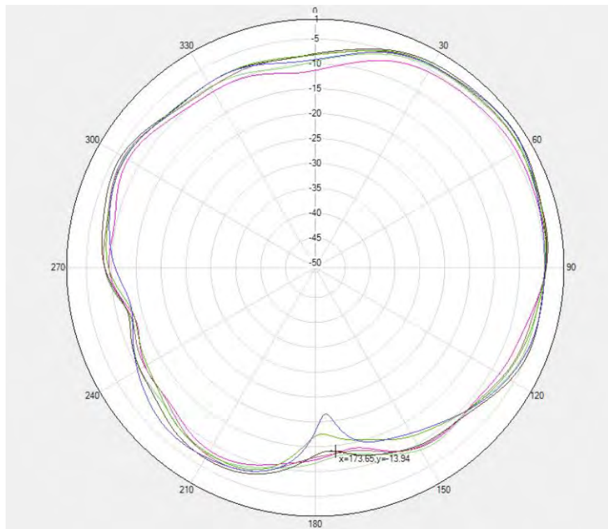
Flip-LTE B40&N40 PRX \Phi=90^\circ
