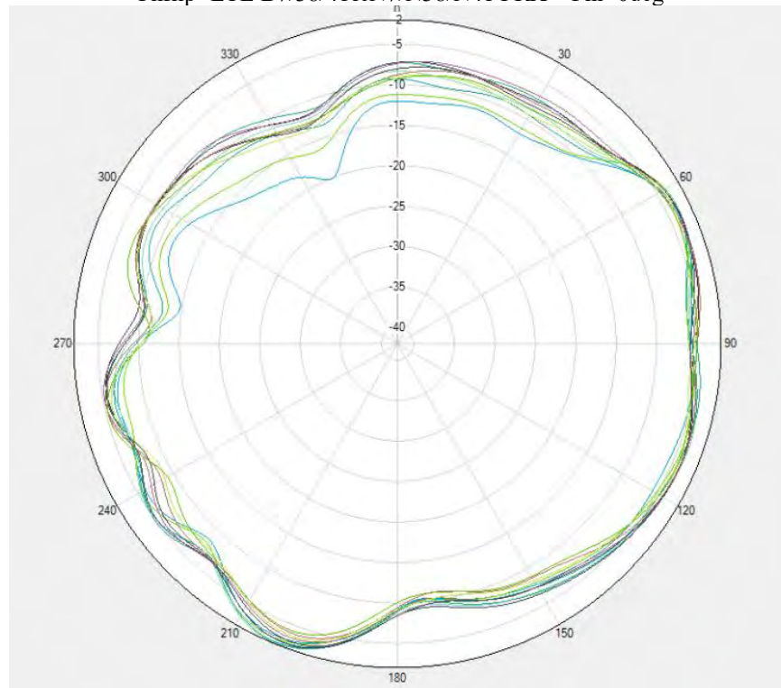
Unflip-LTE B7/38/41&N7/N38/N41 PRX Phi=90deg
