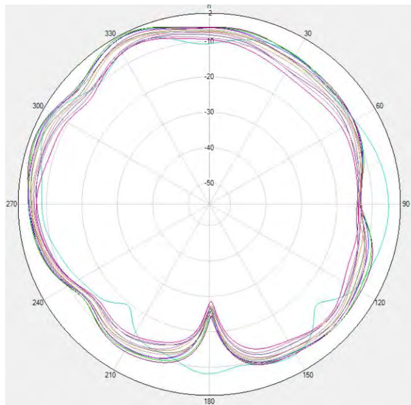
Flip-GPS L1/2.4G WIFI MIMO1 Phi=0deg
