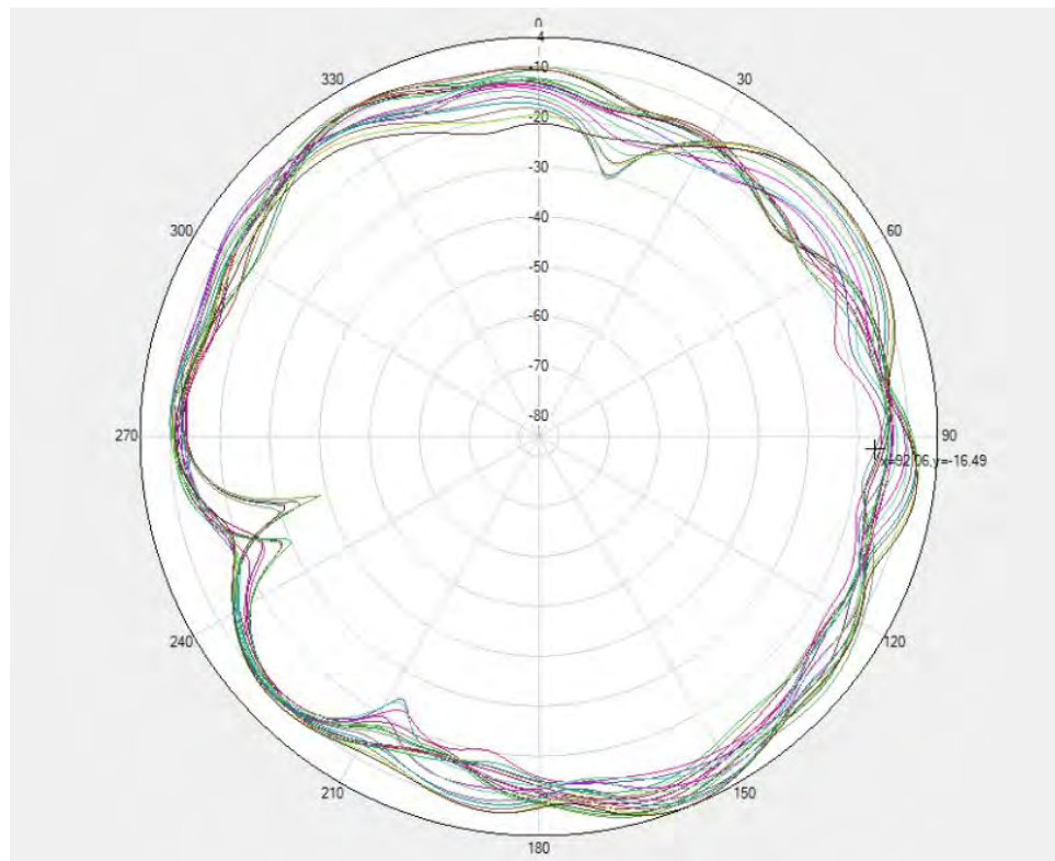
ENDC Unflip LTEB1/B7/B38/40/41 PRX \Phi=0^\circ
