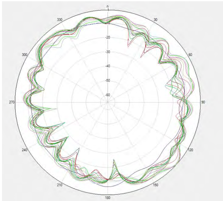
Unflip-GPS L5/5G WIFI MIMO1 \Phi=90^\circ
