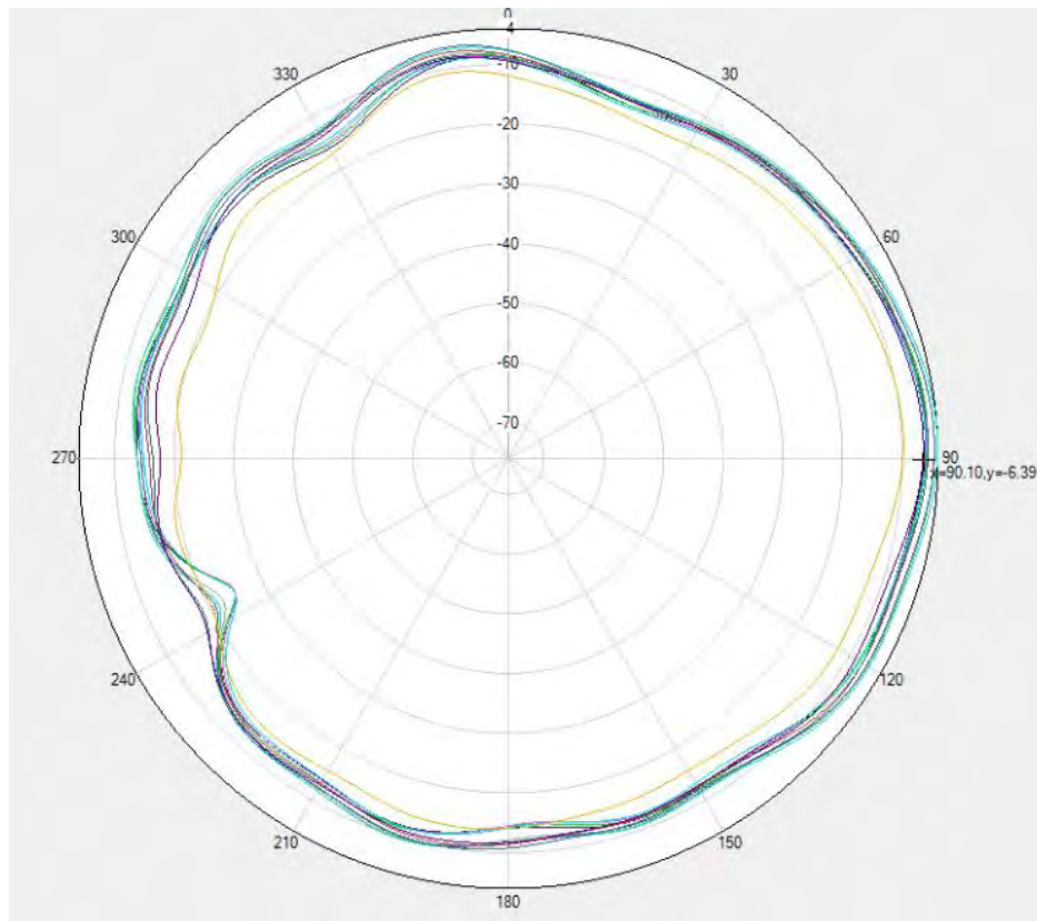
Unflip- LTE B28&N28 \Phi=0^\circ
