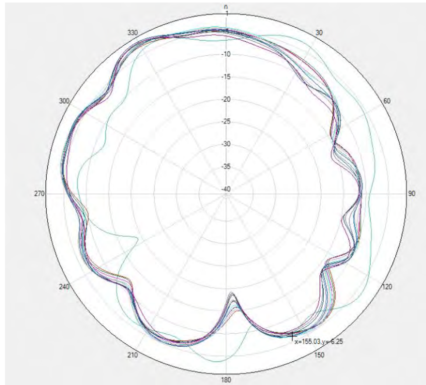
Unflip-GPS L1/2.4G WIFI MIMO1 \Phi=0^\circ
