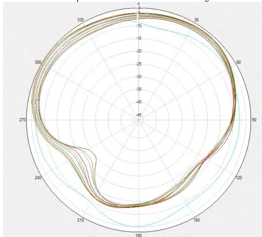
Flip-GPS L1/2.4G WIFI MIMO1 \Theta=90^\circ
