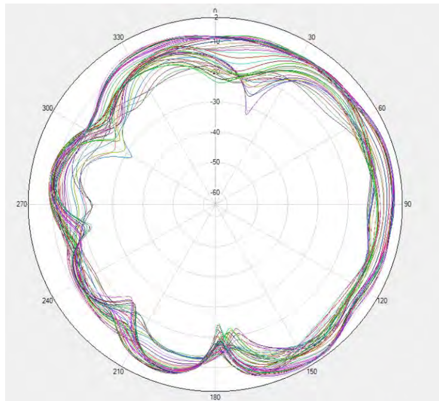
Flip- N77/N78 DRX1 \Phi = 0^\circ
