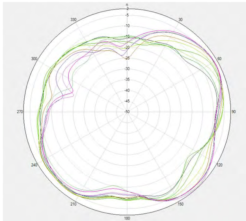
Flip- LTEB38/41&N38/N41 DRX \Phi=90\text{deg}
