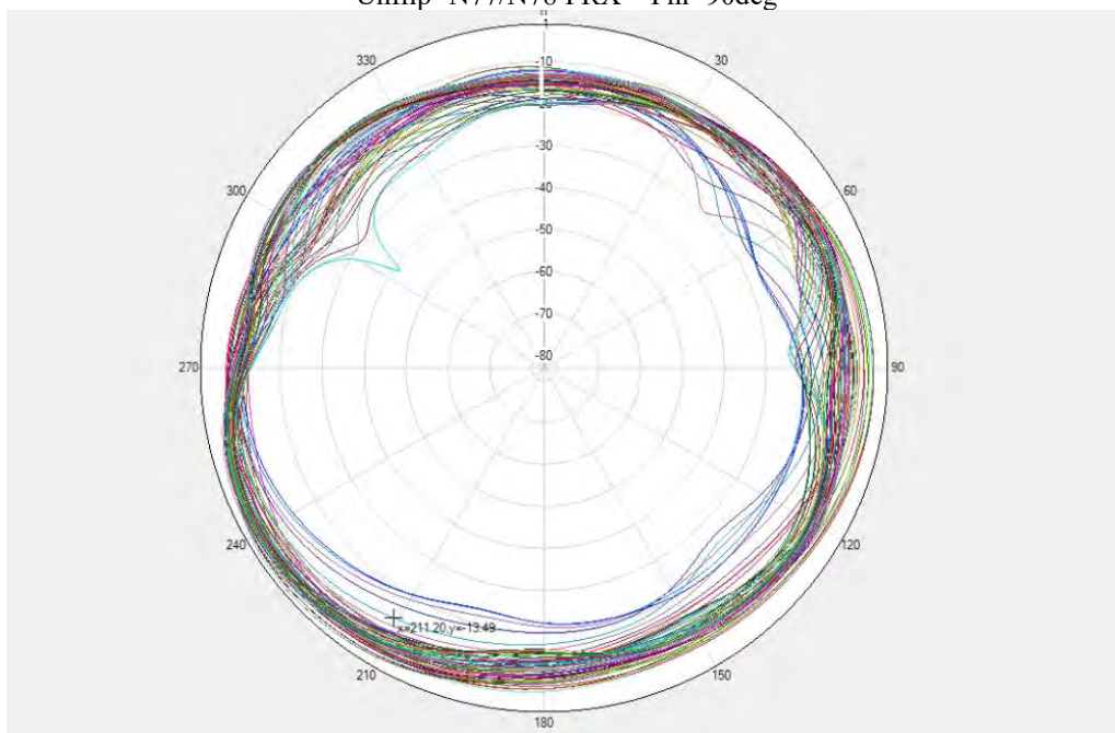
Flip- N77/N78 PRX \Theta=90\text{deg}
