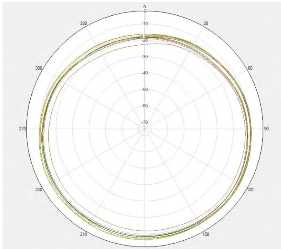
ENDC Unflip LTEB28& N28 PRX Theta=90deg
