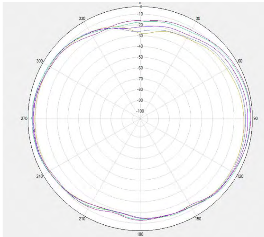
ENDC Unflip LTEB3/B4/B66 PRX \Phi=90\text{deg}
