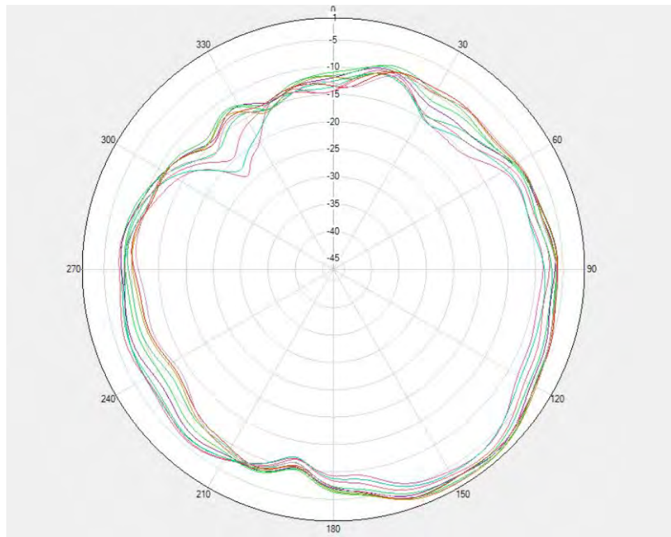
Unflip- LTEB38/41&N38/N41 DRX \Phi=0^\circ
