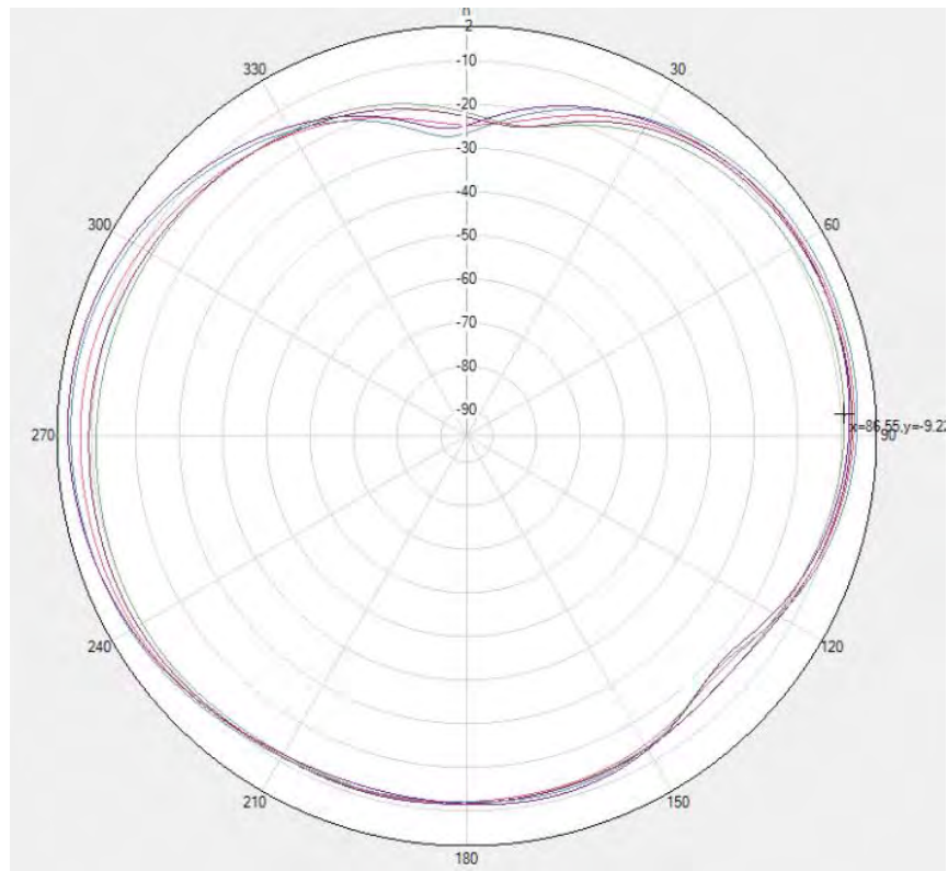
Flip- PCS&WCDMA B2&LTE B2 PRX Theta=90deg
