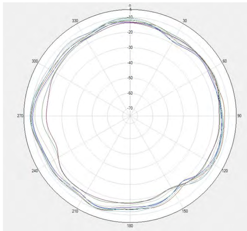
END C Flip LTE B20&NR N20 PRX \Phi = 90^\circ
