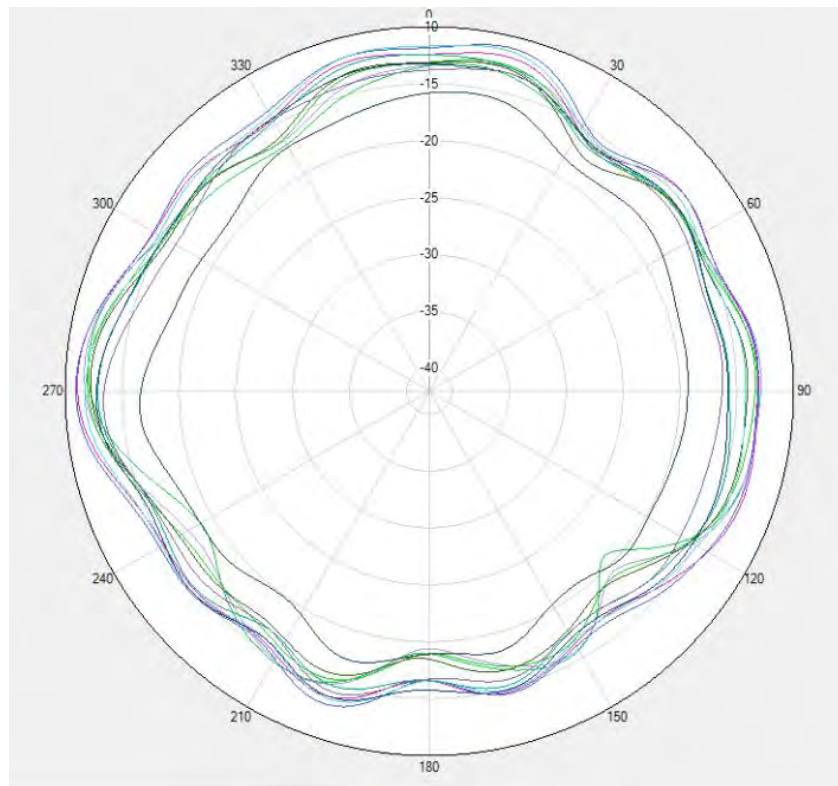
Flip- LTE B28&N28 \Phi=90^\circ
