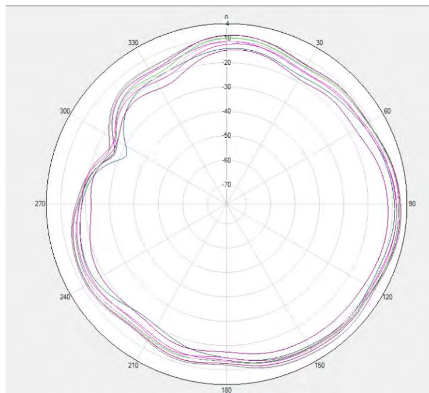
ENDC Unflip LTEB28& N28 PRX Phi=0deg
