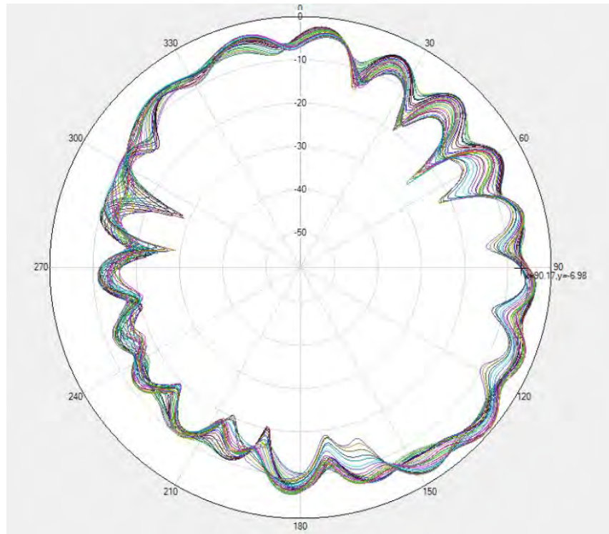
LDS Unflip&Flip- 5G WIFI MIMO2 \Phi = 90^\circ
