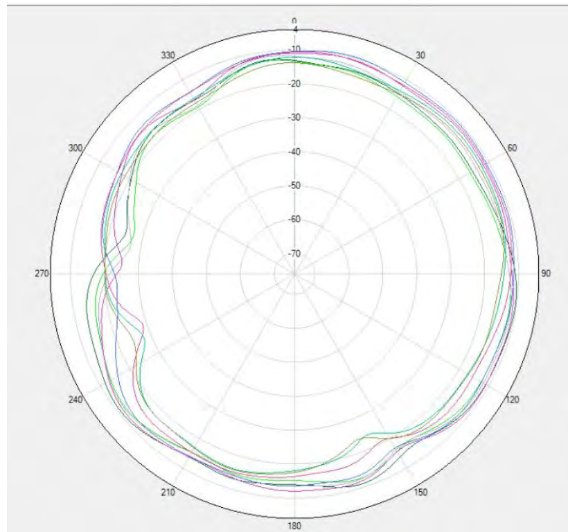
END C Flip LTE B20&NR N20 PRX \Phi = 0^\circ
