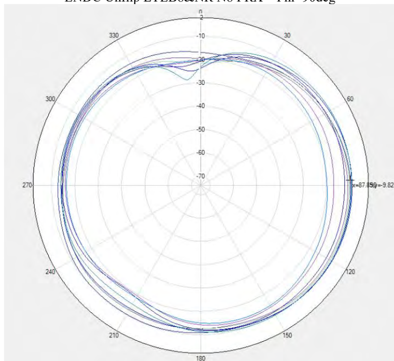
ENDC Unflip LTEB20& N20 PRX \Theta=90\text{deg}
