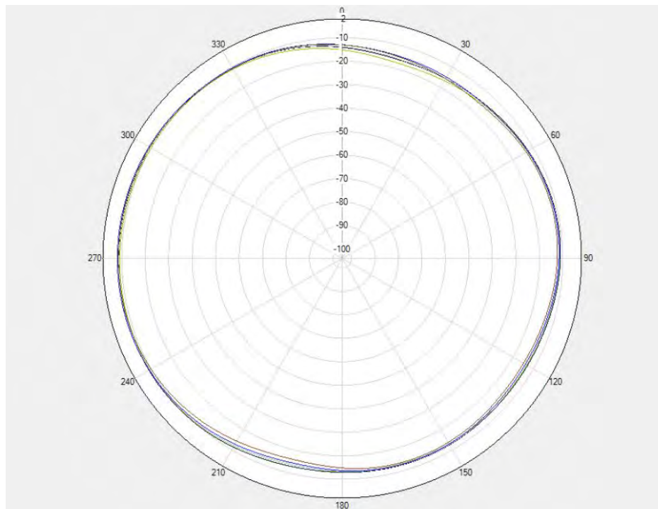
ENDC Unflip LTEB3/B4/B66 PRX \Theta=90^\circ
