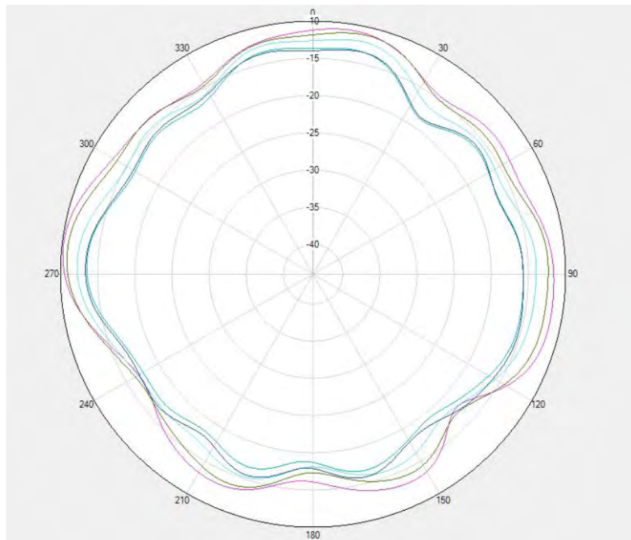
Flip- LTE B12/17&N12 \Phi=90\text{deg}
