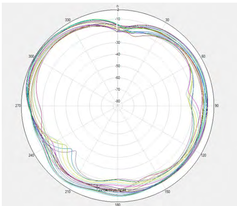
ENDC Flip LTEB1/B7/B38/40/41 PRX \Theta=90\text{deg}
