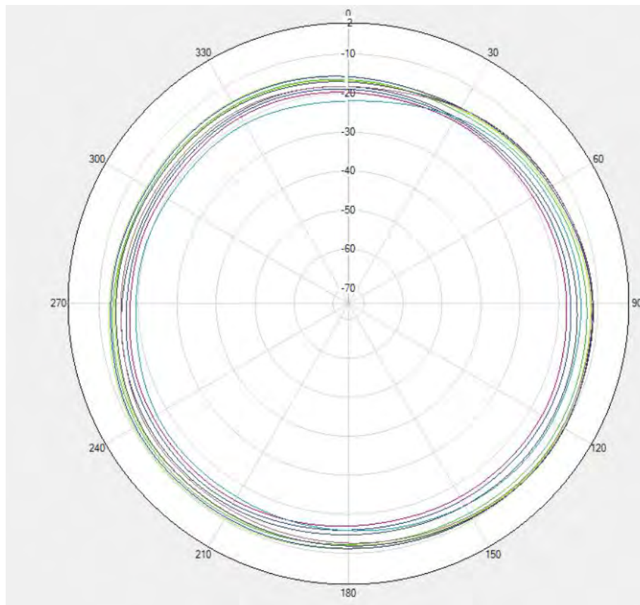
ENDC Flip LTE B28&NR N28 PRX Theta=90deg
