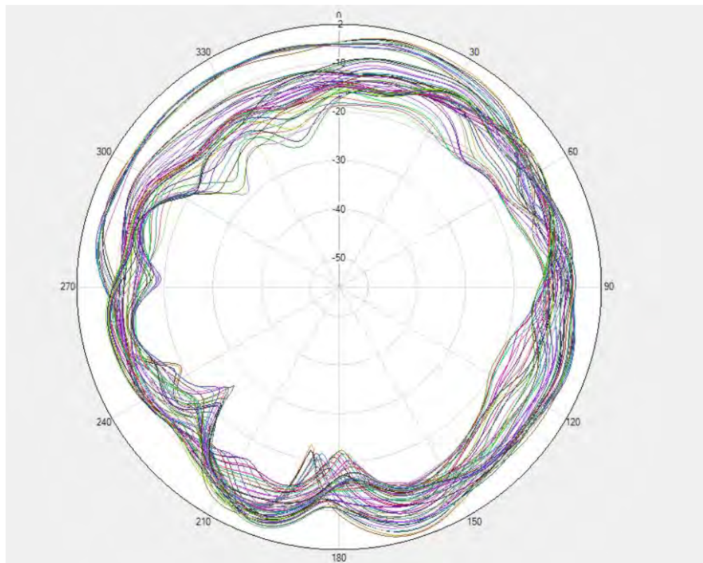
Unflip- N77/N78 PRX \Phi=90\text{deg}
