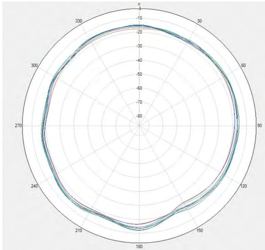
ENDC Unflip LTEB8&NR N8 PRX \Phi=90\text{deg}
