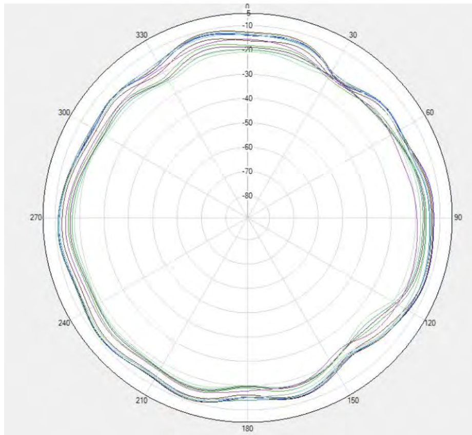
ENDC Flip LTE B28&NR N28 PRX \Phi=90\text{deg}
