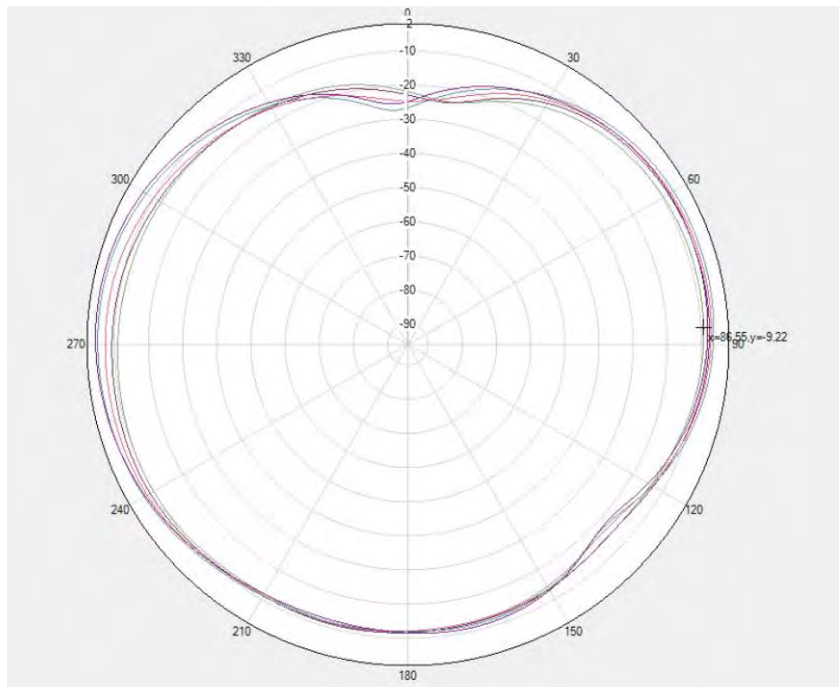
END C Flip LTE3/B4/B66 PRX \Theta = 90^\circ
