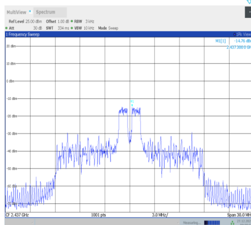
11ax20MIMO-Ant2-2437-26Tone-RU4-PASS
