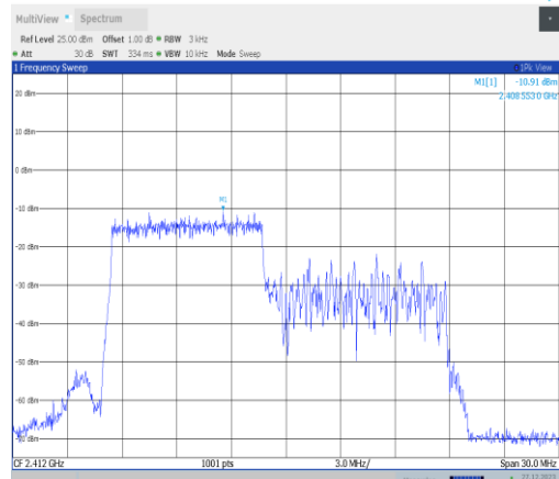
11ax20MIMO-Ant2-2412-106Tone-RU53-PASS
