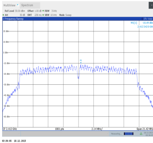
11g-Ant2-2412-PASS
