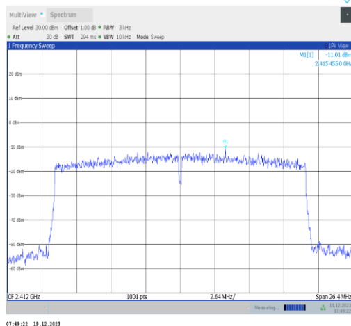
11ax20MIMO-Ant1-2412-PASS
