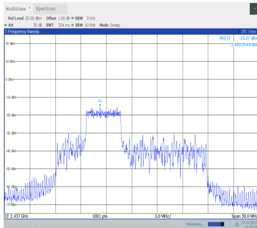
11ax20MIMO-Ant2-2437-52Tone-RU38-PASS
