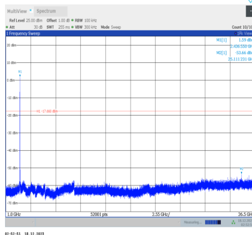
11b-Ant2-2437-1000~26500-PASS
