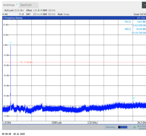
11g-Ant2-2412-1000~26500-PASS
