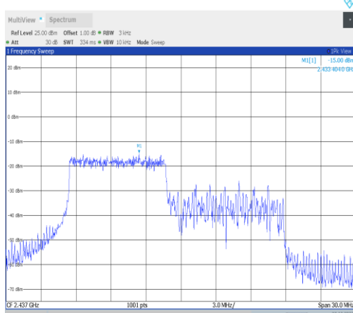
11ax20MIMO-Ant3-2437-106Tone-RU53-PASS
