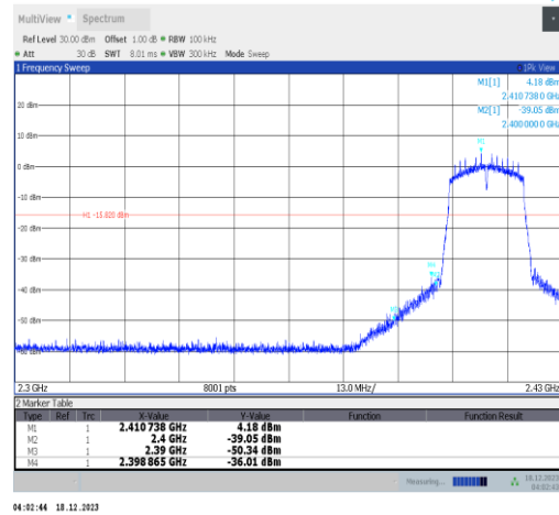
11n20SISO-Ant2-2412-PASS
