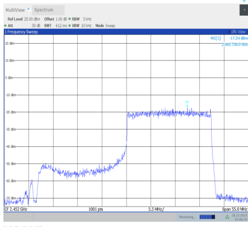
11ax40MIMO-Ant1-2452-242Tone-RU62-PASS
