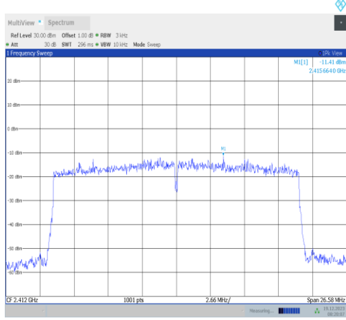
11ax20MIMO-Ant2-2412-PASS
