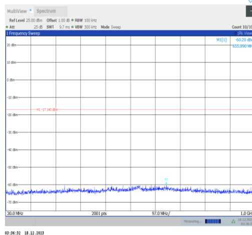
11g-Ant2-2412-30~1000-PASS
