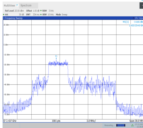
11ax20MIMO-Ant1-2437-52Tone-RU38-PASS
