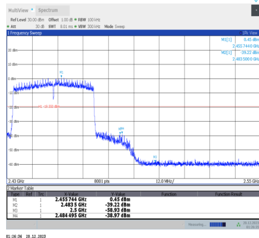
11ax40MIMO-Ant1-2452-PASS
