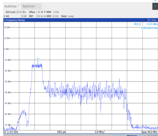
11ax20MIMO-Ant4-2412-26Tone-RU0-PASS
