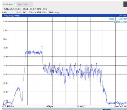
11ax20MIMO-Ant2-2412-52Tone-RU37-PASS
