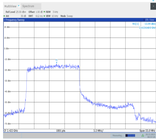
11ax40MIMO-Ant4-2422-242Tone-RU61-PASS
