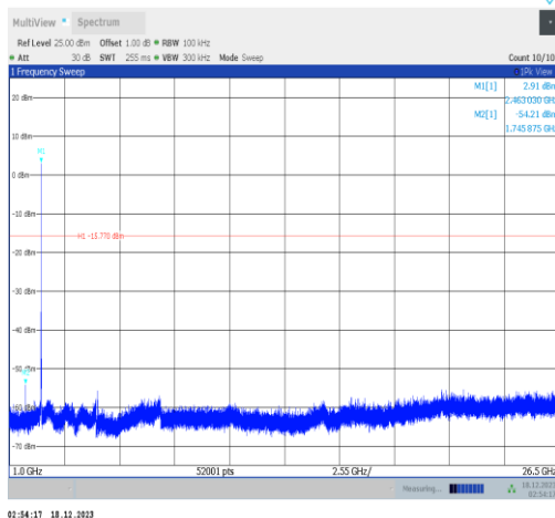
11b-Ant2-2462-1000~26500-PASS
