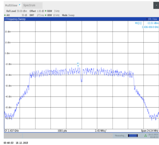
11g-Ant2-2437-PASS
