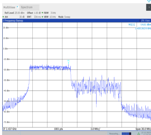
11ax20MIMO-Ant1-2437-106Tone-RU53-PASS
