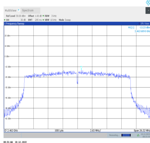
11ax20MIMO-Ant1-2462-PASS
