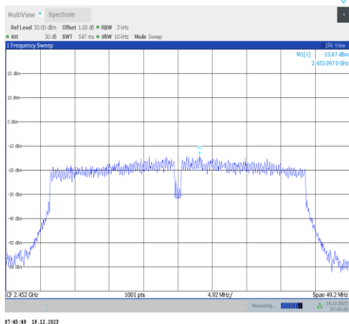
11n40SISO-Ant2-2452-PASS
