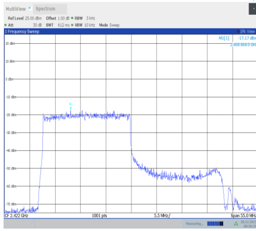
11ax40MIMO-Ant1-2422-242Tone-RU61-PASS
