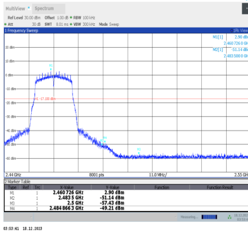
11g-Ant2-2462-PASS
