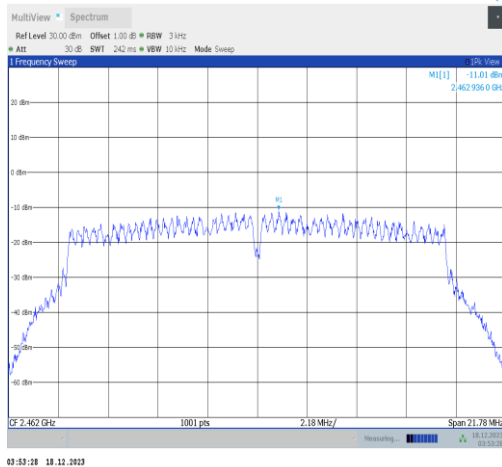
11g-Ant2-2462-PASS
