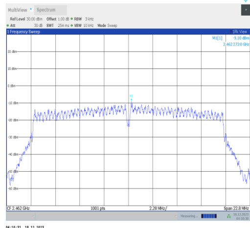
11n20SISO-Ant2-2462-PASS
