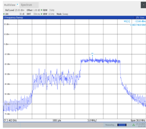
11ax20MIMO-Ant4-2462-106Tone-RU54-PASS
