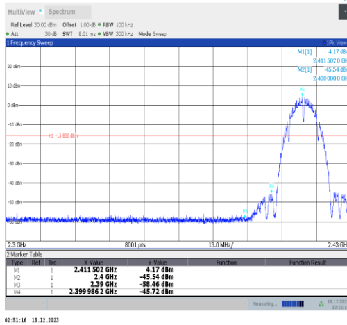
11b-Ant2-2412-PASS
