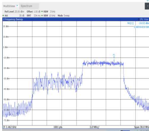
11ax20MIMO-Ant1-2462-106Tone-RU54-PASS
