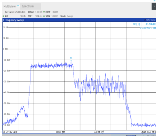
11ax20MIMO-Ant3-2412-106Tone-RU53-PASS
