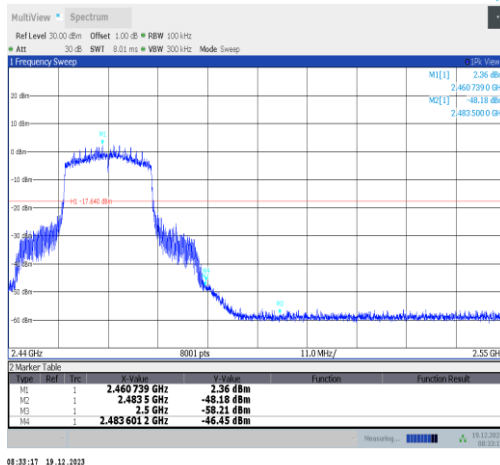
11ax20MIMO-Ant2-2462-PASS
