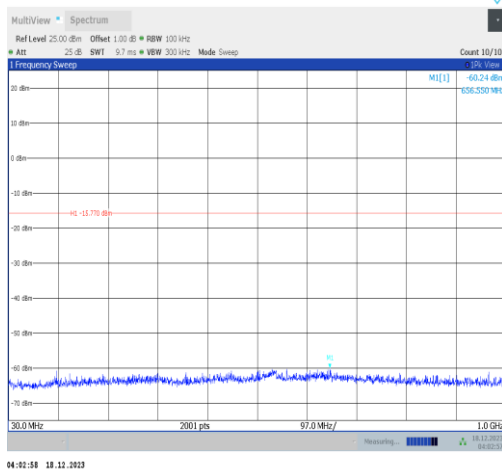
11n20SISO-Ant2-2412-30~1000-PASS
