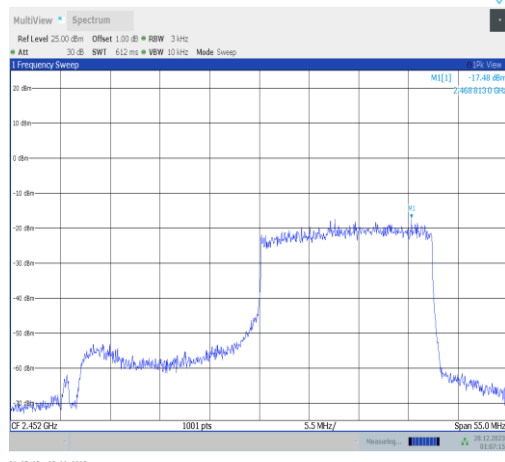
11ax40MIMO-Ant2-2452-242Tone-RU62-PASS
