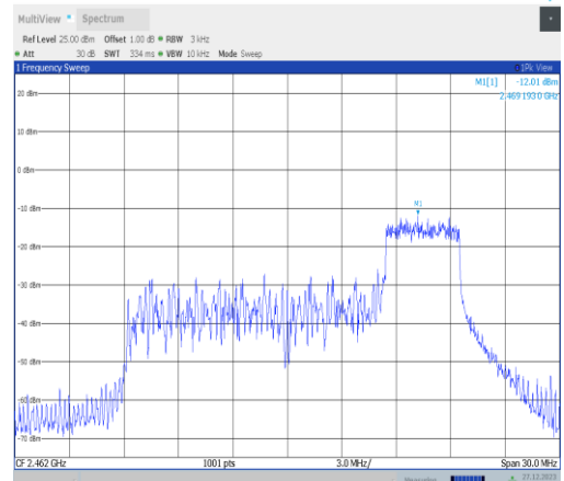
11ax20MIMO-Ant1-2462-52Tone-RU40-PASS
