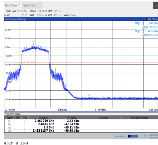
11ax20MIMO-Ant1-2462-PASS
