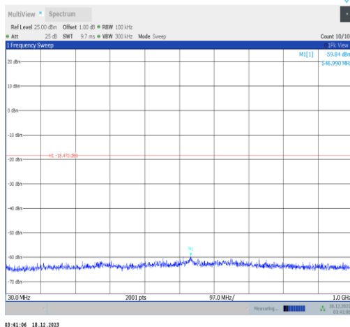
11g-Ant2-2437-30~1000-PASS
