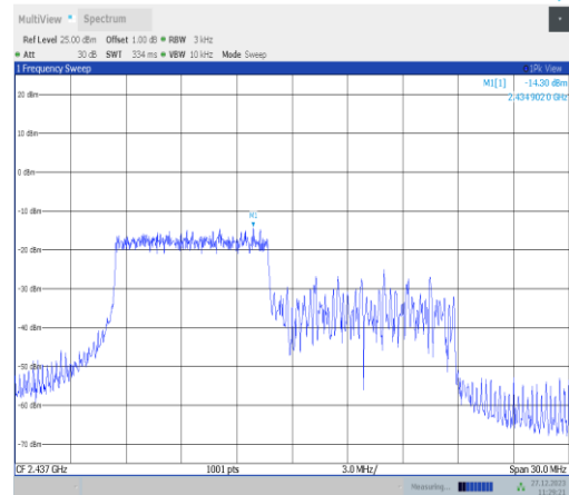
11ax20MIMO-Ant2-2437-106Tone-RU53-PASS
