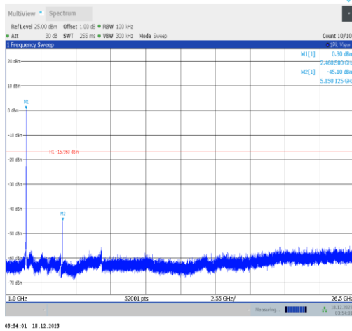
11g-Ant2-2462-1000~26500-PASS
