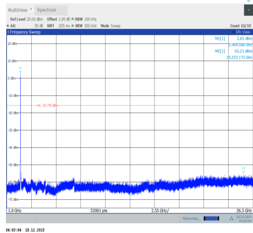
11n20SISO-Ant2-2412-1000~26500-PASS
