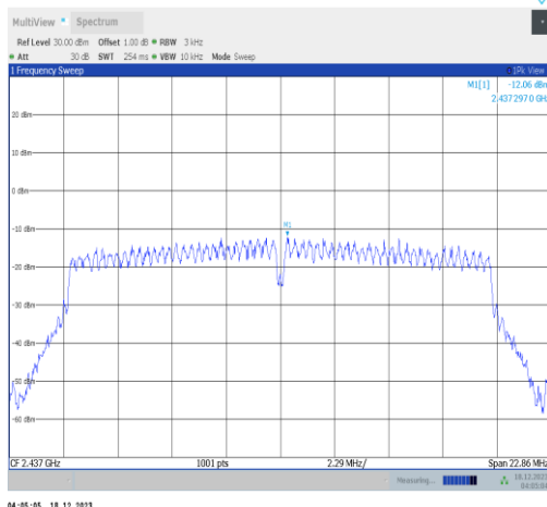
11n20SISO-Ant2-2437-PASS
