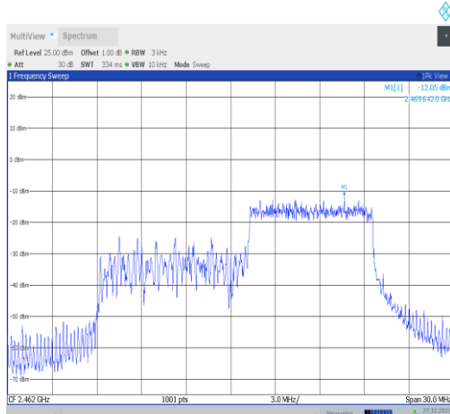
11ax20MIMO-Ant3-2462-26Tone-RU8-PASS
