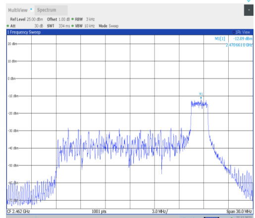
11ax20MIMO-Ant2-2462-26Tone-RU8-PASS
