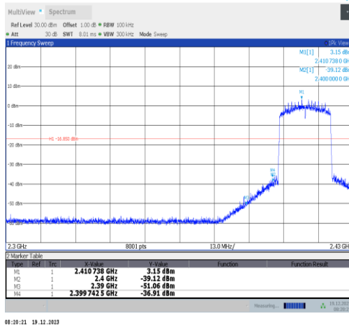
11ax20MIMO-Ant2-2412-PASS
