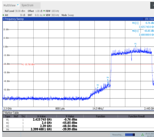
11ax40MIMO-Ant2-2422-PASS
