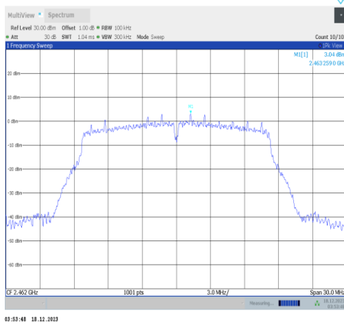
11g-Ant2-2462-0~Reference-PASS
