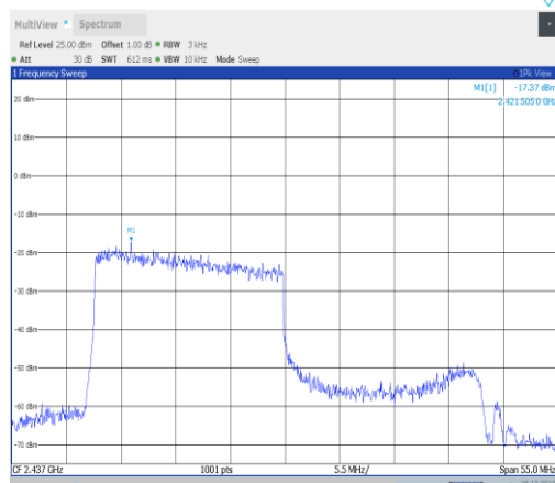
11ax40MIMO-Ant2-2437-242Tone-RU61-PASS
