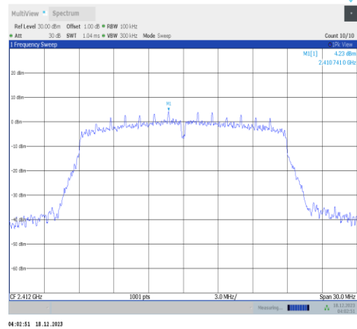
11n20SISO-Ant2-2412-0~Reference-PASS
