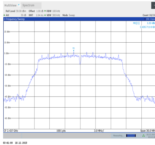
11g-Ant2-2437-0~Reference-PASS
