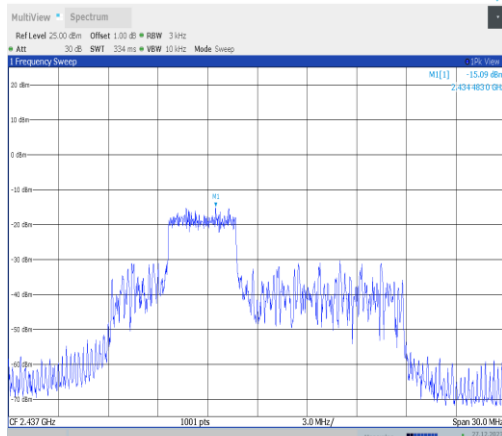
11ax20MIMO-Ant4-2437-52Tone-RU38-PASS
