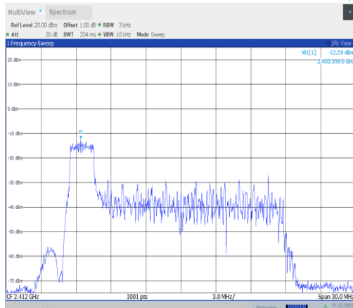
11ax20MIMO-Ant3-2412-26Tone-RU0-PASS
