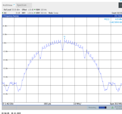
11b-Ant2-2462-0~Reference-PASS
