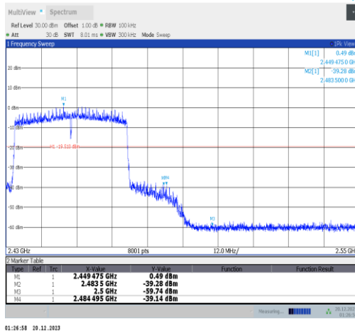
11ax40MIMO-Ant2-2452-PASS
