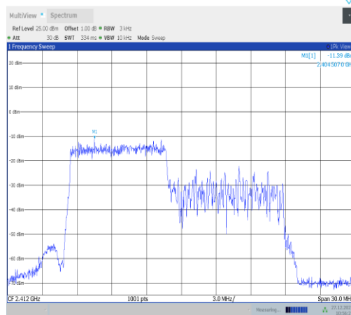
11ax20MIMO-Ant4-2412-106Tone-RU53-PASS
