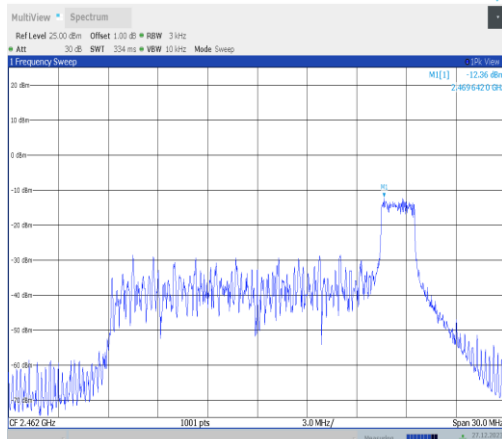
11ax20MIMO-Ant3-2462-26Tone-RU8-PASS
