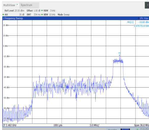
11ax20MIMO-Ant1-2462-26Tone-RU8-PASS
