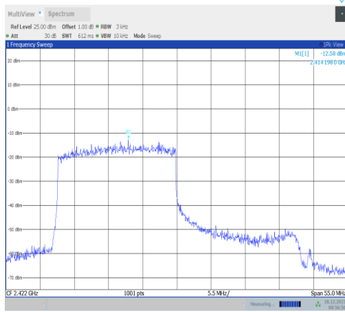
11ax40MIMO-Ant3-2422-242Tone-RU61-PASS
