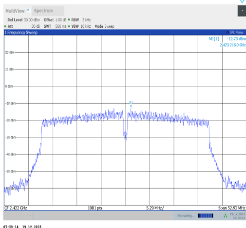
11n40SISO-Ant2-2422-PASS
