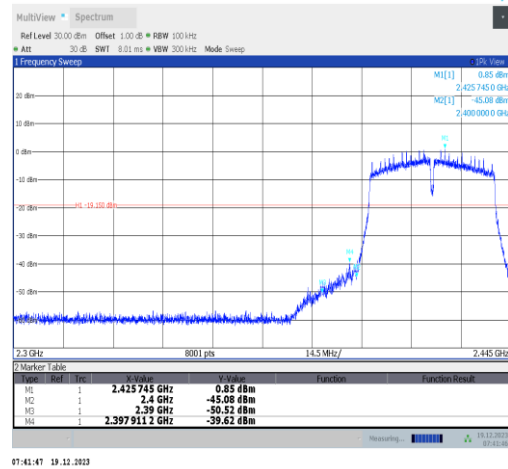
11n40SISO-Ant2-2422-PASS
