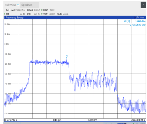
11ax20MIMO-Ant4-2437-106Tone-RU53-PASS
