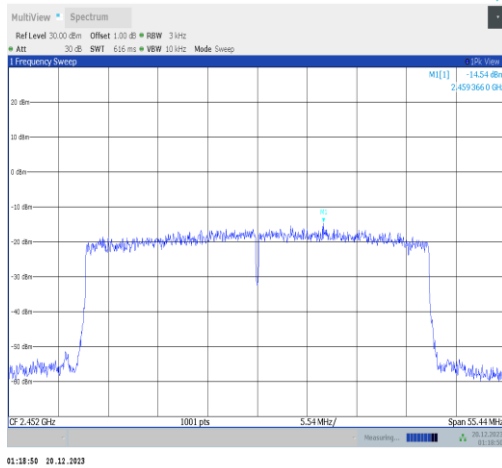
11ax40MIMO-Ant2-2452-PASS
