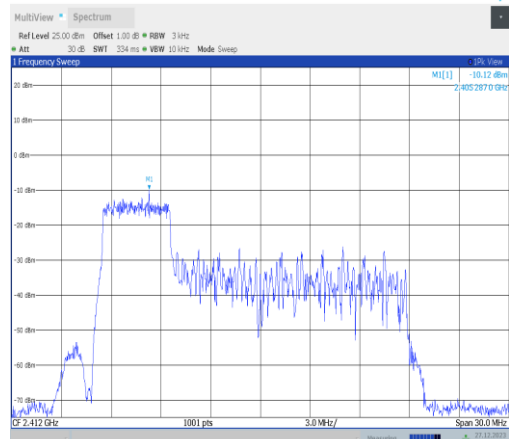
11ax20MIMO-Ant3-2412-52Tone-RU37-PASS
