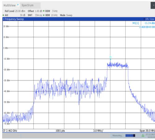
11ax20MIMO-Ant4-2462-52Tone-RU40-PASS
