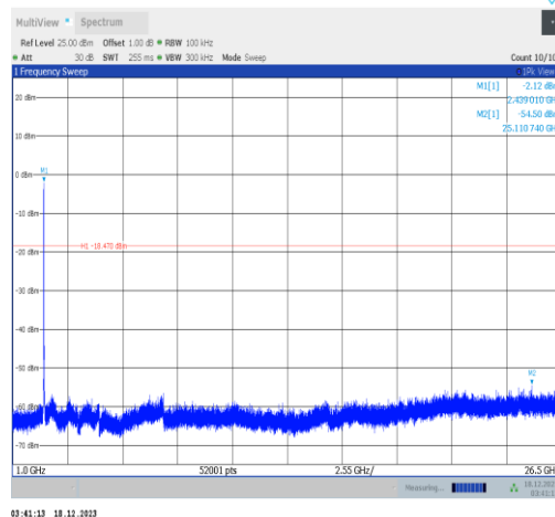
11g-Ant2-2437-1000~26500-PASS
