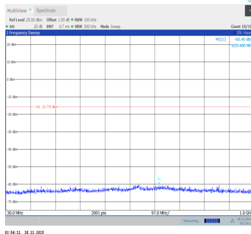
11b-Ant2-2462-30~1000-PASS
