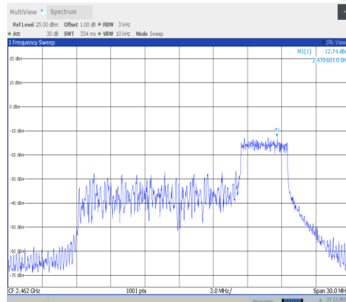
11ax20MIMO-Ant3-2462-52Tone-RU40-PASS
