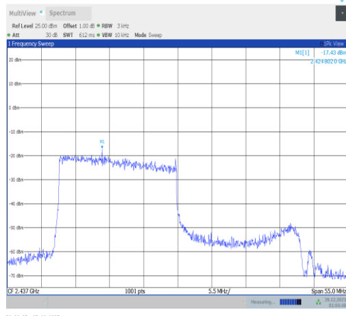
11ax40MIMO-Ant4-2437-242Tone-RU61-PASS
