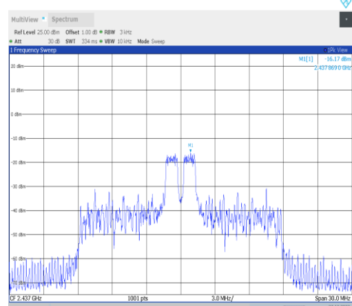
11ax20MIMO-Ant4-2437-26Tone-RU4-PASS
