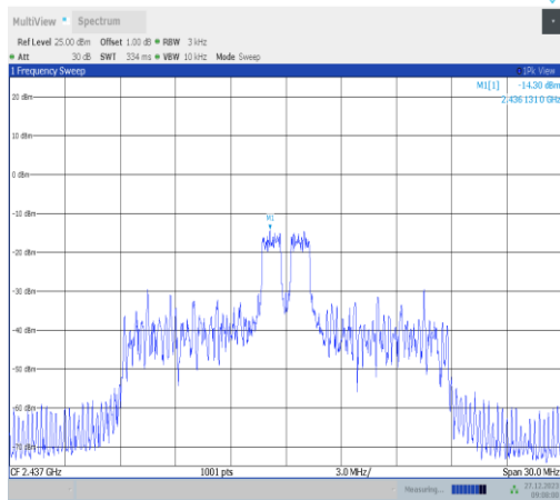
11ax20MIMO-Ant1-2437-26Tone-RU4-PASS
