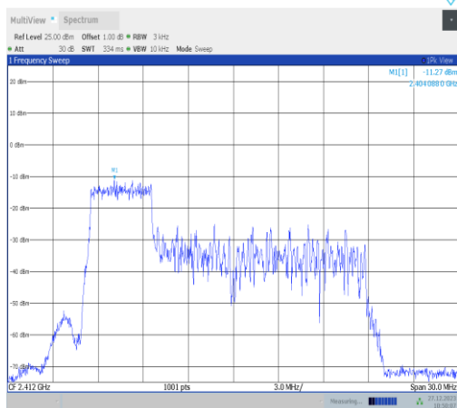
11ax20MIMO-Ant4-2412-52Tone-RU37-PASS
