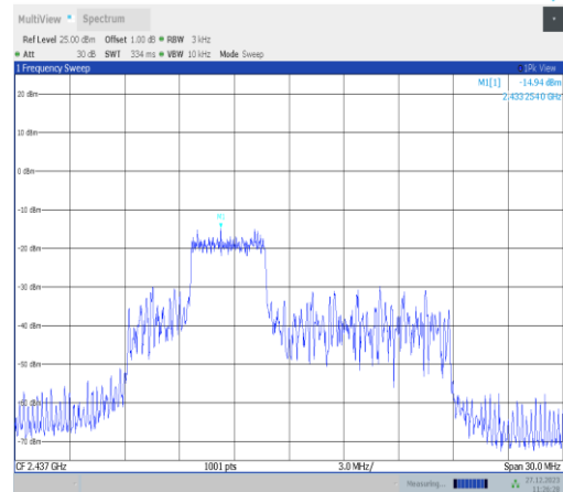
11ax20MIMO-Ant3-2437-52Tone-RU38-PASS
