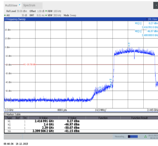
11ax40MIMO-Ant1-2422-PASS
