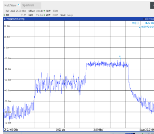
11ax20MIMO-Ant2-2462-106Tone-RU54-PASS
