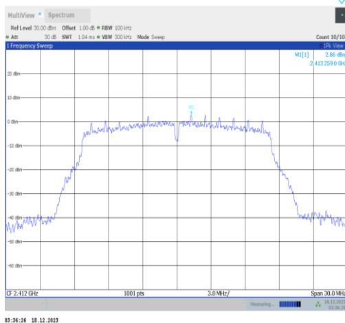
11g-Ant2-2412-0~Reference-PASS
