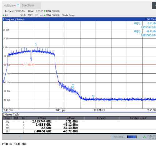
11n40SISO-Ant2-2452-PASS
