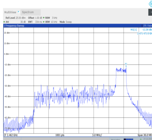
11ax20MIMO-Ant3-2462-52Tone-RU40-PASS
