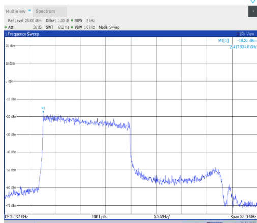
11ax40MIMO-Ant1-2437-242Tone-RU61-PASS
