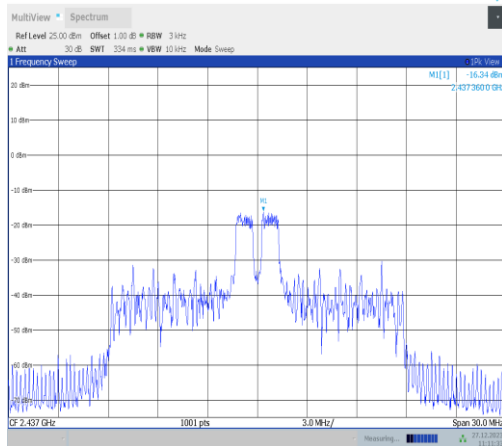
11ax20MIMO-Ant3-2437-26Tone-RU4-PASS
