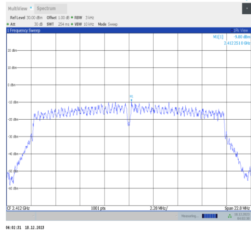
11n20SISO-Ant2-2412-PASS
