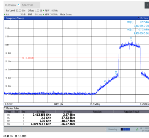
11ax20MIMO-Ant1-2412-PASS
