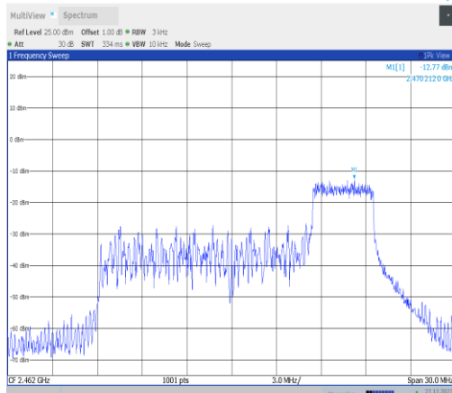
11ax20MIMO-Ant2-2462-52Tone-RU40-PASS
