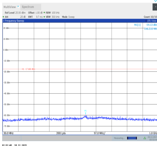
11b-Ant2-2437-30~1000-PASS
