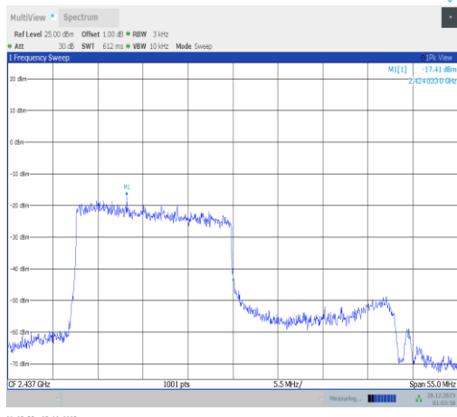
11ax40MIMO-Ant3-2437-242Tone-RU61-PASS
