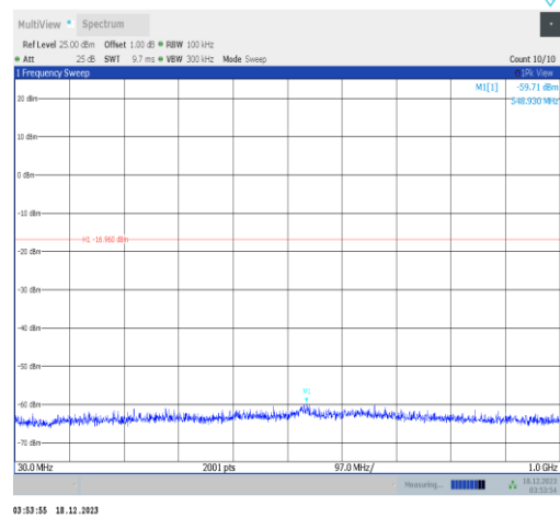
11g-Ant2-2462-30~1000-PASS
