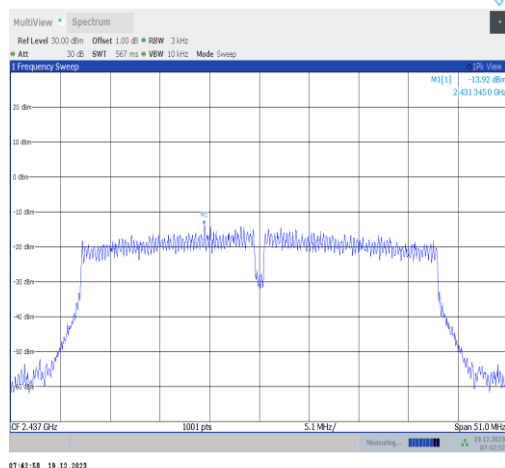
11n40SISO-Ant2-2437-PASS
