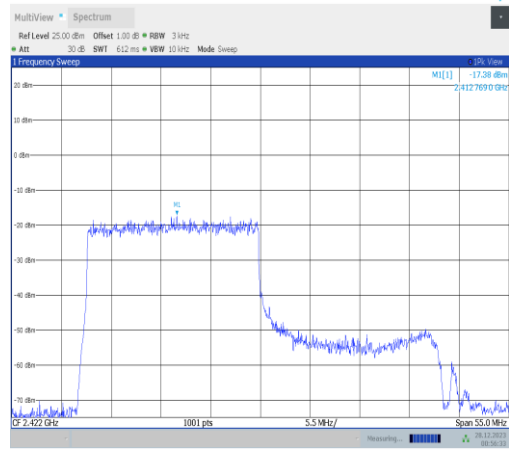
11ax40MIMO-Ant2-2422-242Tone-RU61-PASS
