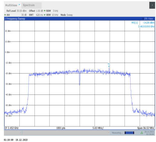
11ax40MIMO-Ant3-2452-PASS
