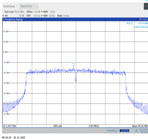
11ax20MIMO-Ant2-2437-PASS
