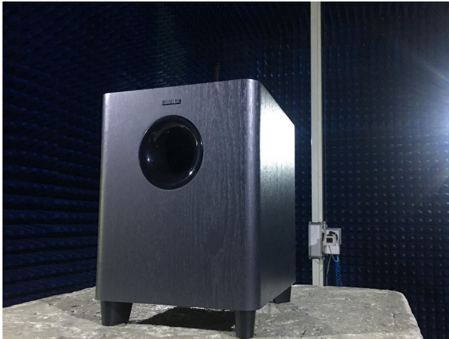
Photograph 5: Set-up for Radiated Spurious Emission, 18GHz - 40GHz
