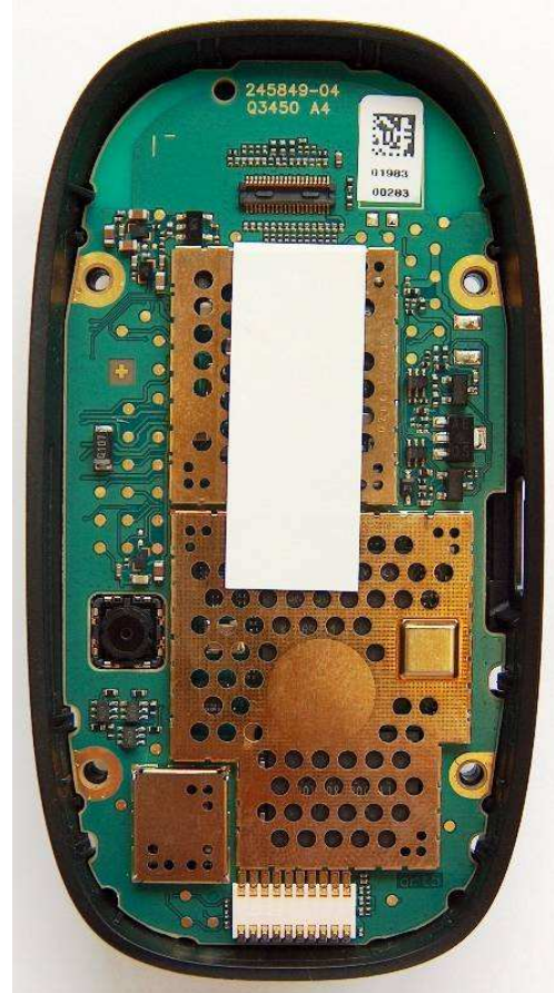
Disassemble Step 7: Rear Cover Base with PCB
