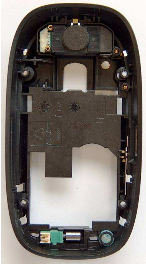
Disassemble Step 6: Rear Cover Base
