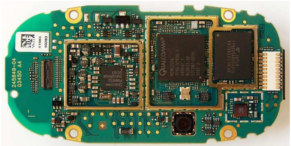
Disassemble Step 8: Back Side of main PCB
