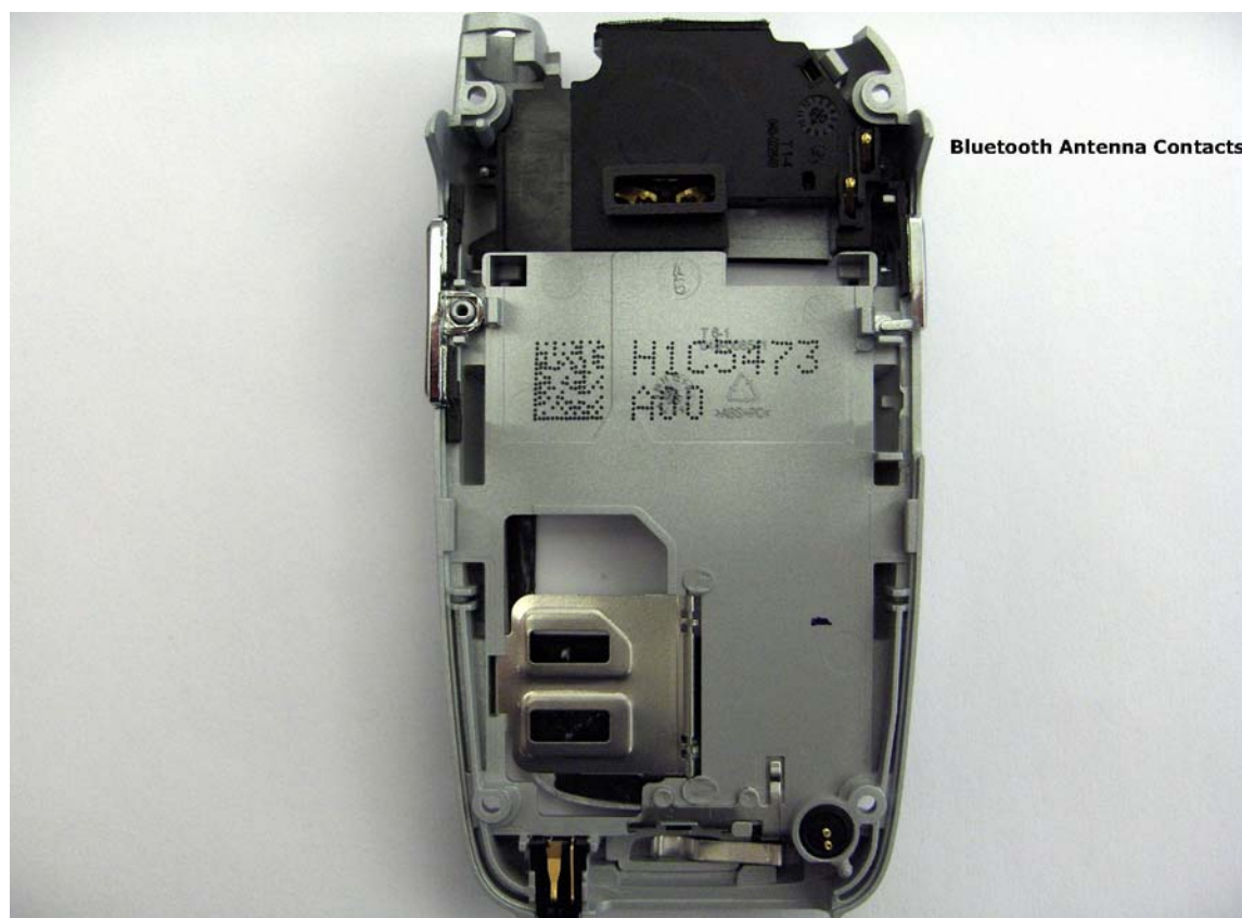
Cover showing the contact points for Bluetooth antenna
