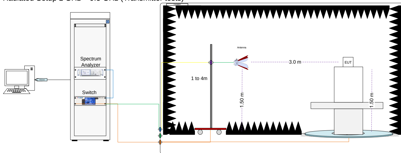
Radiated Setup 1 GHz – 9.5 GHz (Transmitter tests)
