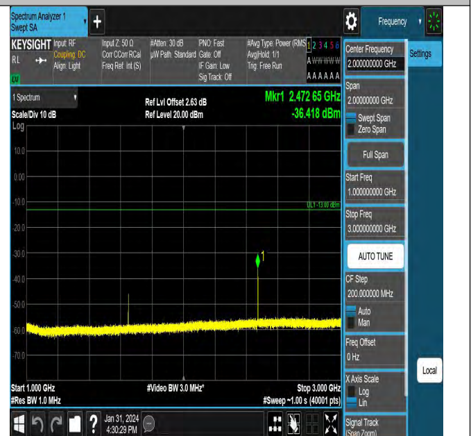
Band5_1.4MHz_QPSK_20407_1RB#0_1000~3000_1000~3000
