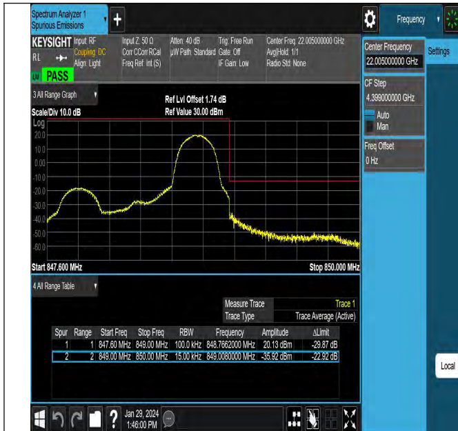
Band5_1.4MHz_QPSK_20643_1RB#5
