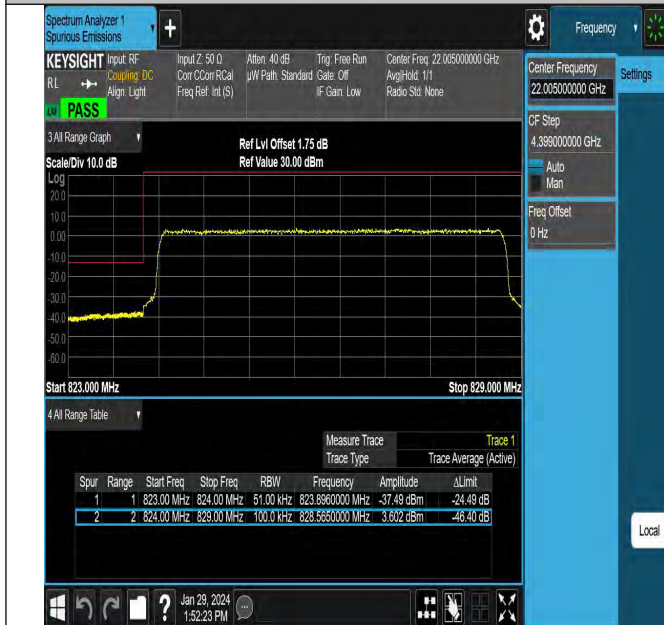
Band5_5MHz_QPSK_20425_25RB#0
