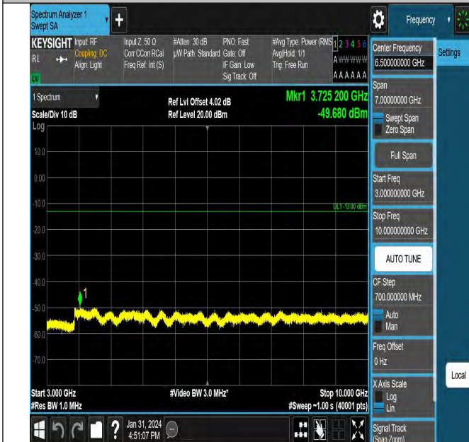
Band5_5MHz_QPSK_20425_1RB#0_3000~10000_3000~100
