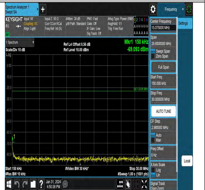
Band5_5MHz_QPSK_20425_1RB#0_0.15~30_0.15~30
